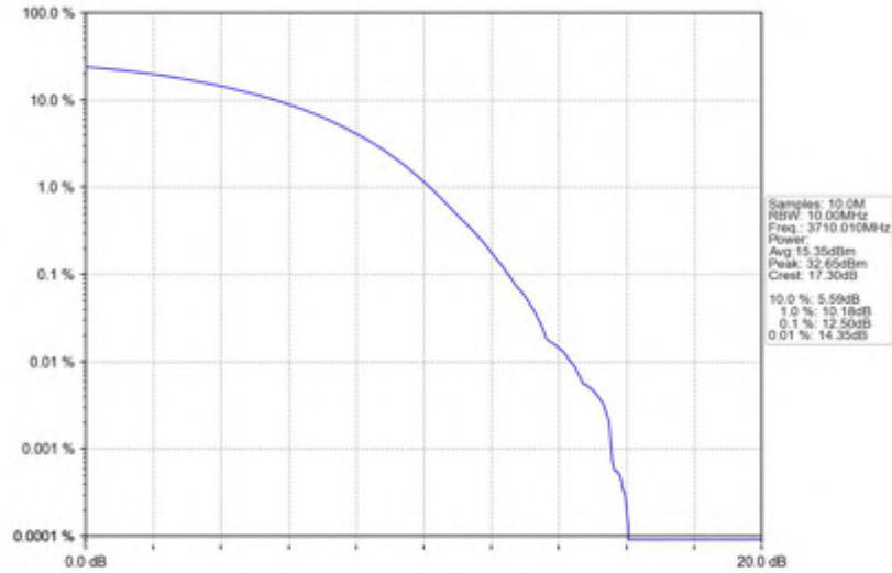
n78(3700-3800MHz)_30kHz_SISO_NTNV_20MHz_CP-OFDM 256 QAM_3710.01MHz_Outer_Full
