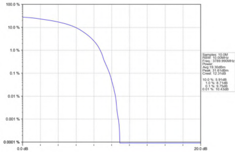
n78(3700-3800MHz)_30kHz_SISO_NTNV_20MHz_DFT-s-OFDM_QPSK_3789.99MHz_Outer_Full
