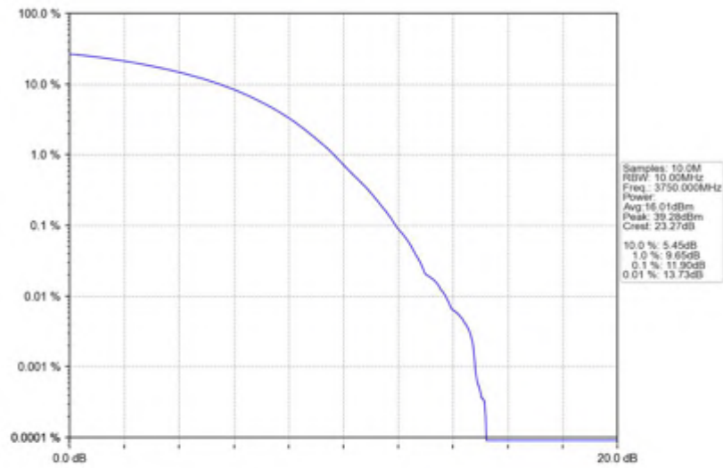
n78(3700-3800MHz)_30kHz_SISO_NTNV_20MHz_CP-OFDM 256 QAM_3750MHz_Outer_Full
