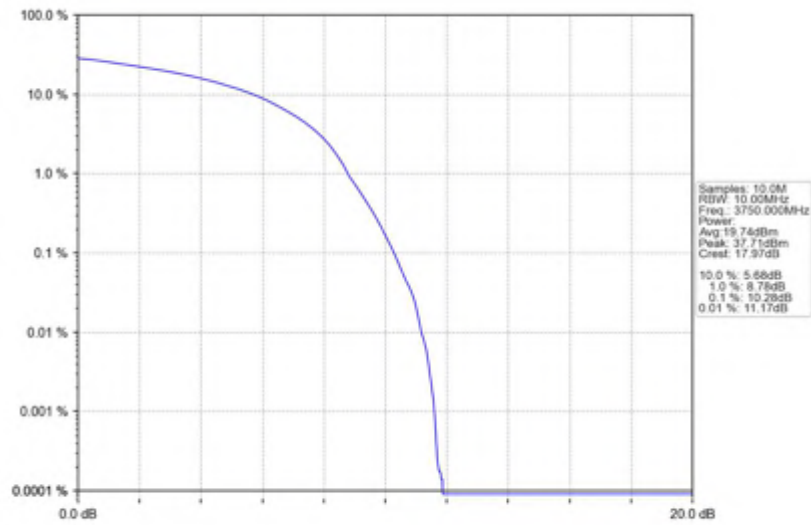
n78(3700-3800MHz)_30kHz_SISO_NTNV_20MHz_DFT-s-OFDM_16_QAM_3750MHz_Outer_Full
