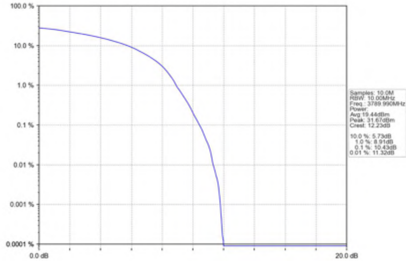
n78(3700-3800MHz)_30kHz_SISO_NTNV_20MHz_DFT-s-OFDM_16_QAM_3789.99MHz_Outer_Full
