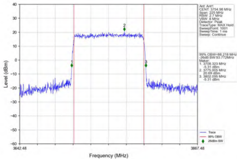
n78(3700-3800MHz)_30kHz_SISO_NTNV_90MHz_CP-OFDM 64 QAM_3754.98MHz_Outer_Full
