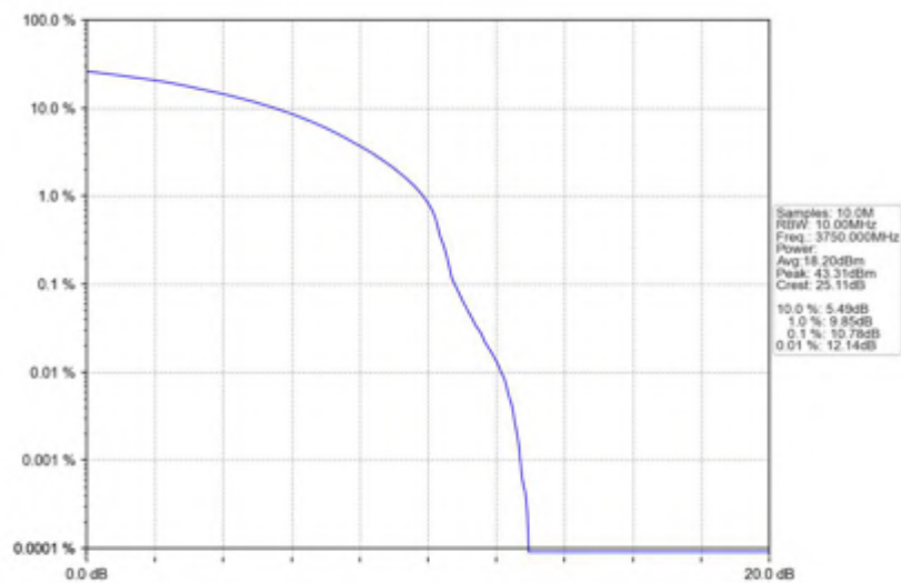
n78(3700-3800MHz)_30kHz_SISO_NTNV_30MHz_DFT-s-OFDM_16_QAM_3750MHz_Outer_Full
