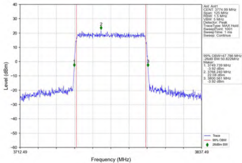
n78(3700-3800MHz)_30kHz_SISO_NTNV_50MHz_CP-OFDM QPSK_3774.99MHz_Outer_Full
