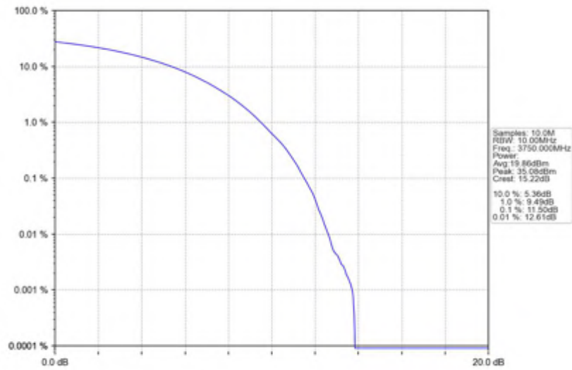
n78(3700-3800MHz)_30kHz_SISO_NTNV_20MHz_CP-OFDM_16_QAM_3750MHz_Outer_Full
