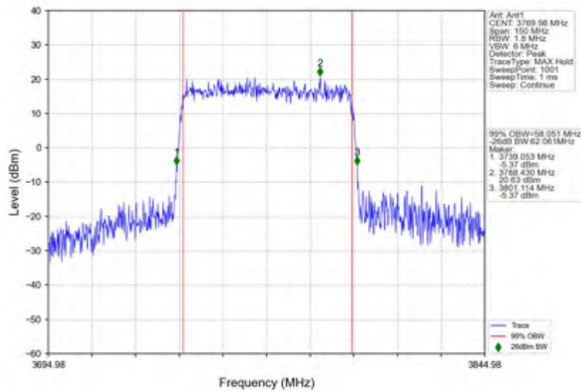
n78(3700-3800MHz)_30kHz_SISO_NTNV_60MHz_CP-OFDM QPSK_3769.98MHz_Outer_Full
