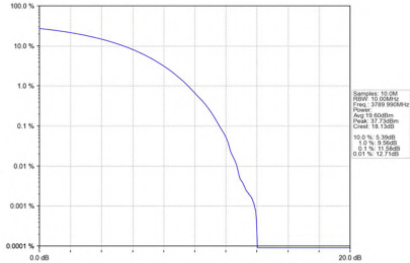
n78(3700-3800MHz)_30kHz_SISO_NTNV_20MHz_CP-OFDM 16 QAM_3789.99MHz_Outer_Full
