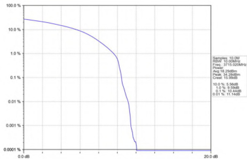
n78(3700-3800MHz)_30kHz_SISO_NTNV_30MHz_DFT-s-OFDM QPSK_3715.02MHz_Outer_Full
