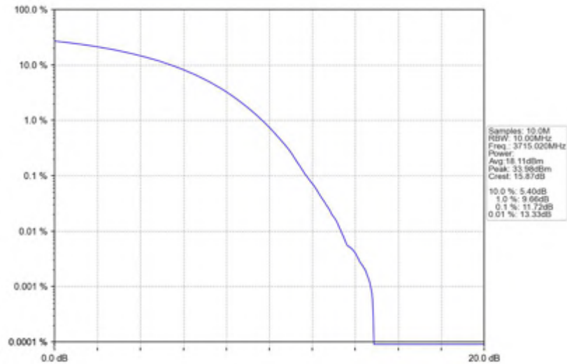
n78(3700-3800MHz)_30kHz_SISO_NTNV_30MHz_CP-OFDM_16_QAM_3715.02MHz_Outer_Full
