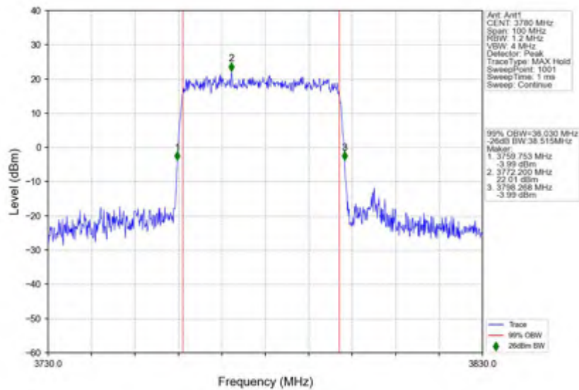
n78(3700-3800MHz)_30kHz_SISO_NTNV_40MHz_DFT-s-OFDM 64 QAM 3780MHz_Outer_Full
