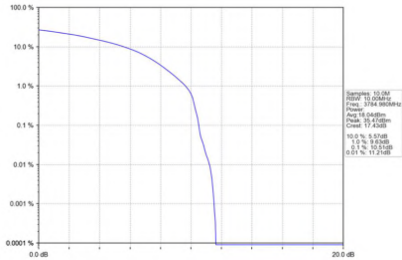
n78(3700-3800MHz)_30kHz_SISO_NTNV_30MHz_DFT-s-OFDM_QPSK_3784.98MHz_Outer_Full
