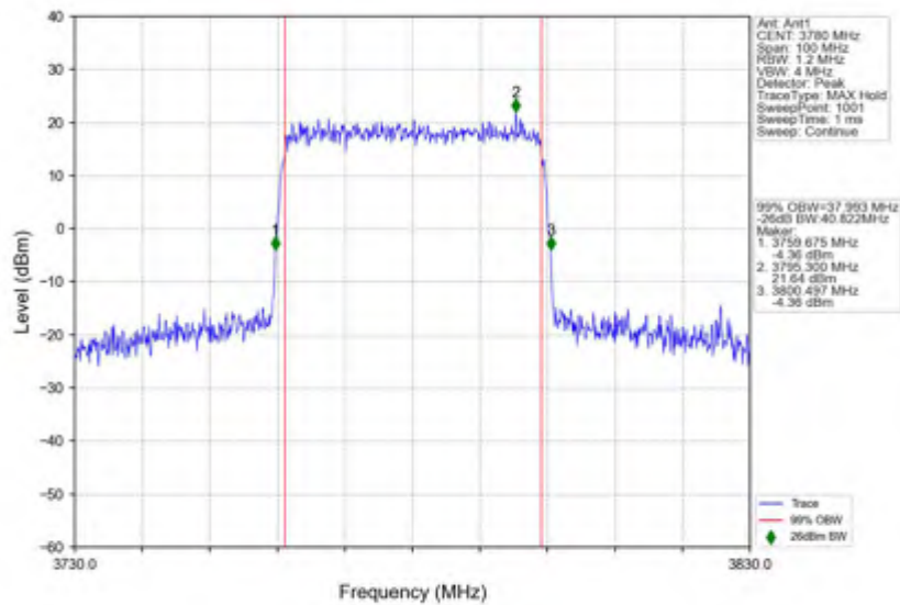
n78(3700-3800MHz)_30kHz_SISO_NTNV_40MHz_CP-OFDM QPSK_3780MHz_Outer_Full
