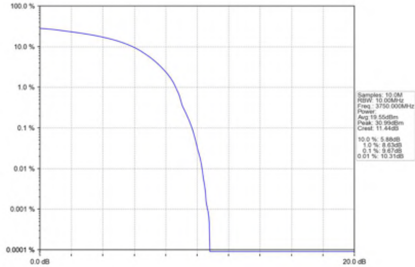
n78(3700-3800MHz)_30kHz_SISO_NTNV_20MHz_DFT-s-OFDM_QPSK_3750MHz_Outer_Full
