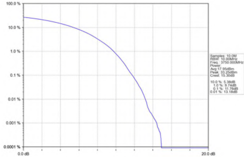
n78(3700-3800MHz)_30kHz_SISO_NTNV_30MHz_CP-OFDM QPSK_3750MHz_Outer_Full
