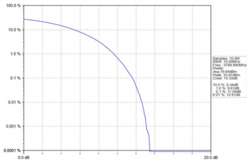
n78(3700-3800MHz)_30kHz_SISO_NTNV_20MHz_CP-OFDM QPSK_3789.99MHz_Outer_Full
