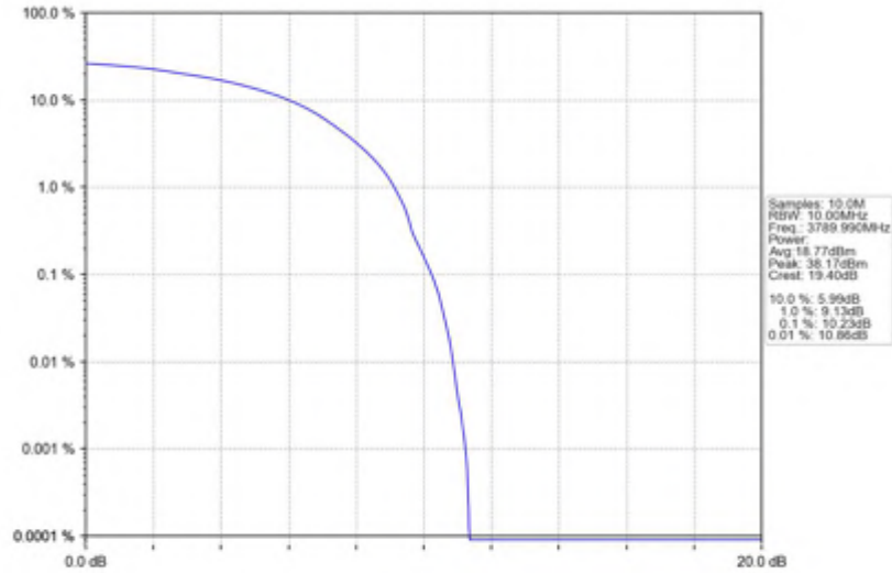
n78(3700-3800MHz)_30kHz_SISO_NTNV_20MHz_DFT-s-OFDM PI/2 BPSK_3789.99MHz_Outer_Full
