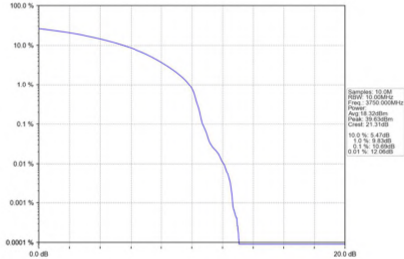
n78(3700-3800MHz)_30kHz_SISO_NTNV_30MHz_DFT-s-OFDM_64_QAM_3750MHz_Outer_Full
