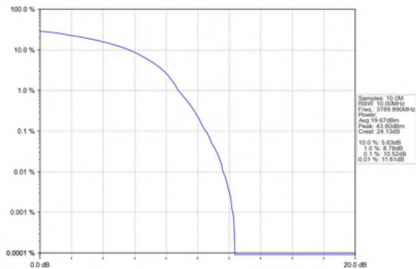
n78(3700-3800MHz)_30kHz_SISO_NTNV_20MHz_DFT-s-OFDM_64_QAM_3789.99MHz_Outer_Full
