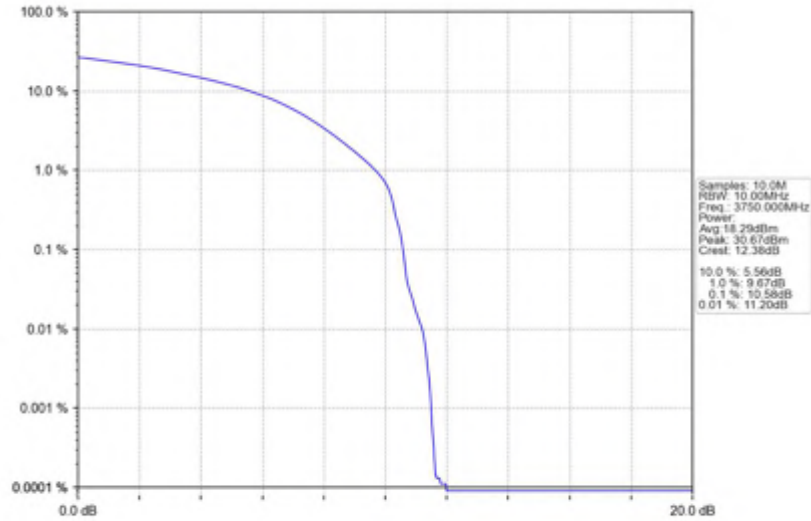
n78(3700-3800MHz)_30kHz_SISO_NTNV_30MHz_DFT-s-OFDM_QPSK_3750MHz_Outer_Full
