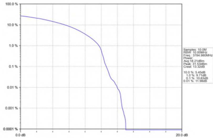
n78(3700-3800MHz)_30kHz_SISO_NTNV_30MHz_DFT-s-OFDM_64_QAM_3784.98MHz_Outer_Full
