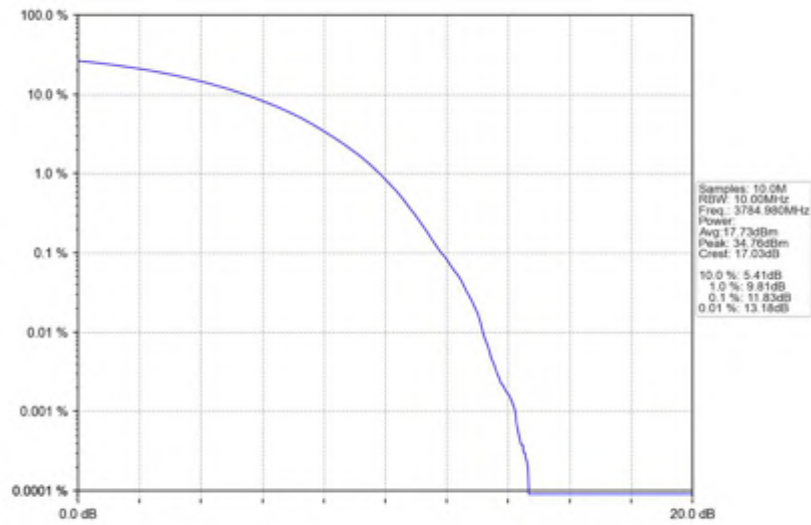
n78(3700-3800MHz)_30kHz_SISO_NTNV_30MHz_CP-OFDM QPSK_3784.98MHz_Outer_Full
