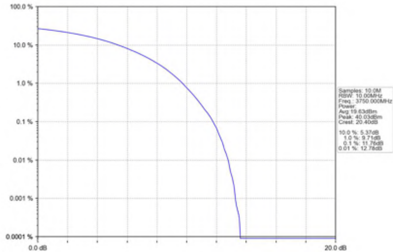
n78(3700-3800MHz)_30kHz_SISO_NTNV_20MHz_CP-OFDM QPSK_3750MHz_Outer_Full
