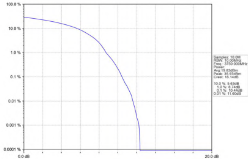
n78(3700-3800MHz)_30kHz_SISO_NTNV_20MHz_DFT-s-OFDM_64_QAM_3750MHz_Outer_Full
