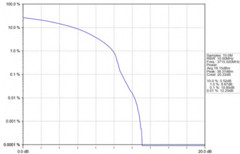
n78(3700-3800MHz)_30kHz_SISO_NTNV_30MHz_DFT-s-OFDM_16_QAM_3715.02MHz_Outer_Full
