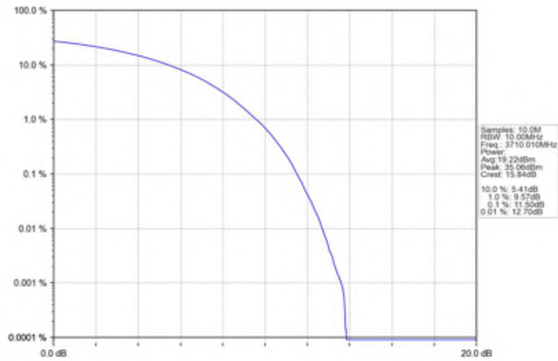
n78(3700-3800MHz)_30kHz_SISO_NTNV_20MHz_CP-OFDM 64 QAM_3710.01MHz_Outer_Full
