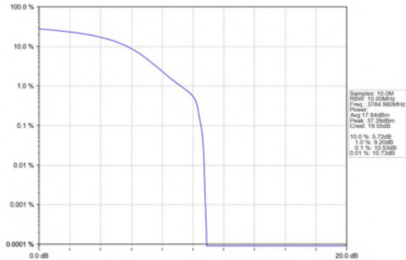
n78(3700-3800MHz)_30kHz_SISO_NTNV_30MHz_DFT-s-OFDM PI/2 BPSK_3784.98MHz_Outer_Full
