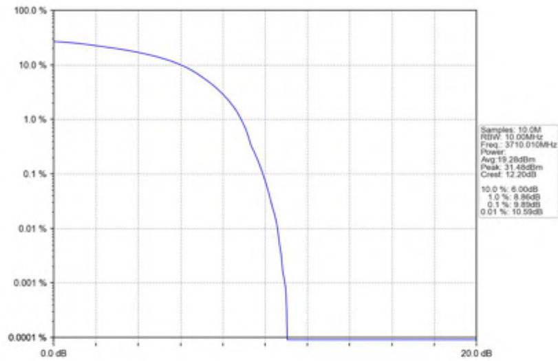
n78(3700-3800MHz)_30kHz_SISO_NTNV_20MHz_DFT-s-OFDM QPSK_3710.01MHz_Outer_Full
