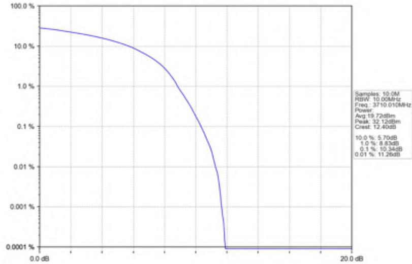
n78(3700-3800MHz)_30kHz_SISO_NTNV_20MHz_DFT-s-OFDM_16_QAM_3710.01MHz_Outer_Full
