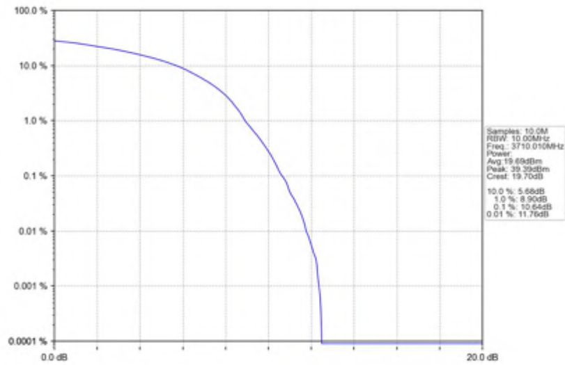
n78(3700-3800MHz)_30kHz_SISO_NTNV_20MHz_DFT-s-OFDM_64_QAM_3710.01MHz_Outer_Full
