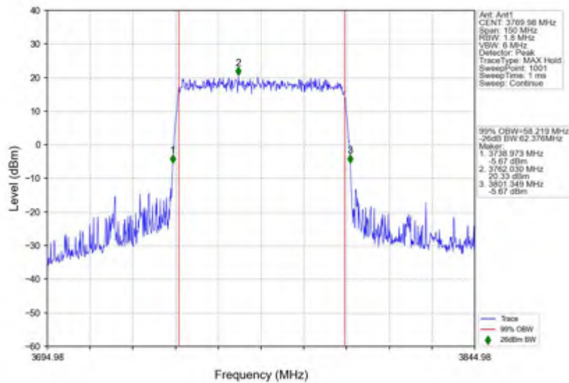
n78(3700-3800MHz)_30kHz_SISO_NTNV_60MHz_DFT-s-OFDM_QPSK_3769.98MHz_Outer_Full
