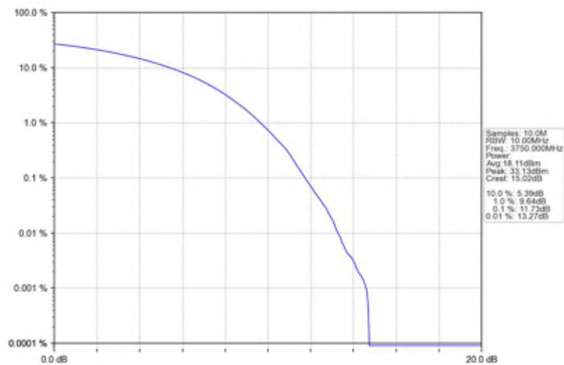
n78(3700-3800MHz)_30kHz_SISO_NTNV_30MHz_CP-OFDM_16_QAM_3750MHz_Outer_Full
