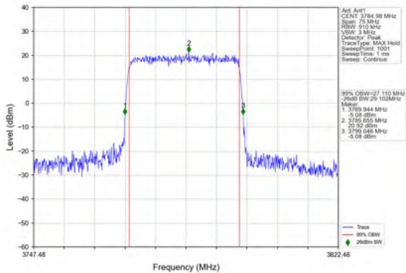
n78(3700-3800MHz)_30kHz_SISO_NTNV_30MHz_DFT-s-OFDM_QPSK_3784.98MHz_Outer_Full
