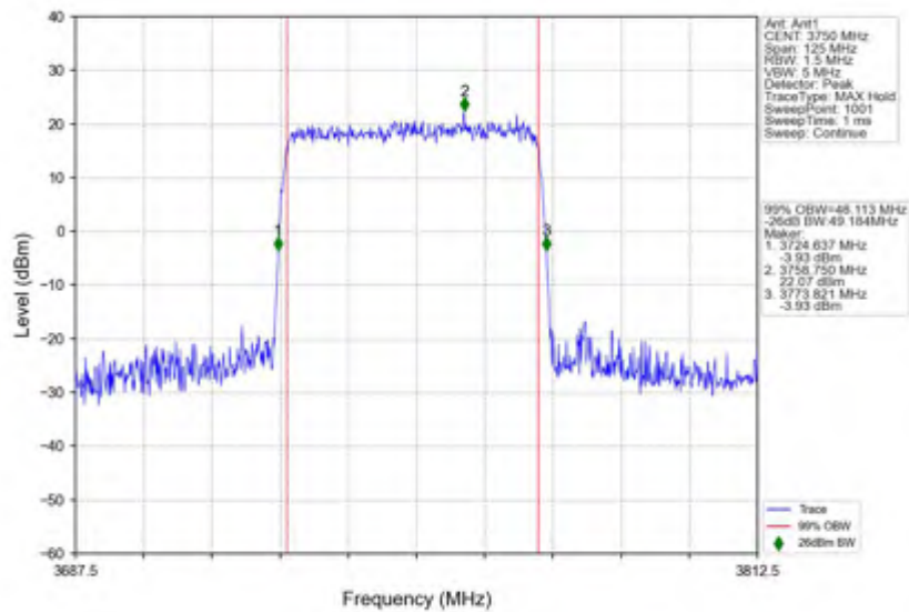
n78(3700-3800MHz)_30kHz_SISO_NTNV_50MHz_DFT-s-OFDM_16_QAM_3750MHz_Outer_Full
