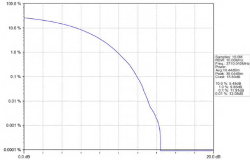
n78(3700-3800MHz)_30kHz_SISO_NTNV_20MHz_CP-OFDM_16_QAM_3710.01MHz_Outer_Full
