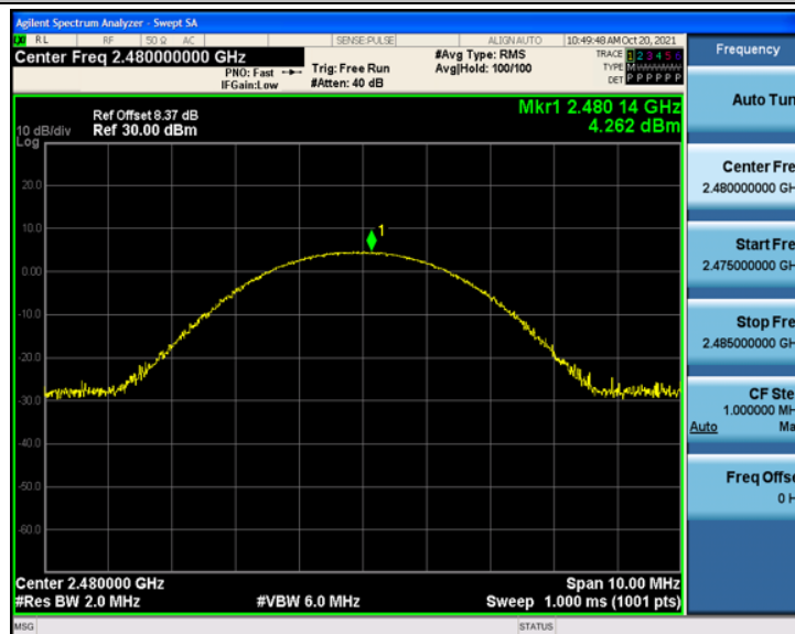
3DH5_Ant1_2480
