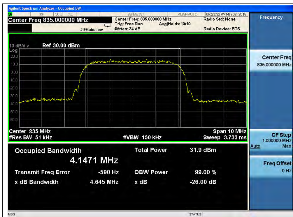
(Plot P2, HSPA+850 MHz, Channel = 4175)
