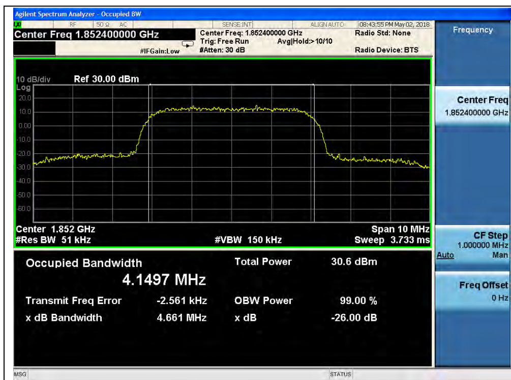
(Plot L1, HSDPA 1900MHz, Channel = 9262)
