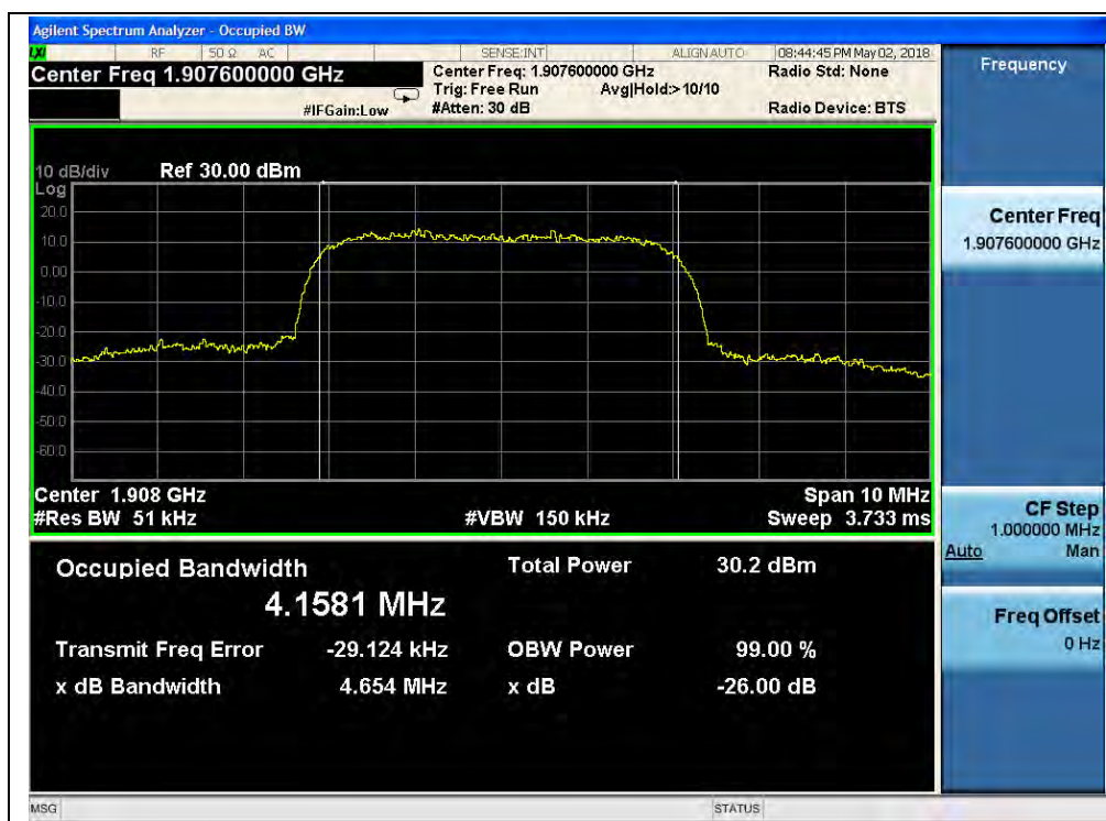
(Plot L3, HSDPA 1900MHz, Channel = 9538)
