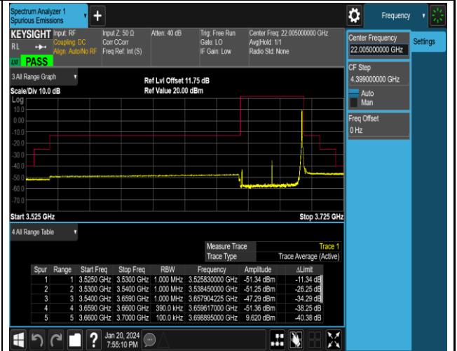
NTNV_N48_PC3_30_40_H_TID6_#1
