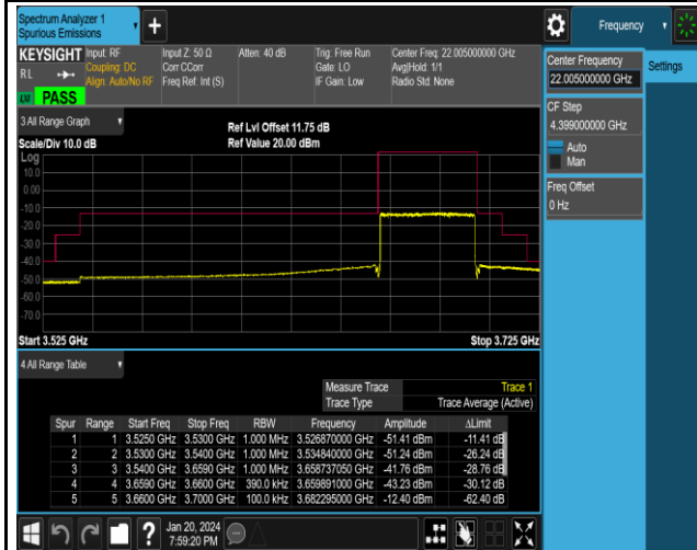
NTNV_N48_PC3_30_40_H_TID16_#1
