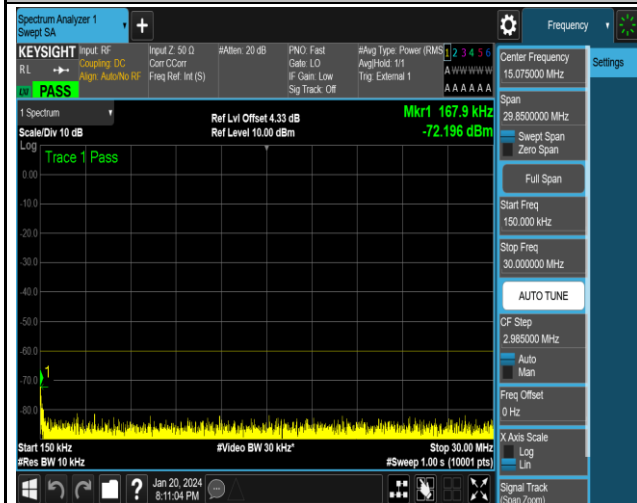
NTNV_N48_PC3_30_40_L_TID1_NS_01_0.15_30_#1
