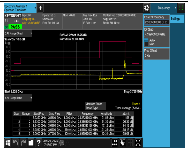
NTNV_N48_PC3_30_40_H_TID3_#1
