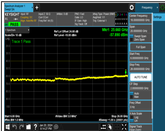
NTNV_N48_PC3_30_40_L_TID1_NS_01_6000_26000_#1
