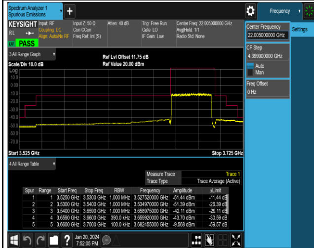
NTNV_N48_PC3_30_40_H_TID4_#1
