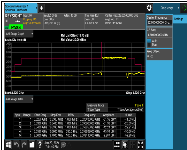
NTNV_N48_PC3_30_40_H_TID1_#1
