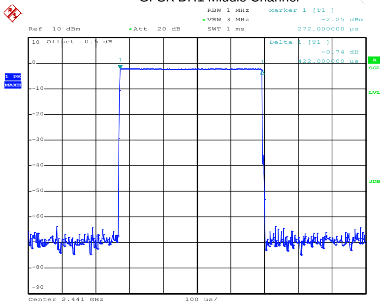
Test Plots GFSK DH1 Middle Channel
