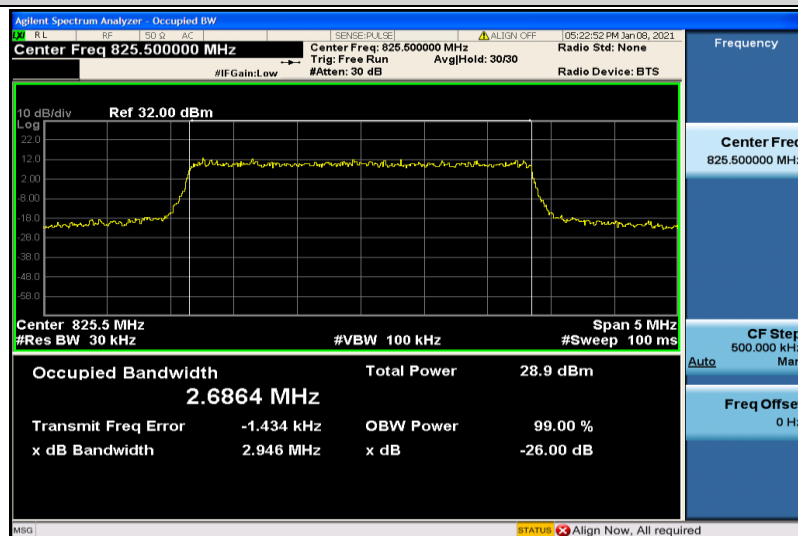
Band26-3MHz-QPSK-26805-15RB#0-2.6864
