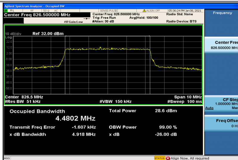
Band26-5MHz-16QAM-26815-25RB#0-4.4802
