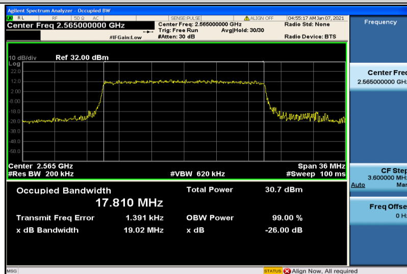
Band41-20MHz-16QAM-40340-100RB#0-17.810
