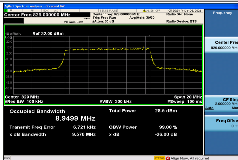
Band26-10MHz-16QAM-26840-50RB#0-8.9499
