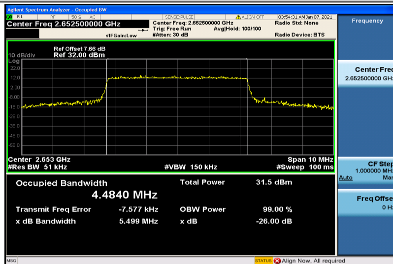
Band41-5MHz-QPSK-41215-25RB#0-4.4840
