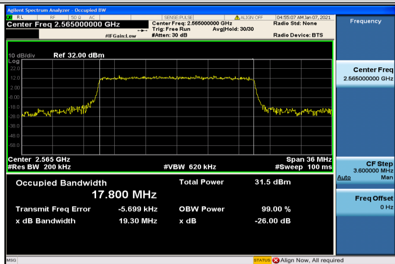
Band41-20MHz-QPSK-40340-100RB#0-17.800
