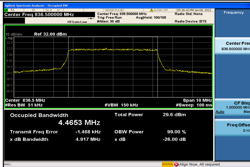
Band26-5MHz-QPSK-26915-25RB#0-4.4653
