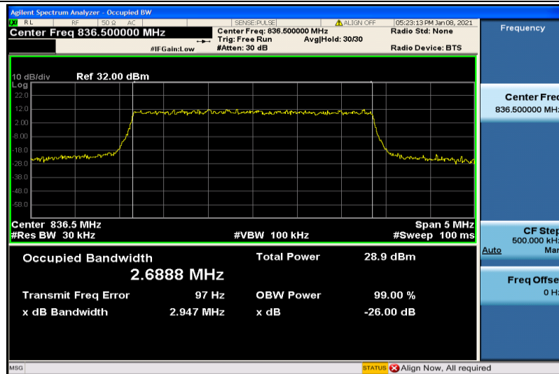
Band26-3MHz-QPSK-26915-15RB#0-2.6888
