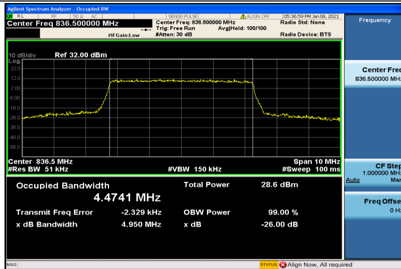
Band26-5MHz-16QAM-26915-25RB#0-4.4741
