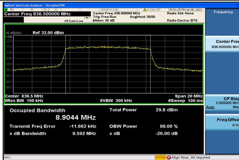
Band26-10MHz-QPSK-26915-50RB#0-8.9044
