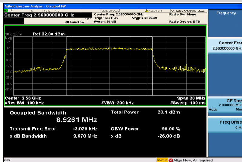
Band41-10MHz-16QAM-40290-50RB#0-8.9261
