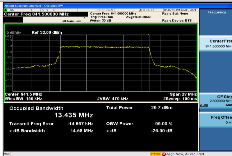
Band26-15MHz-QPSK-26965-75RB#0-13.435
