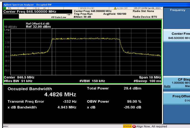
Band26-5MHz-QPSK-27015-25RB#0-4.4826
