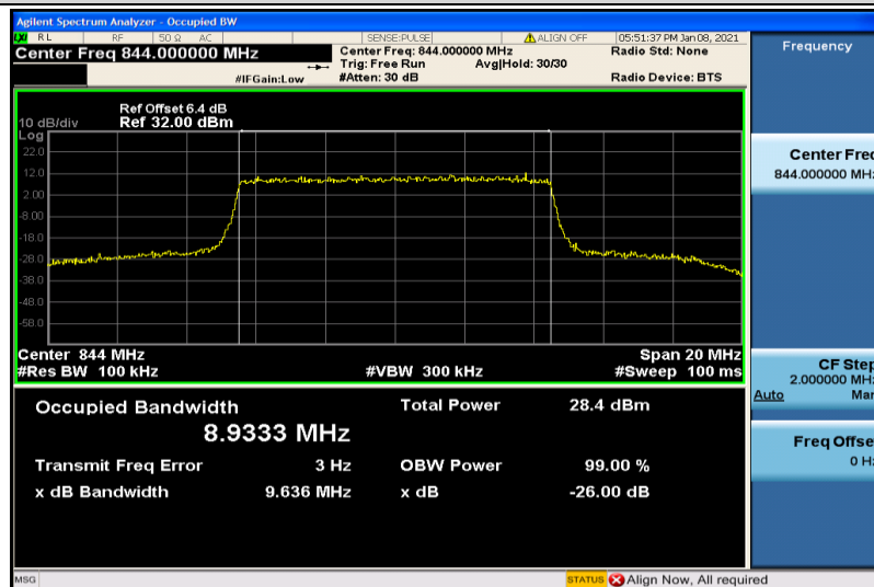
Band26-10MHz-16QAM-26990-50RB#0-8.9333
