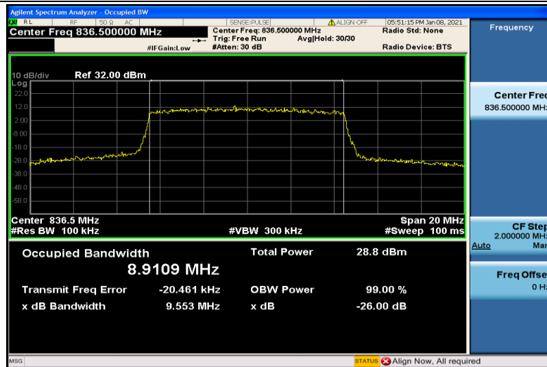
Band26-10MHz-16QAM-26915-50RB#0-8.9109
