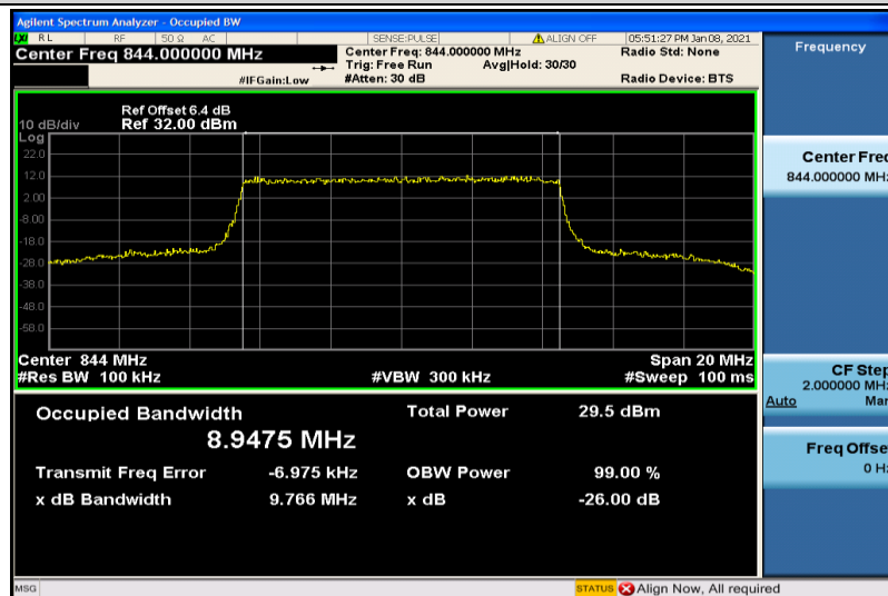
Band26-10MHz-QPSK-26990-50RB#0-8.9475
