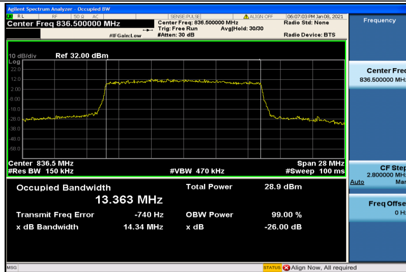
Band26-15MHz-QPSK-26915-75RB#0-13.363
