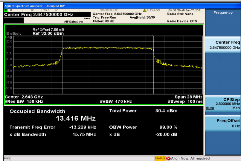
Band41-15MHz-16QAM-41165-75RB#0-13.416
