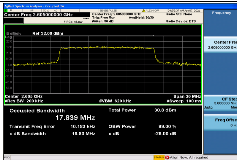
Band41-20MHz-16QAM-40740-100RB#0-17.839
