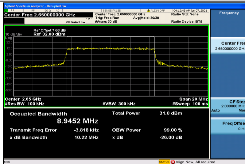
Band41-10MHz-QPSK-41190-50RB#0-8.9452
