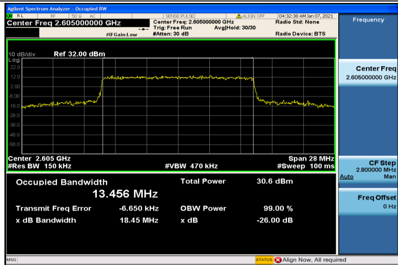
Band41-15MHz-16QAM-40740-75RB#0-13.456
