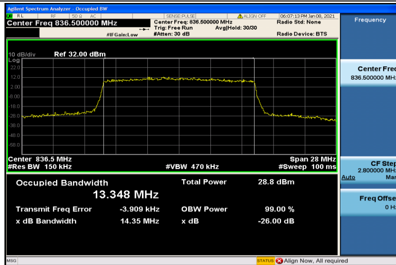
Band26-15MHz-16QAM-26915-75RB#0-13.348
