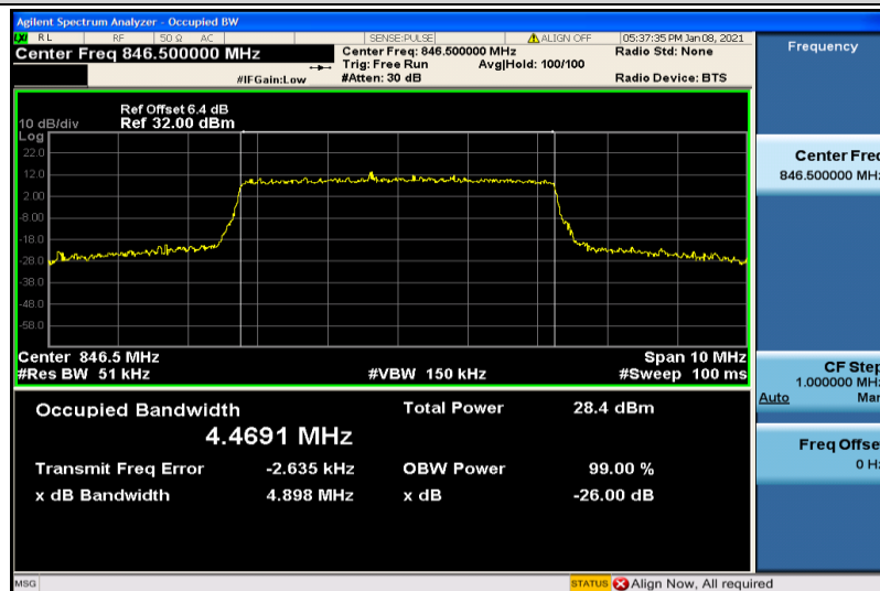
Band26-5MHz-16QAM-27015-25RB#0-4.4691
