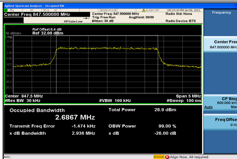
Band26-3MHz-QPSK-27025-15RB#0-2.6867
