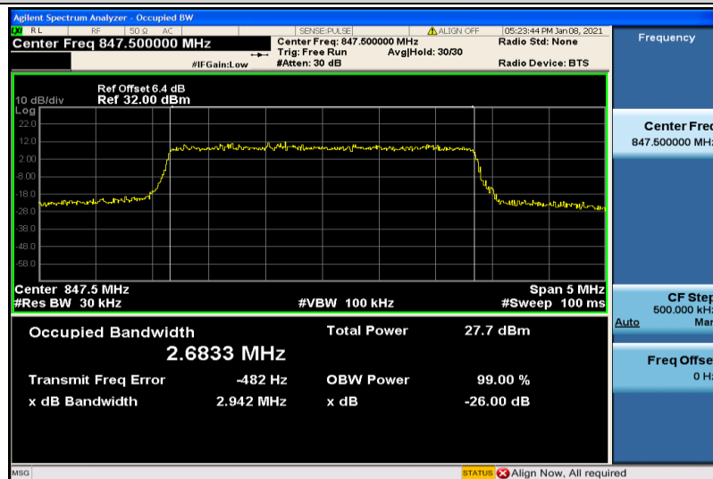
Band26-3MHz-16QAM-27025-15RB#0-2.6833
