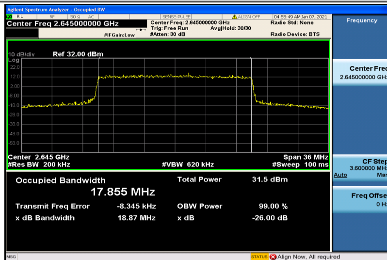
Band41-20MHz-QPSK-41140-100RB#0-17.855
