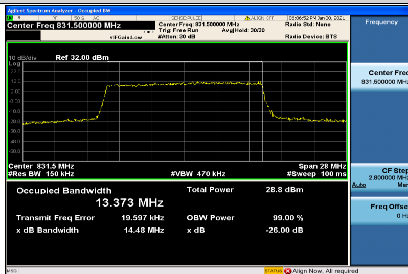
Band26-15MHz-16QAM-26865-75RB#0-13.373
