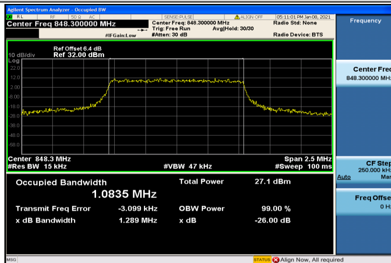
Band26-1.4MHz-16QAM-27033-6RB#0-1.0835
