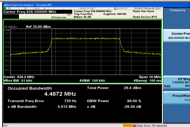
Band26-5MHz-QPSK-26815-25RB#0-4.4872
