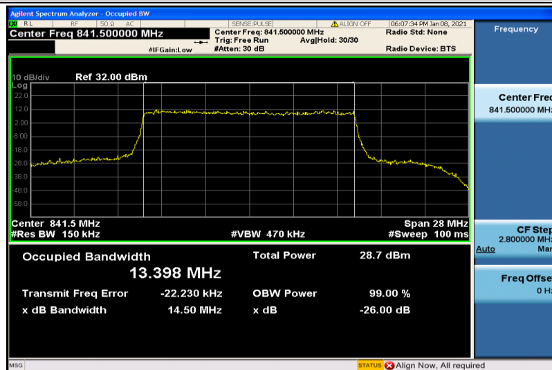
Band26-15MHz-16QAM-26965-75RB#0-13.398
