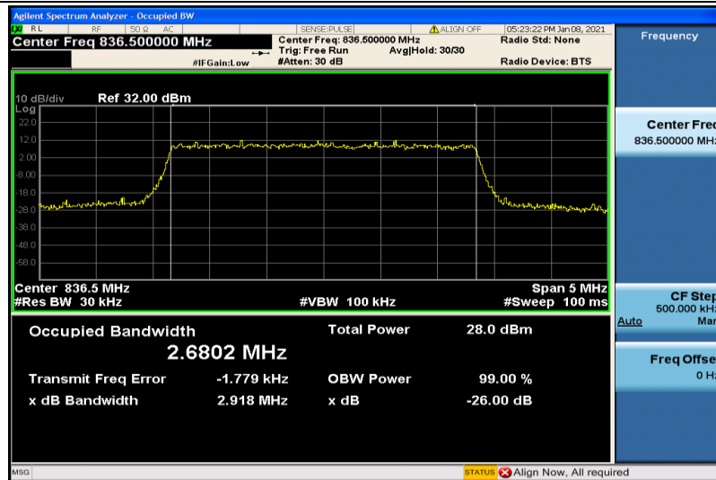
Band26-3MHz-16QAM-26915-15RB#0-2.6802
