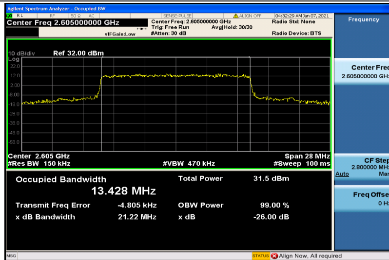
Band41-15MHz-QPSK-40740-75RB#0-13.428
