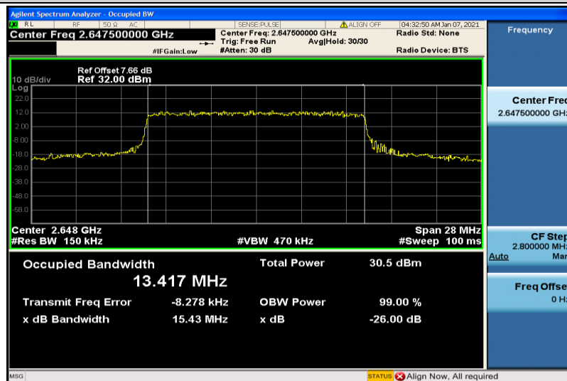
Band41-15MHz-QPSK-41165-75RB#0-13.417
