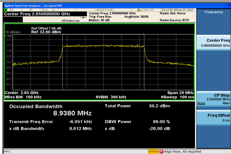
Band41-10MHz-16QAM-41190-50RB#0-8.9380
