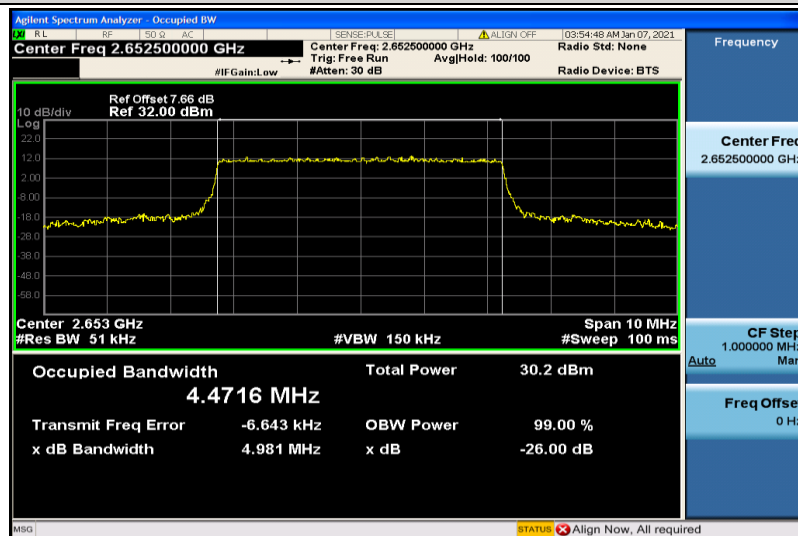
Band41-5MHz-16QAM-41215-25RB#0-4.4716
