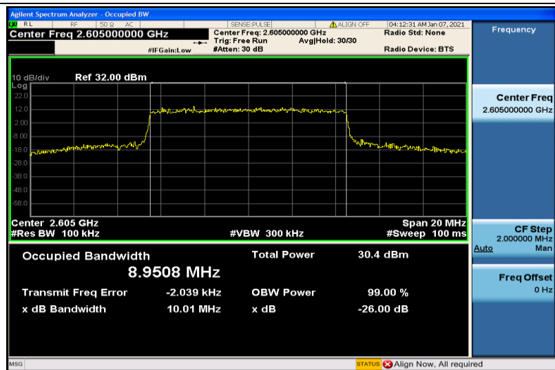
Band41-10MHz-16QAM-40740-50RB#0-8.9508
