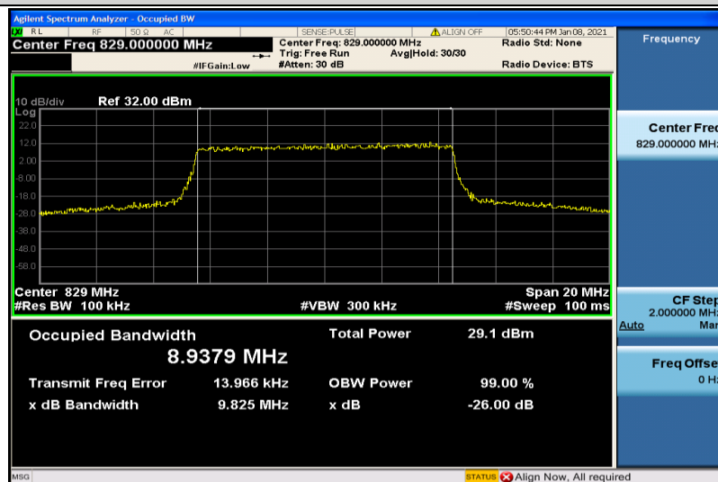
Band26-10MHz-QPSK-26840-50RB#0-8.9379
