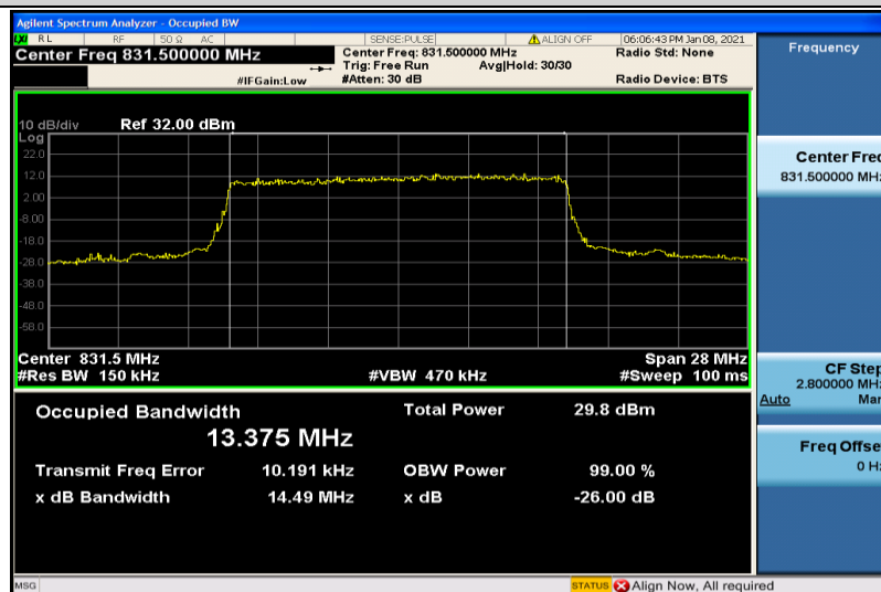
Band26-15MHz-QPSK-26865-75RB#0-13.375
