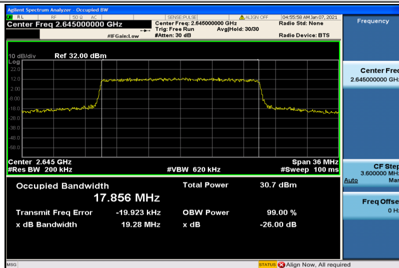
Band41-20MHz-16QAM-41140-100RB#0-17.856
