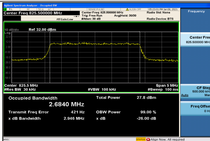
Band26-3MHz-16QAM-26805-15RB#0-2.6840
