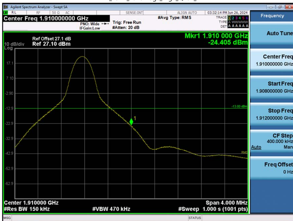
LTE B2_15 M_Band Edge_High_QPSK_1RB
