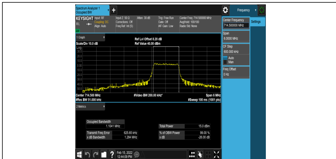
Band12-3MHz-16QAM-23165-6-0-High-1.1041-1.284-PASS
