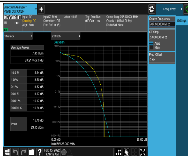
Band12-3MHz-QPSK-23095-6-0-Low-9.62-≤13-PASS
