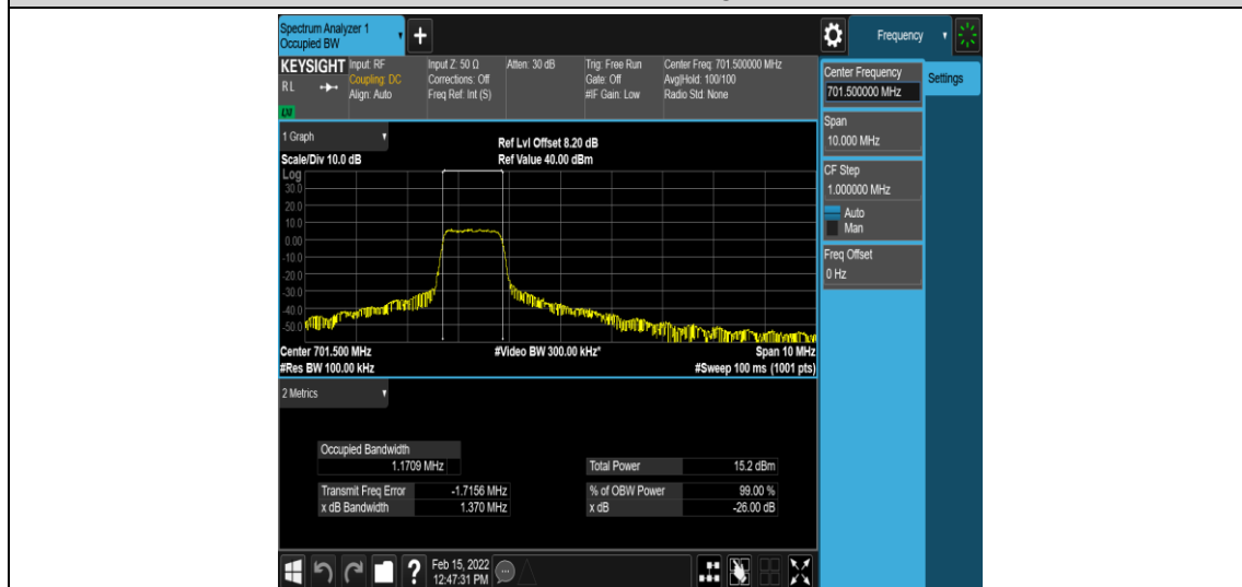
Band12-5MHz-QPSK-23035-6-0-Low-1.1709-1.370-PASS
