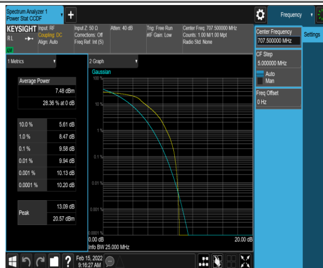
Band12-3MHz-16QAM-23095-6-0-Low-9.58-&lt;=13-PASS
