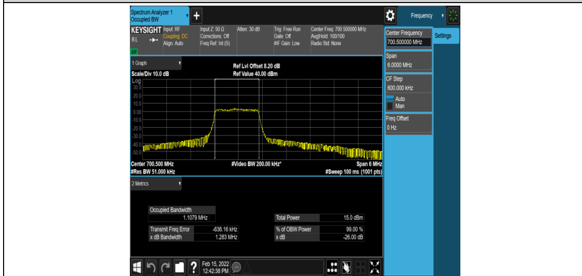
Band12-3MHz-QPSK-23025-6-0-Low-1.1079-1.283-PASS
