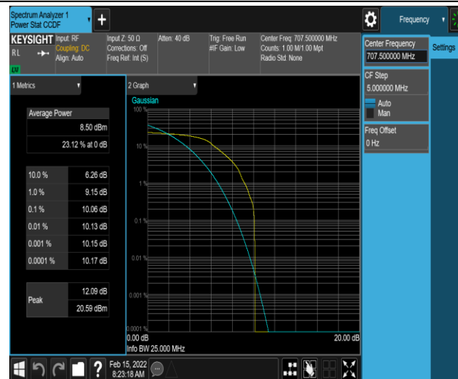
Band12-1.4MHz-QPSK-23095-1-0-Low-10.06-<=13-PASS
