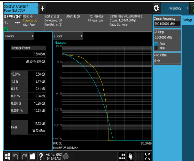
Band12-3MHz-16QAM-23025-6-0-Low-9.44-&lt;=13-PASS
