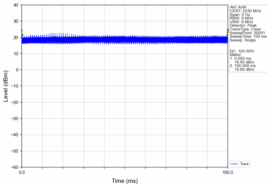
40M_HCH_5230MHz_Ant4_NTNV
