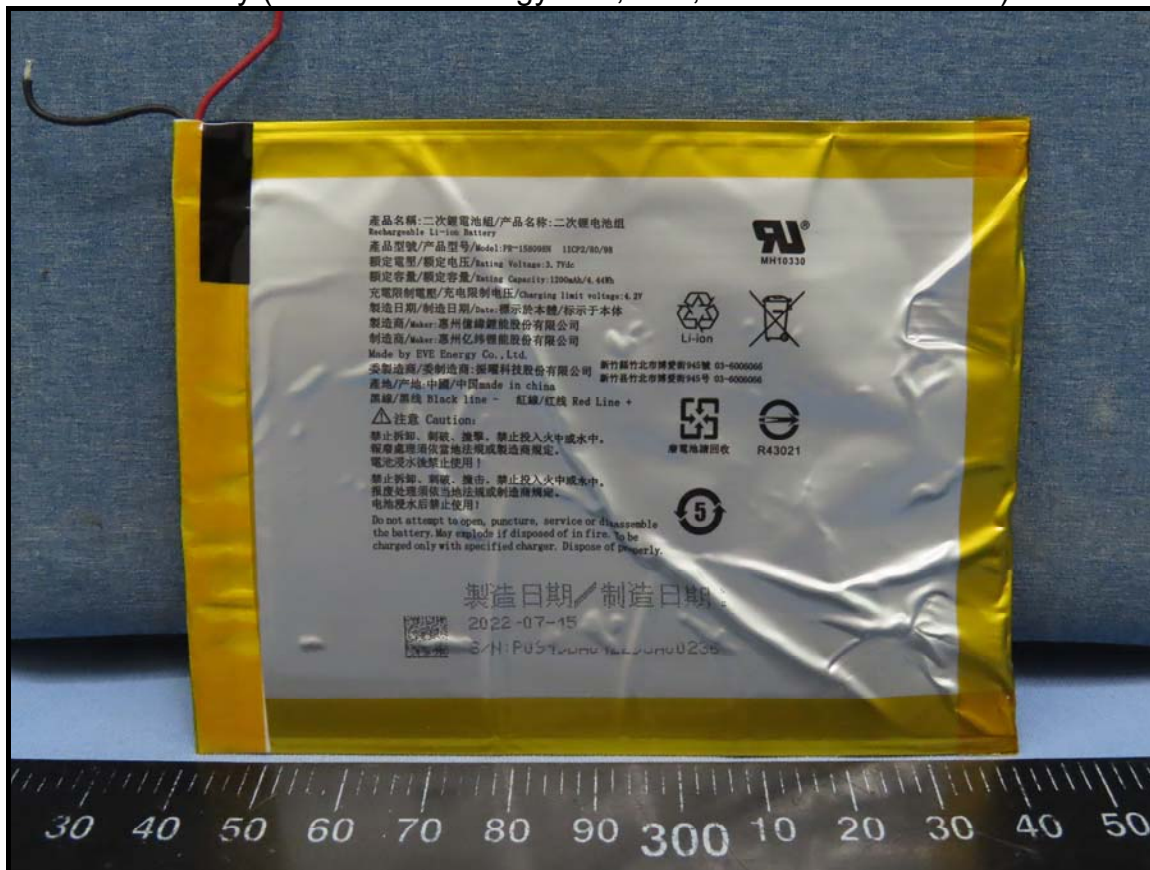
Battery (Brand: EVE Energy CO., LTD, Model: PR-158098N)
