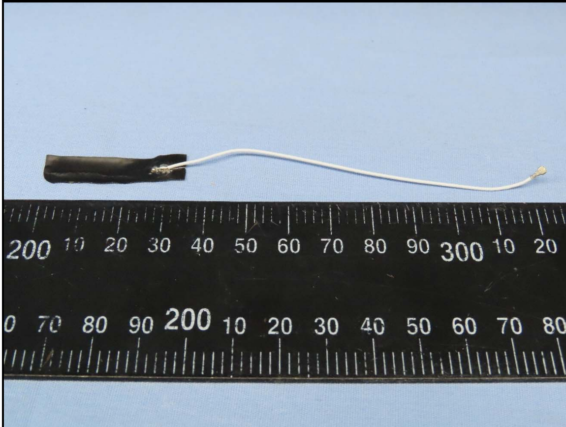
Antenna (Brand: INPAQ, Model: RFFPA360911EMLB101)
