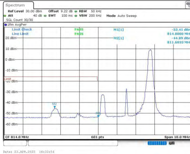
Band26@90-3MHz-16QAM-26705-1RB#14
