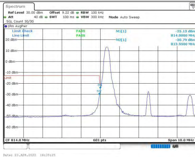
Band26@90-5MHz-QPSK-26715-1RB#0
