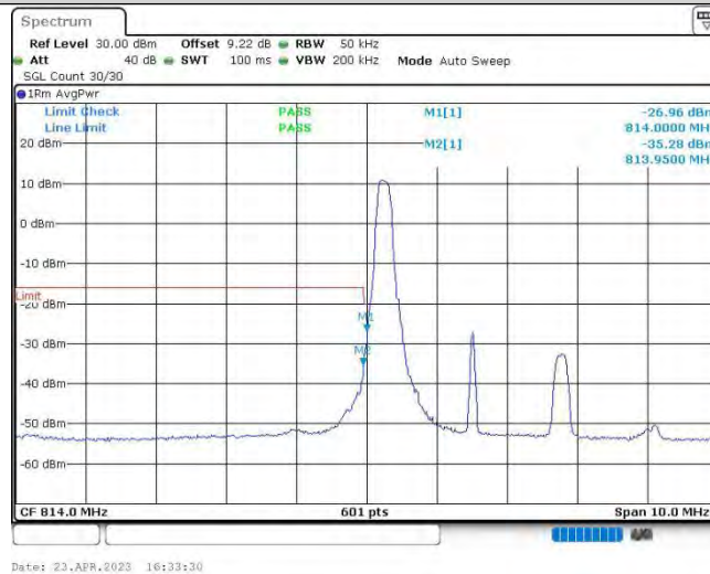
Band26@90-3MHz-QPSK-26705-1RB#0
