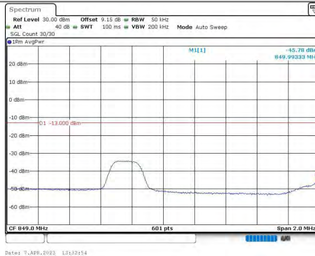
Band5-3MHz-16QAM-20635-1RB#0
