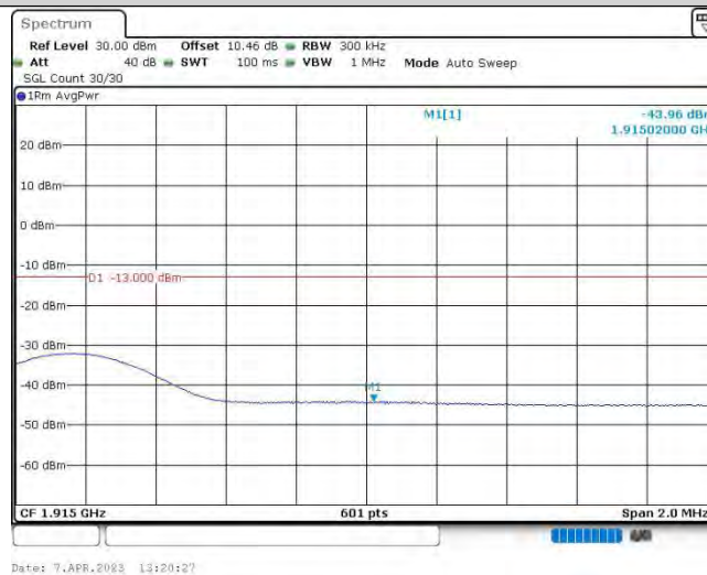
Band25-15MHz-16QAM-26615-1RB#0
