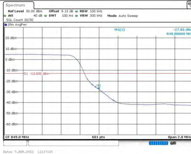
Band5-5MHz-16QAM-20625-25RB#0
