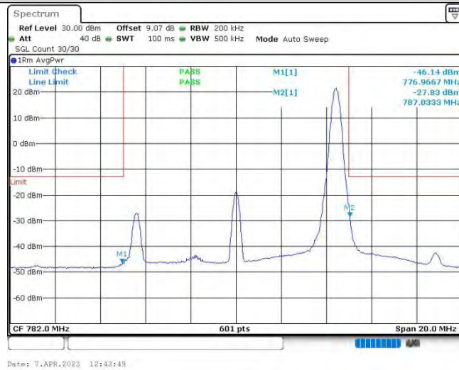
Band13-10MHz-16QAM-23230-1RB#49
