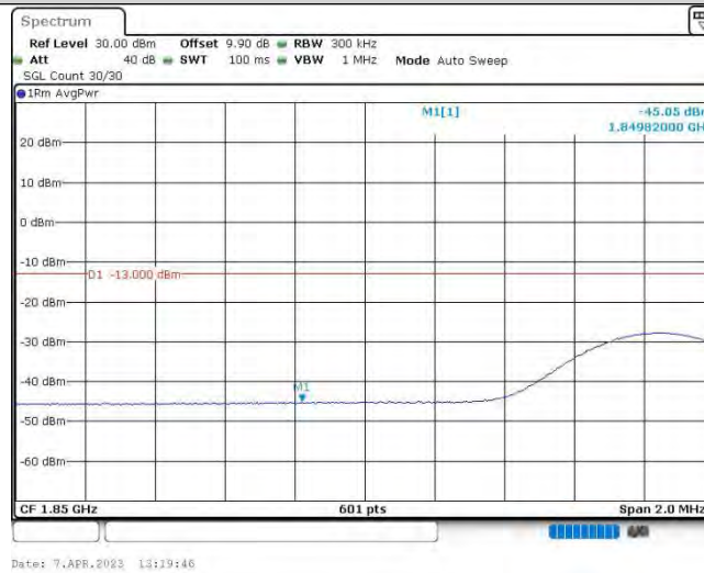
Band25-15MHz-16QAM-26115-1RB#74
