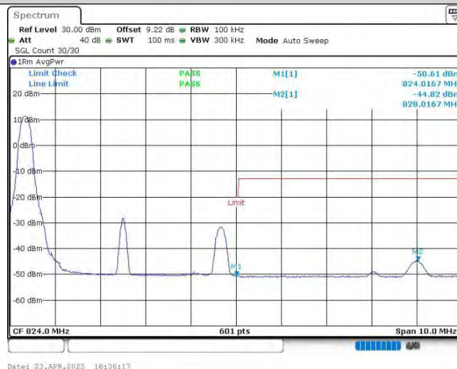
Band26@90-5MHz-QPSK-26765-1RB#0
