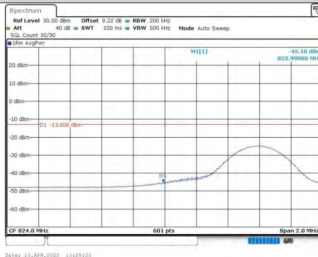
Band5-10MHz-QPSK-20450-1RB#49
