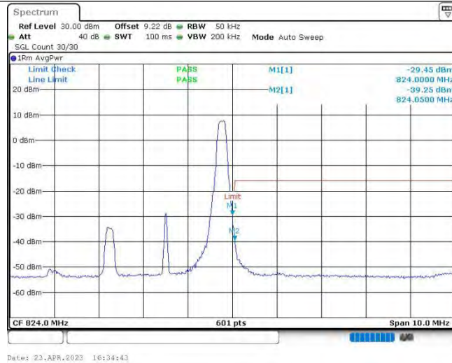
Band26@90-3MHz-16QAM-26775-1RB#14
