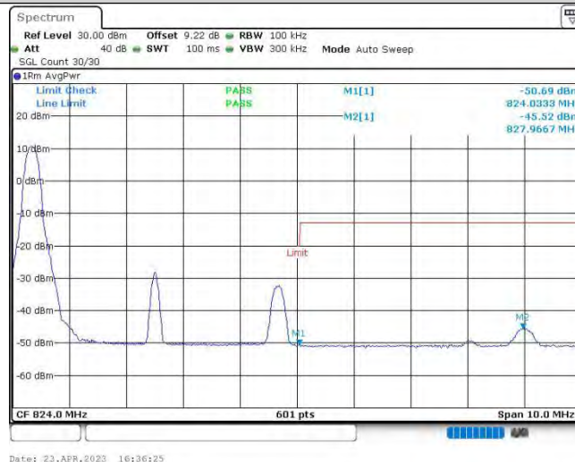
Band26@90-5MHz-16QAM-26765-1RB#0
