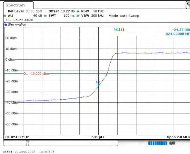
Band26@22-3MHz-QPSK-26805-15RB#0
