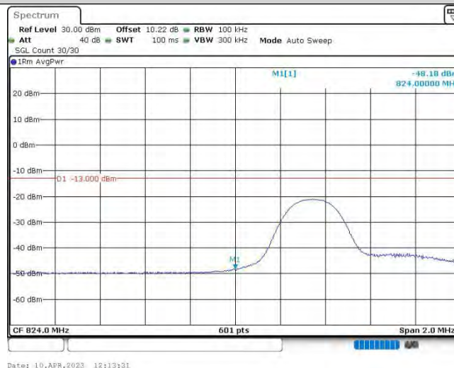
Band26@22-5MHz-QPSK-26815-1RB#24
