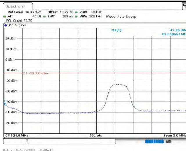
Band26@22-3MHz-QPSK-26805-1RB#14
