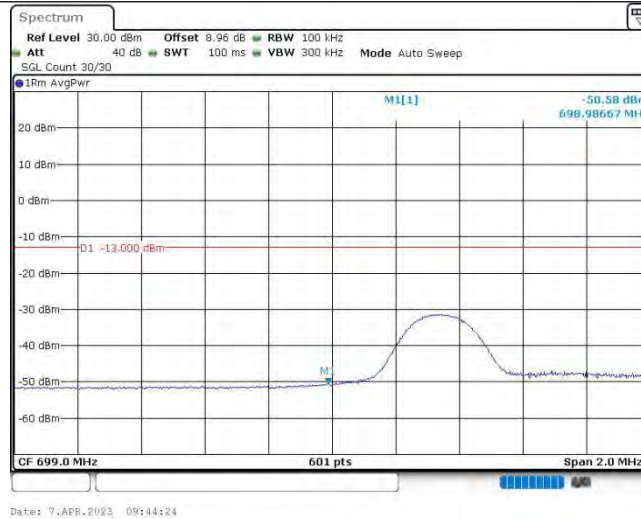
Band12-5MHz-16QAM-23035-1RB#24
