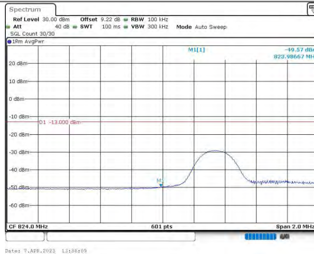
Band5-5MHz-16QAM-20425-1RB#24
