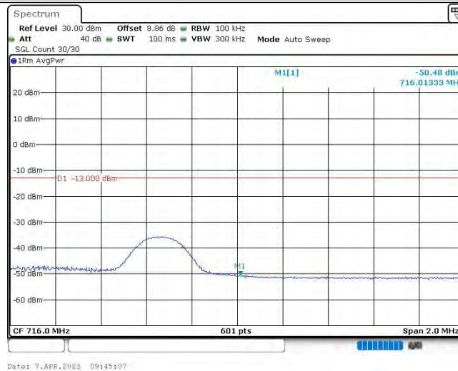
Band12-5MHz-16QAM-23155-1RB#0
