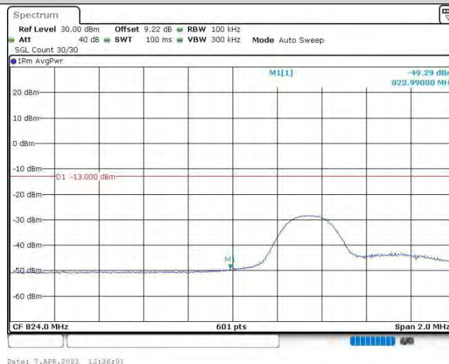
Band5-5MHz-QPSK-20425-1RB#24
