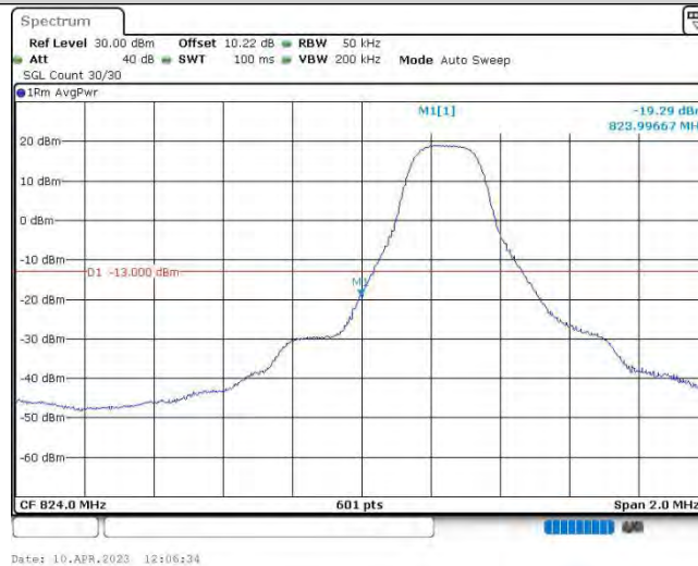
Band26@22-3MHz-QPSK-26805-1RB#0
