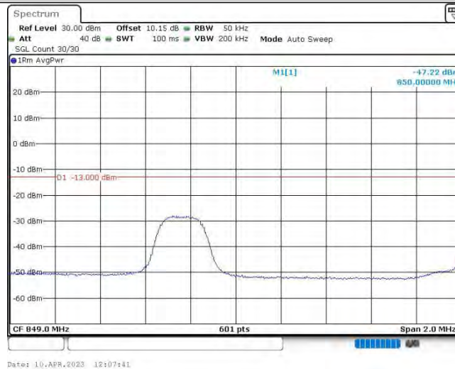
Band26@22-3MHz-16QAM-27025-1RB#0
