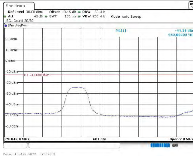
Band26@22-3MHz-QPSK-27025-1RB#0
