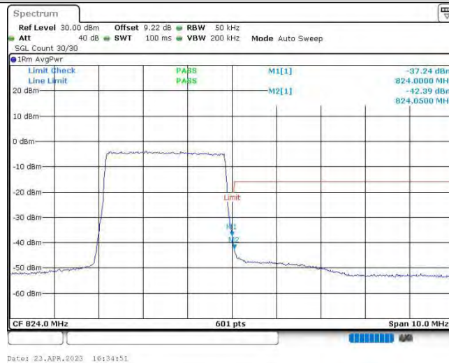
Band26@90-3MHz-QPSK-26775-15RB#0
