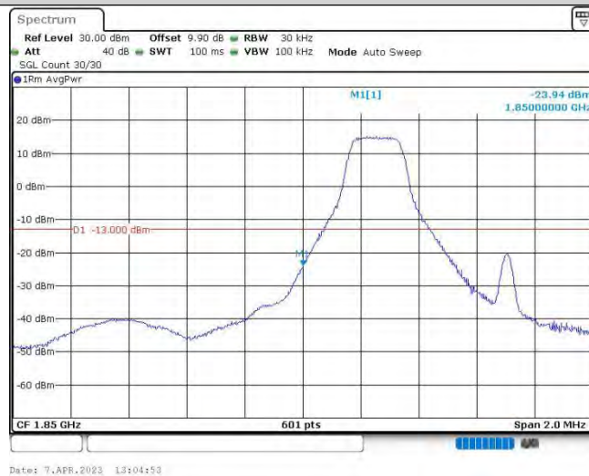
Band25-1.4MHz-QPSK-26047-1RB#0
