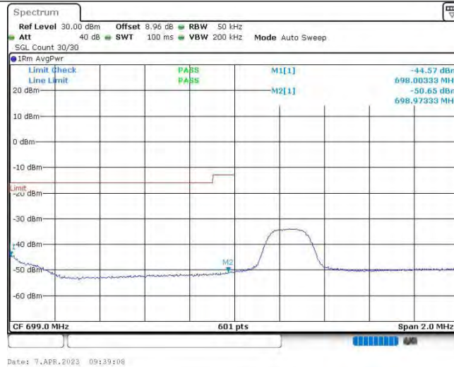
Band12-3MHz-QPSK-23025-1RB#14
