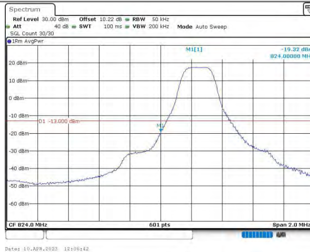
Band26@22-3MHz-16QAM-26805-1RB#0
