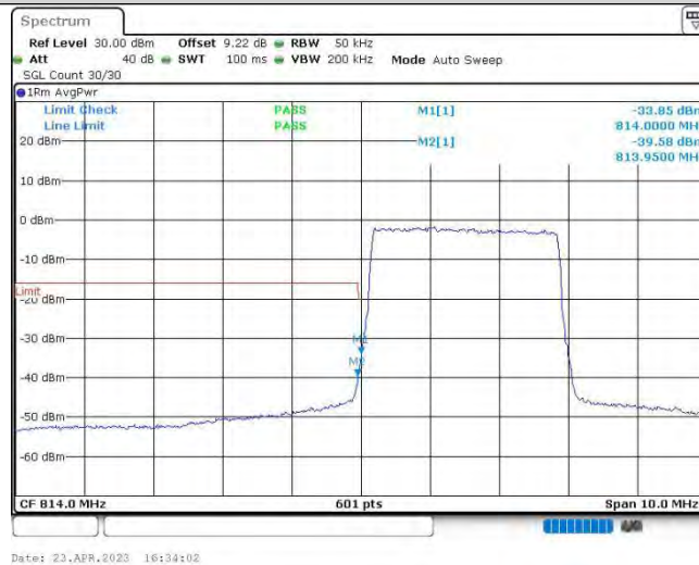
Band26@90-3MHz-QPSK-26705-15RB#0
