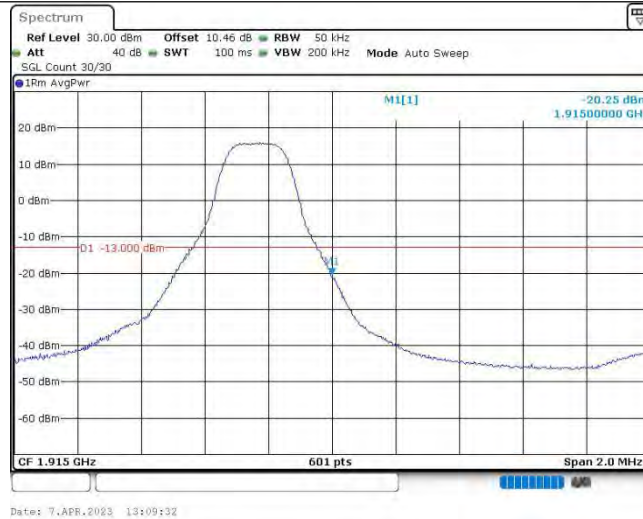
Band25-3MHz-16QAM-26675-1RB#14
