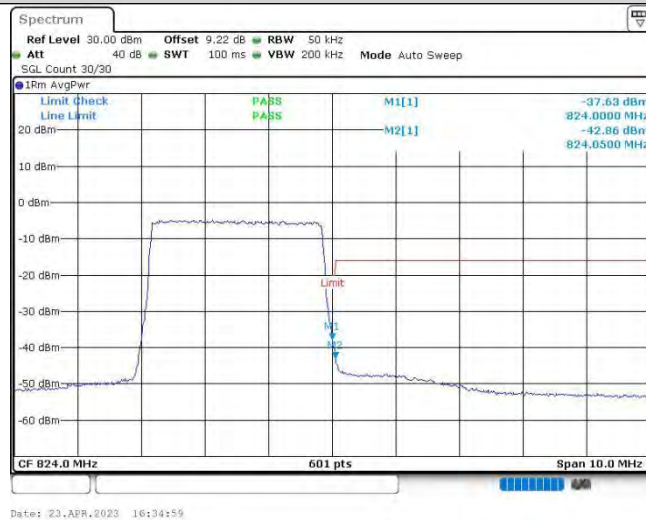
Band26@90-3MHz-16QAM-26775-15RB#0
