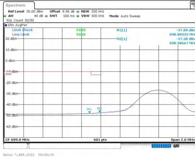
Band12-10MHz-16QAM-23060-1RB#49
