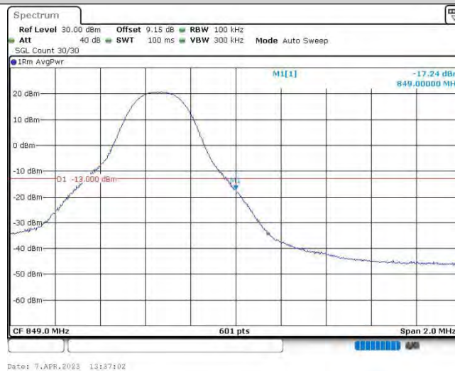
Band5-5MHz-QPSK-20625-1RB#24
