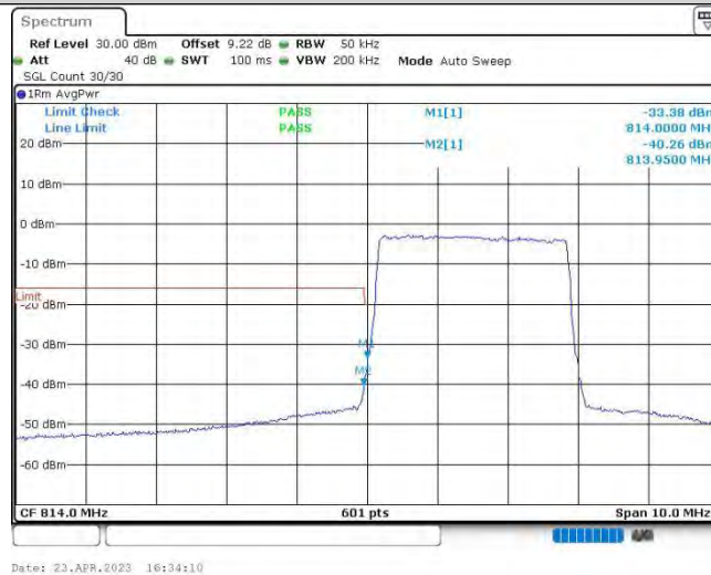
Band26@90-3MHz-16QAM-26705-15RB#0
