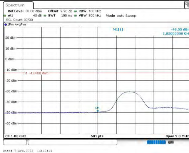
Band25-5MHz-QPSK-26065-1RB#24
