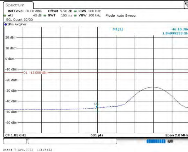
Band25-10MHz-QPSK-26090-1RB#49
