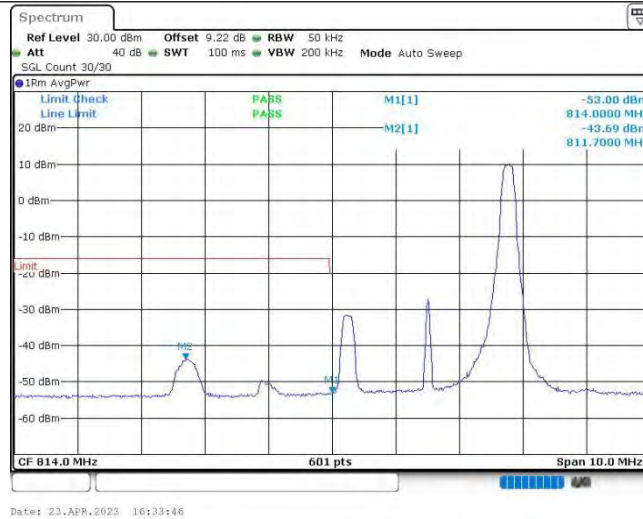
Band26@90-3MHz-QPSK-26705-1RB#14
