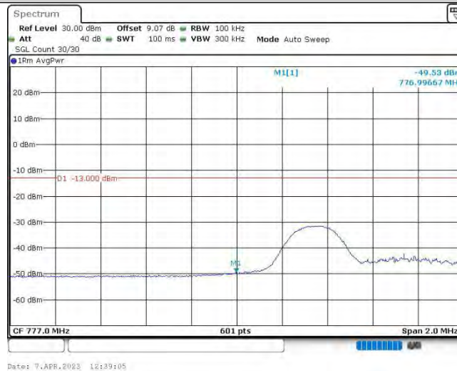
Band13-5MHz-QPSK-23205-1RB#24
