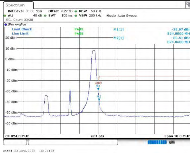
Band26@90-3MHz-QPSK-26775-1RB#14
