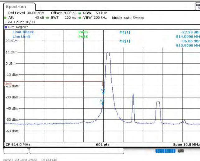
Band26@90-3MHz-16QAM-26705-1RB#0
