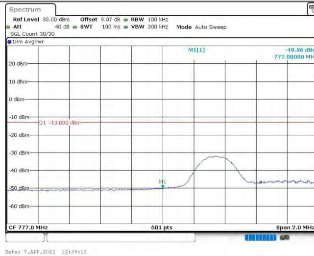
Band13-5MHz-16QAM-23205-1RB#24
