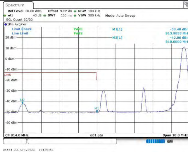
Band26@90-5MHz-16QAM-26715-1RB#24
