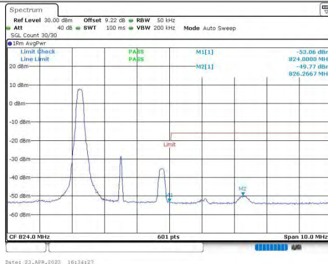
Band26@90-3MHz-16QAM-26775-1RB#0
