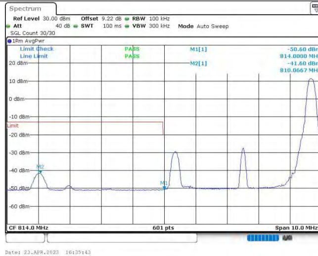
Band26@90-5MHz-QPSK-26715-1RB#24
