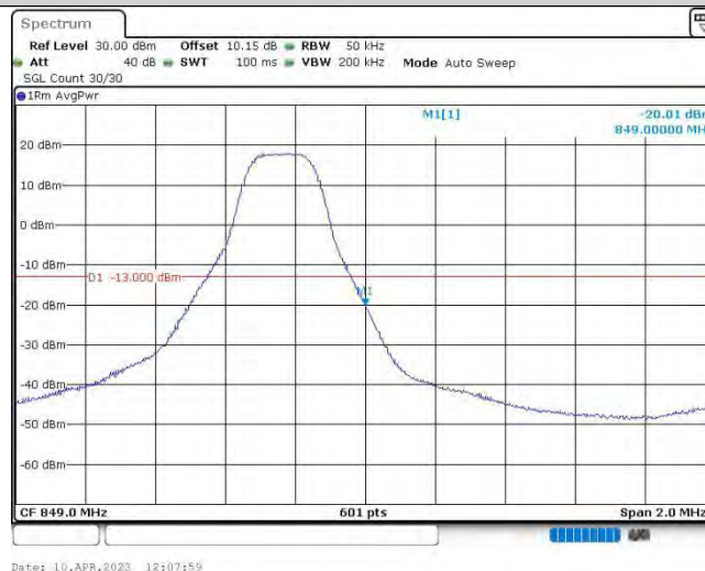
Band26@22-3MHz-16QAM-27025-1RB#14
