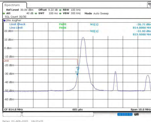
Band26@90-5MHz-16QAM-26715-1RB#0
