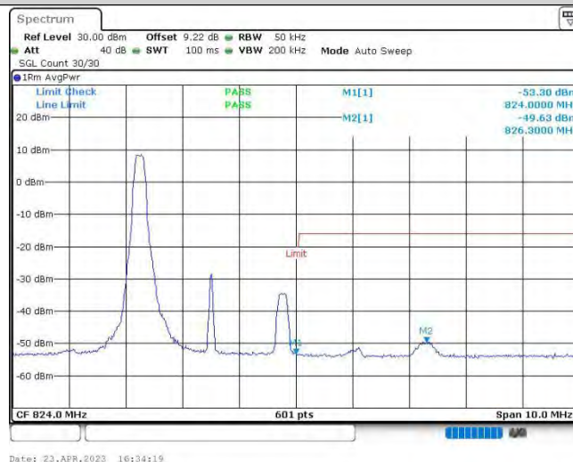
Band26@90-3MHz-QPSK-26775-1RB#0
