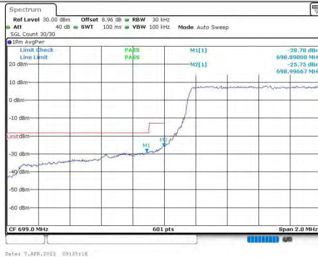
Band12-1.4MHz-QPSK-23017-6RB#0
