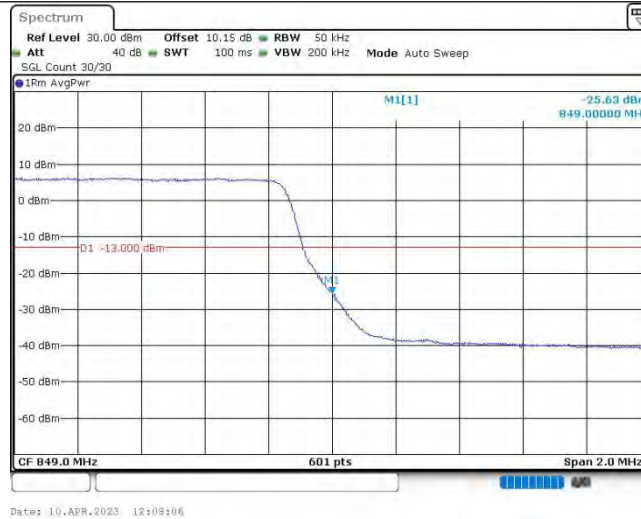
Band26@22-3MHz-QPSK-27025-15RB#0
