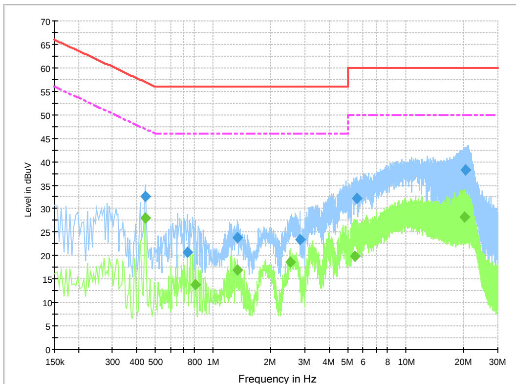
Figure A.14 Conducted Emission
