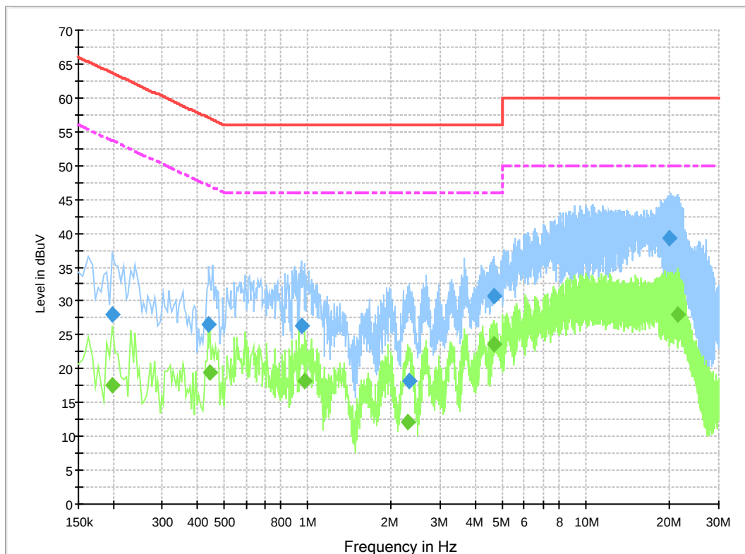
Figure A.15 Conducted Emission
