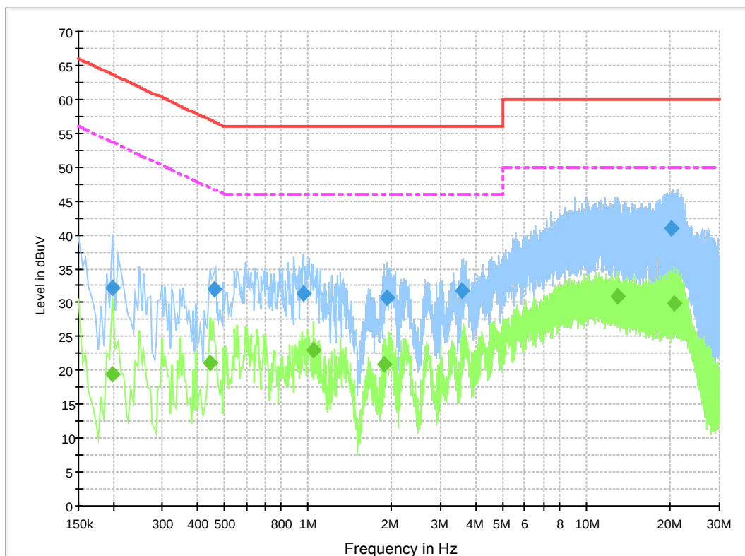
Figure A.17 Conducted Emission
