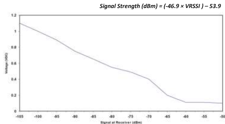
Figure 2: RSSI Voltage vs. Received Signal Strength
