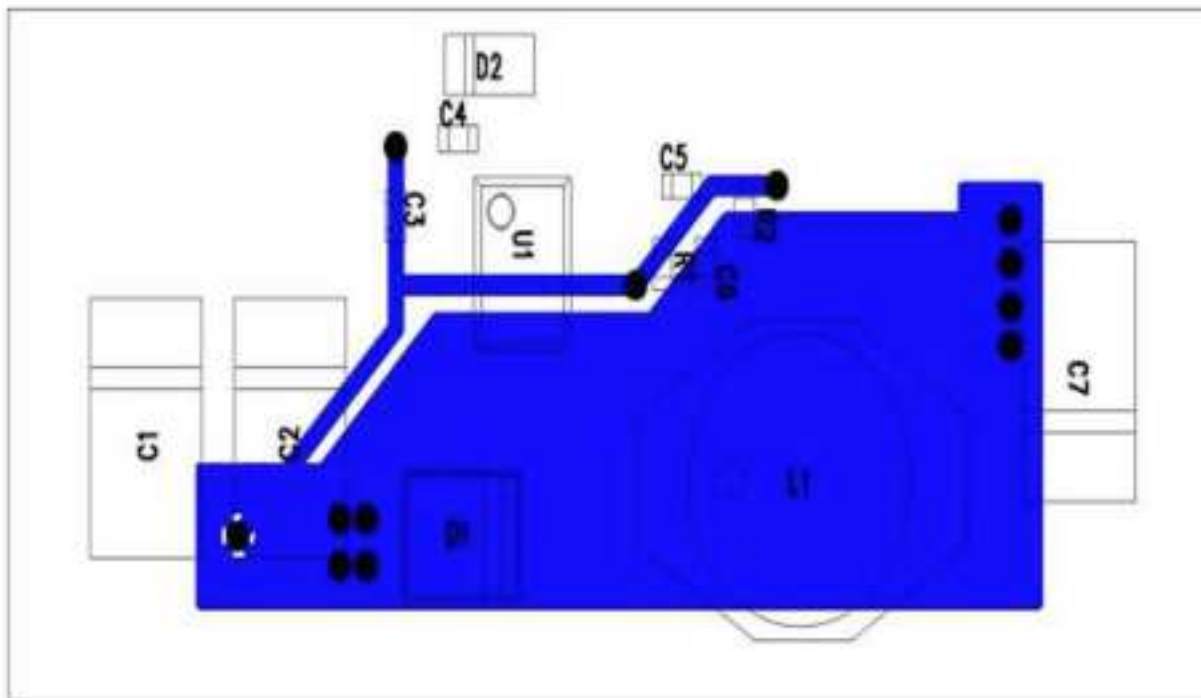
Figure 15: PCB Layout
