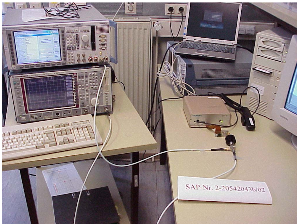
Photograph 7: Test site for conducted measurements (1)
