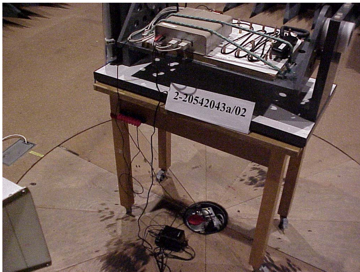
Photograph 5: Test setup for radiated emissions
