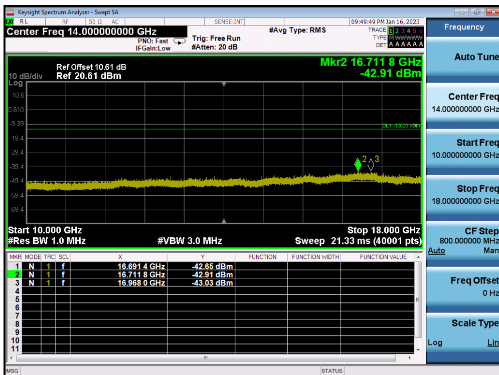
LTE Band 66(4) / 20MHz / 64QAM - RB Size/Offset (50/0) - High Channel
