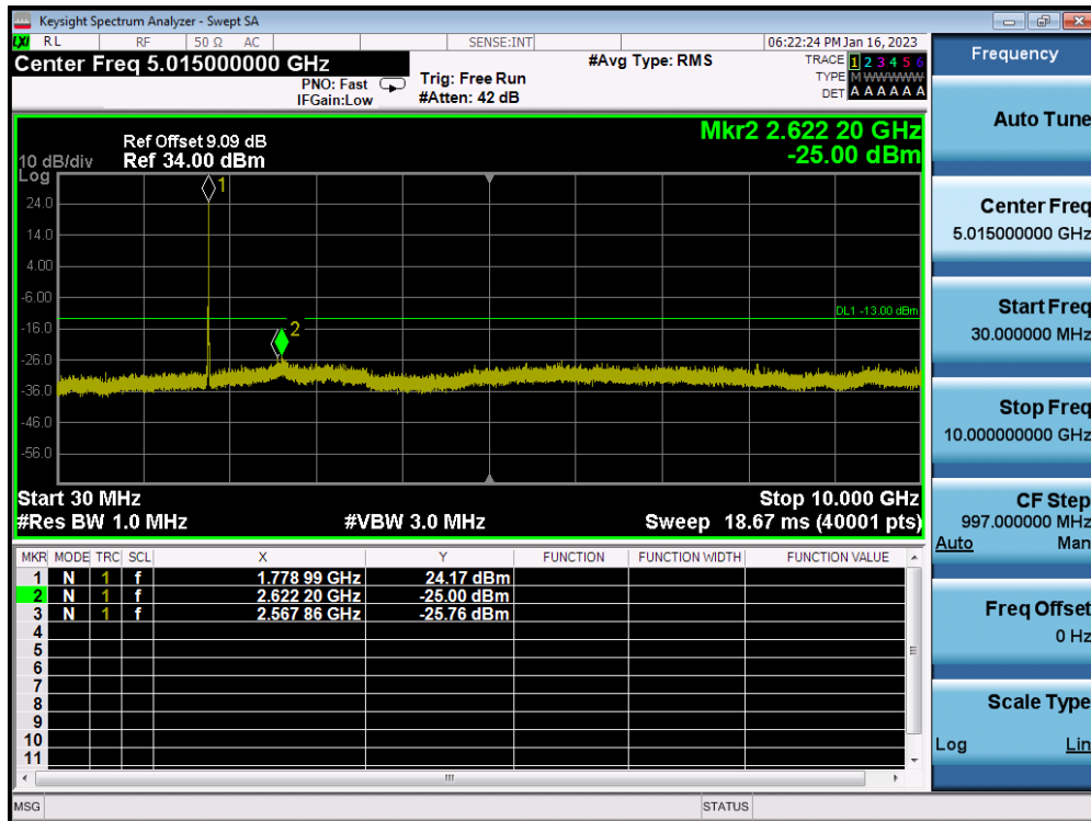
LTE Band 66(4) / 10MHz / 16QAM - RB Size/Offset (25/25) - High Channel
