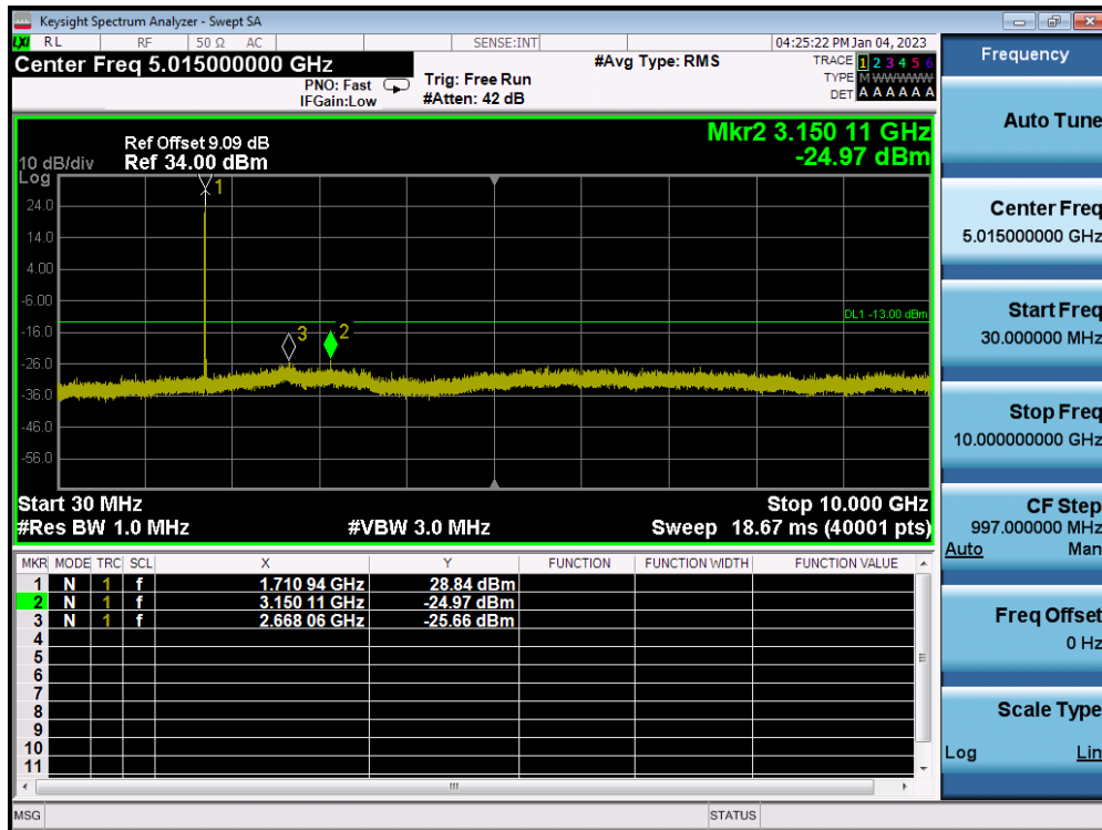
LTE Band 66(4) / 15MHz / 16QAM - RB Size/Offset (1/0) - Low Channel
