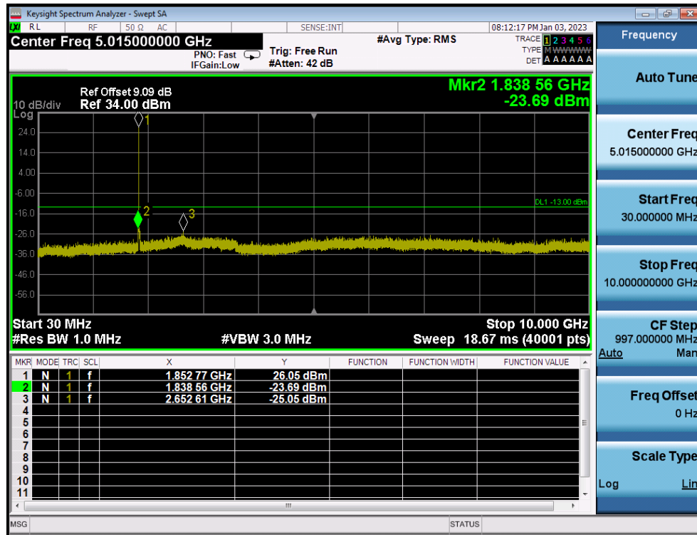
LTE Band 2 / 5MHz / QPSK - RB Size/Offset (25/0) - Low Channel
