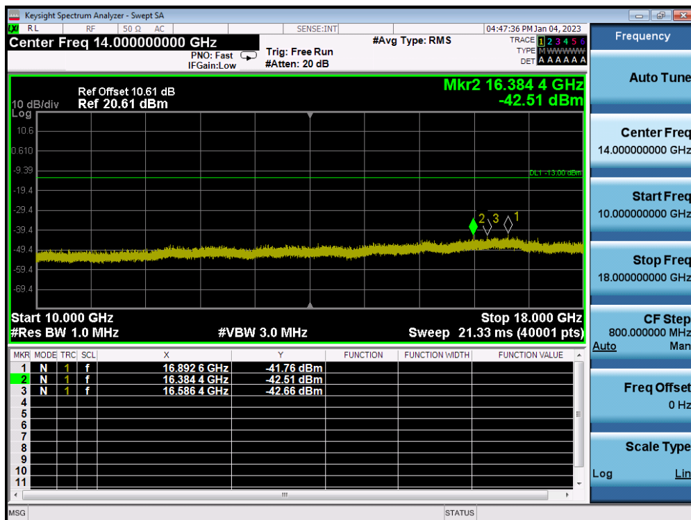
LTE Band 66(4) / 15MHz / 16QAM - RB Size/Offset (1/74) - Mid Channel
