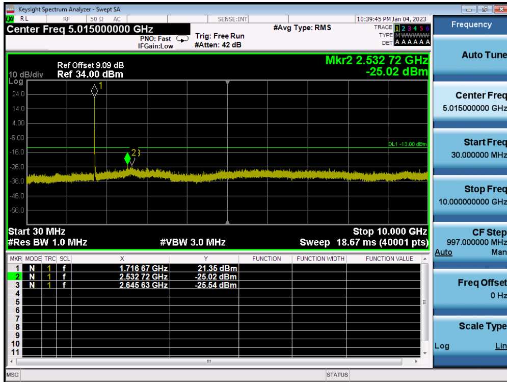
LTE Band 66(4) / 20MHz / 64QAM - RB Size/Offset (50/0) - Low Channel
