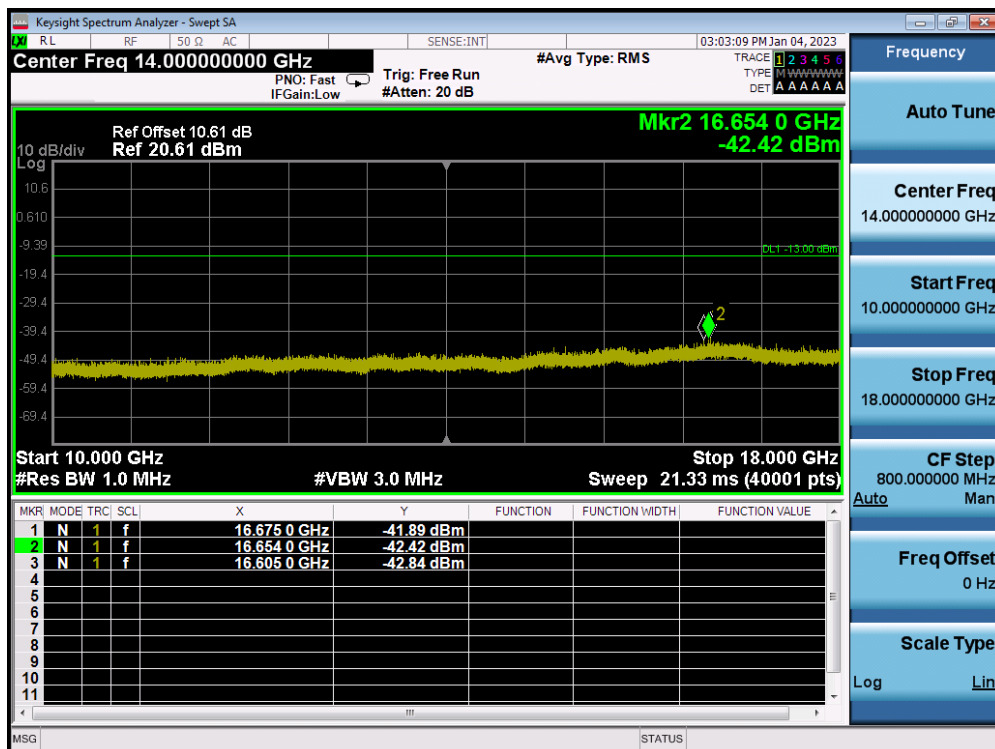
LTE Band 66(4) / 5MHz / 16QAM - RB Size/Offset (1/24) - Mid Channel
