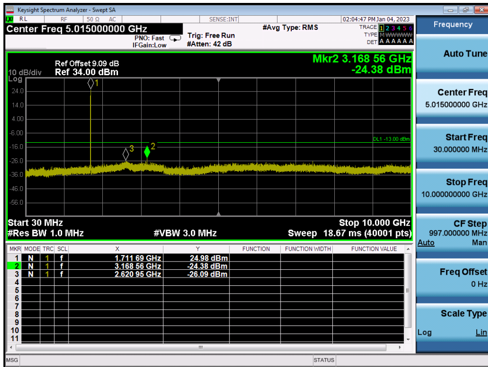
LTE Band 66(4) / 3MHz / 16QAM - RB Size/Offset (15/0) - Low Channel
