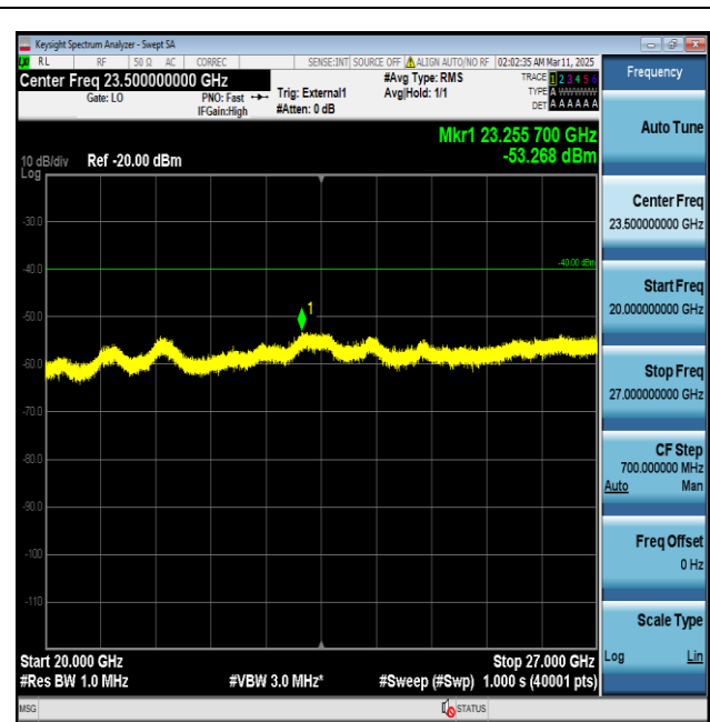
Band48-20MHz-QPSK-56640-1RB#0-20000~27000-PASS
