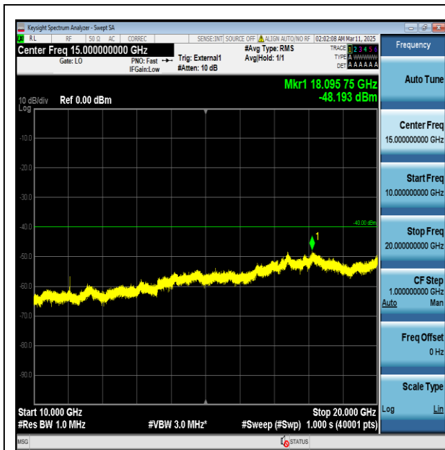
Band48-20MHz-QPSK-56640-1RB#0-10000~20000-PASS
