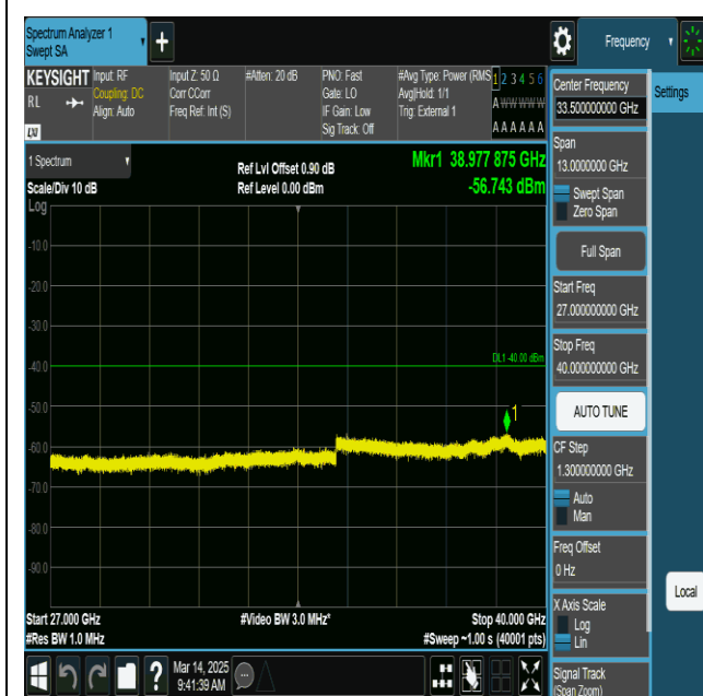
Band48-20MHz-QPSK-56440-1RB#0-27000~40000-PASS
