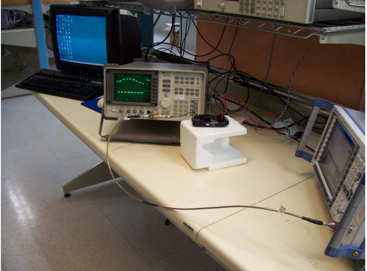
Bluetooth RF Conducted Emission Test-Setup Photo
