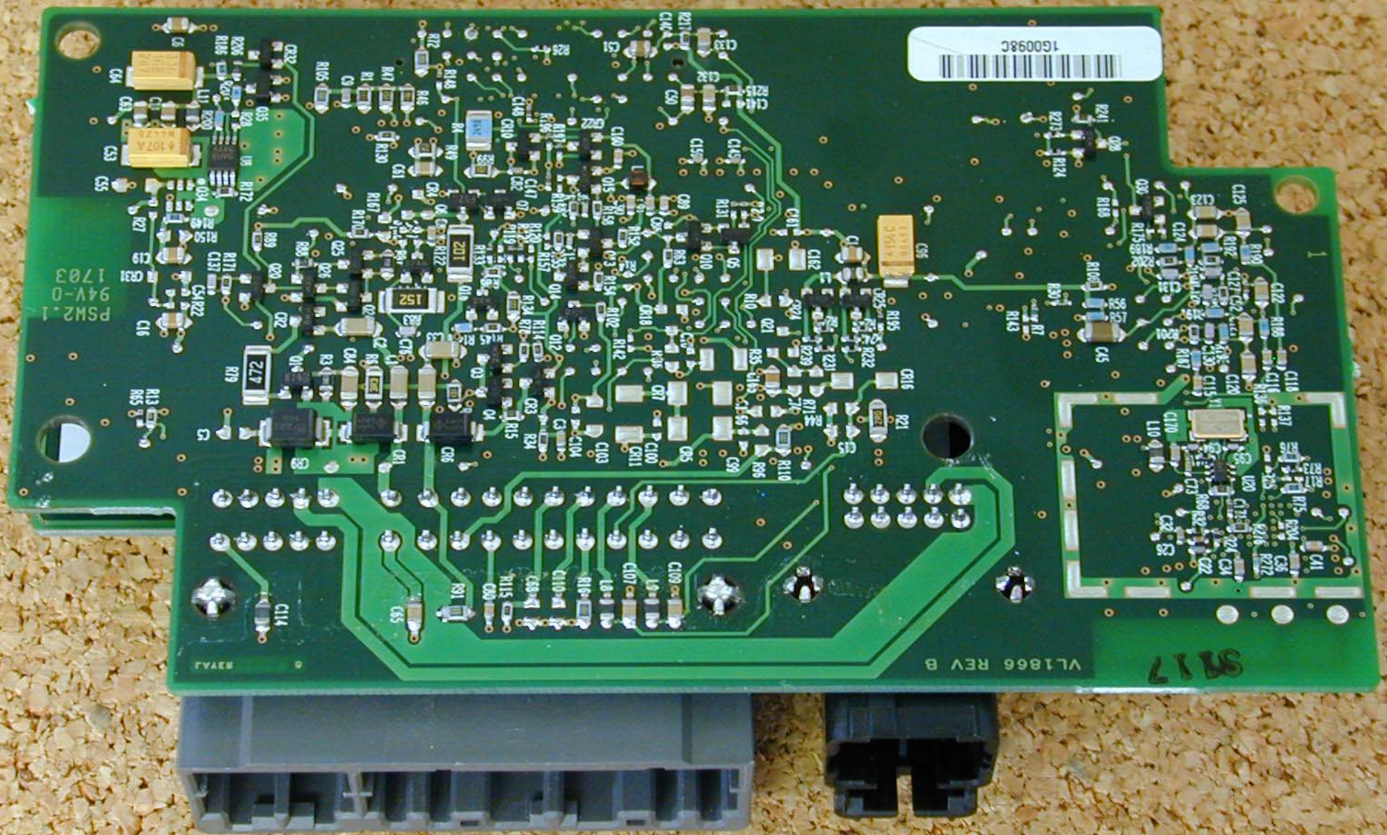
Module 05064022AE PCB (bottom)
