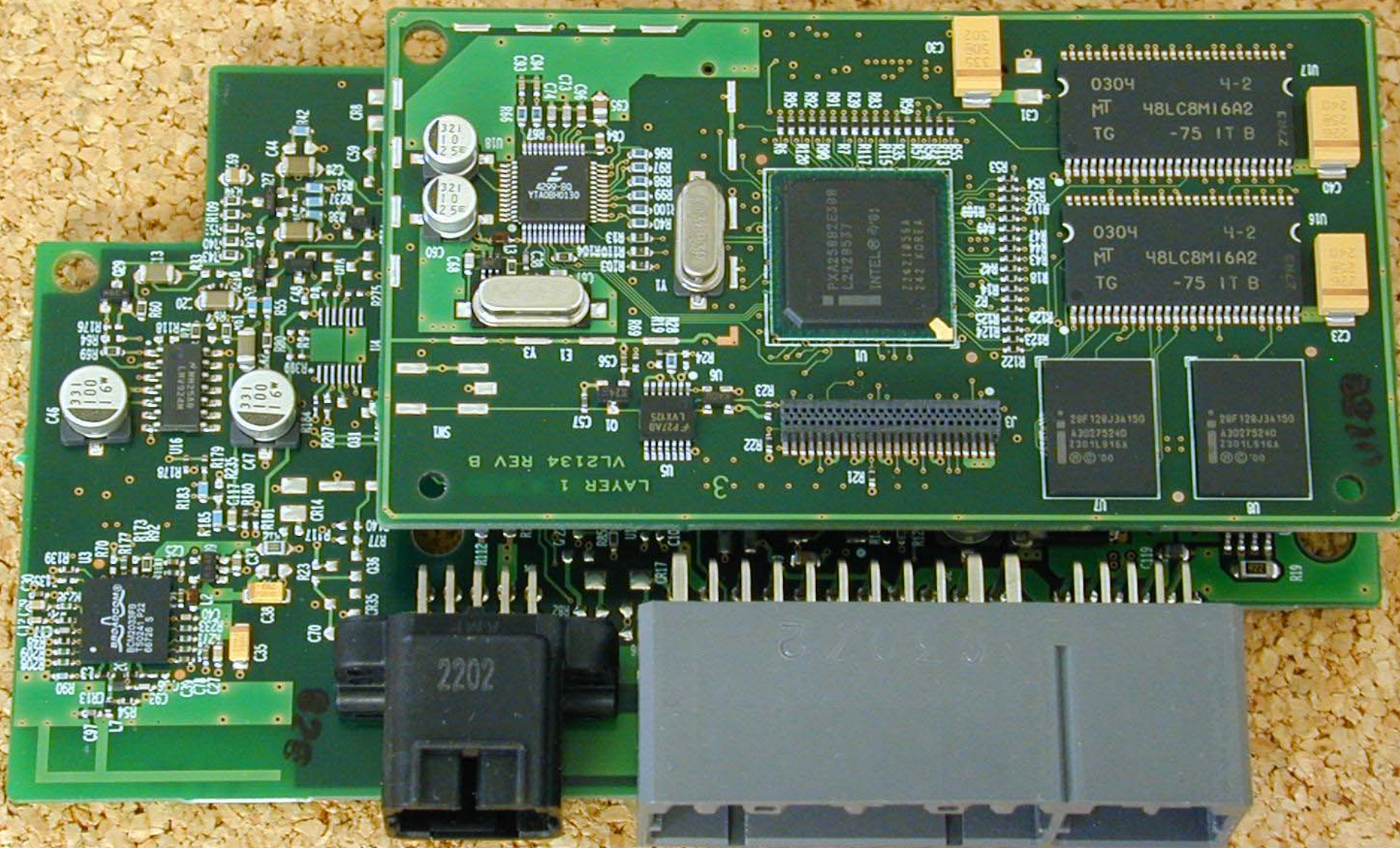
Module 05064022AE PCB (top)
