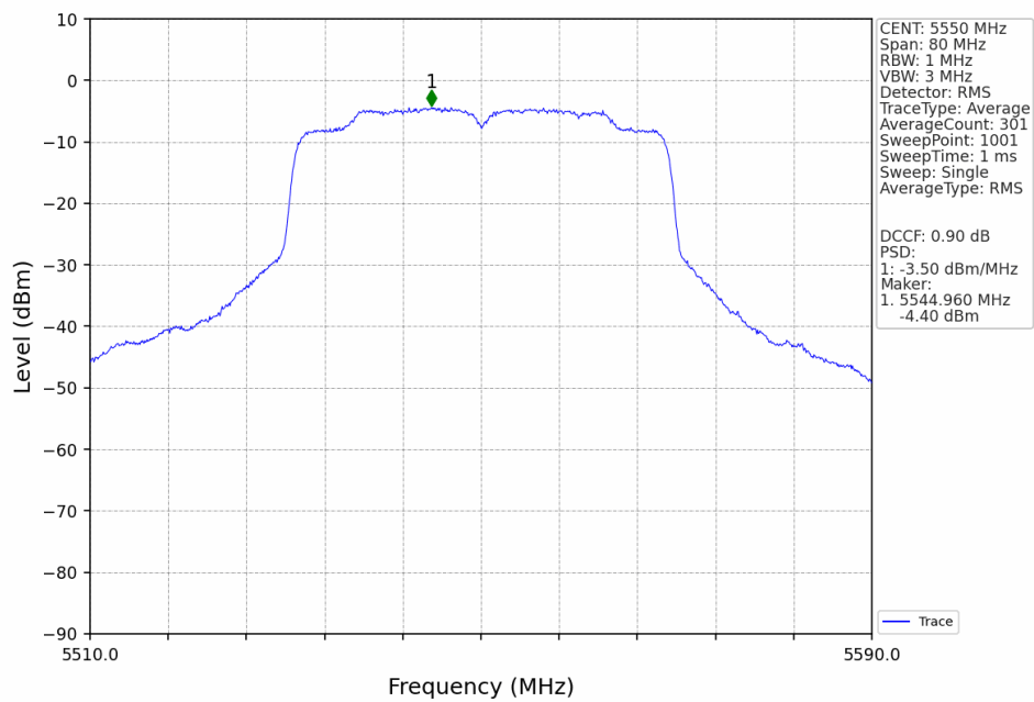
802.11ax(HEW40)_MCH_5550MHz_SU_ / Ant1_NTNV
