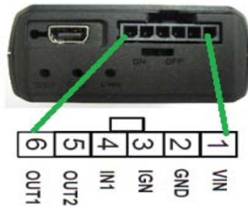
Figure 2. 6PIN Connector on GV55W
