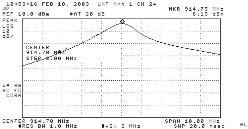
UHF Antenna Port 1, Channel 24
