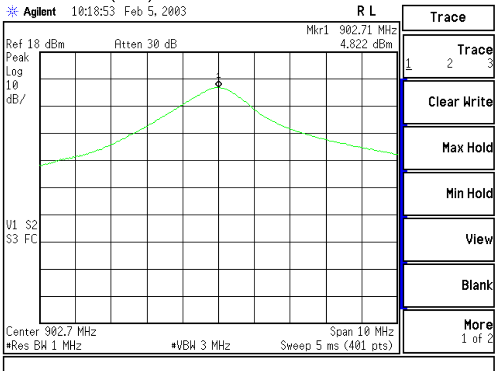
Peak output power UHF Antenna Port 1, Channel 0
