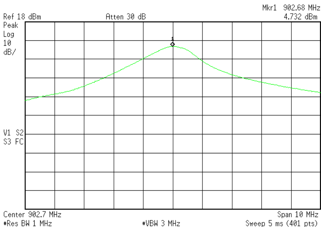
Peak output power UHF Antenna Port 2, Channel 0
