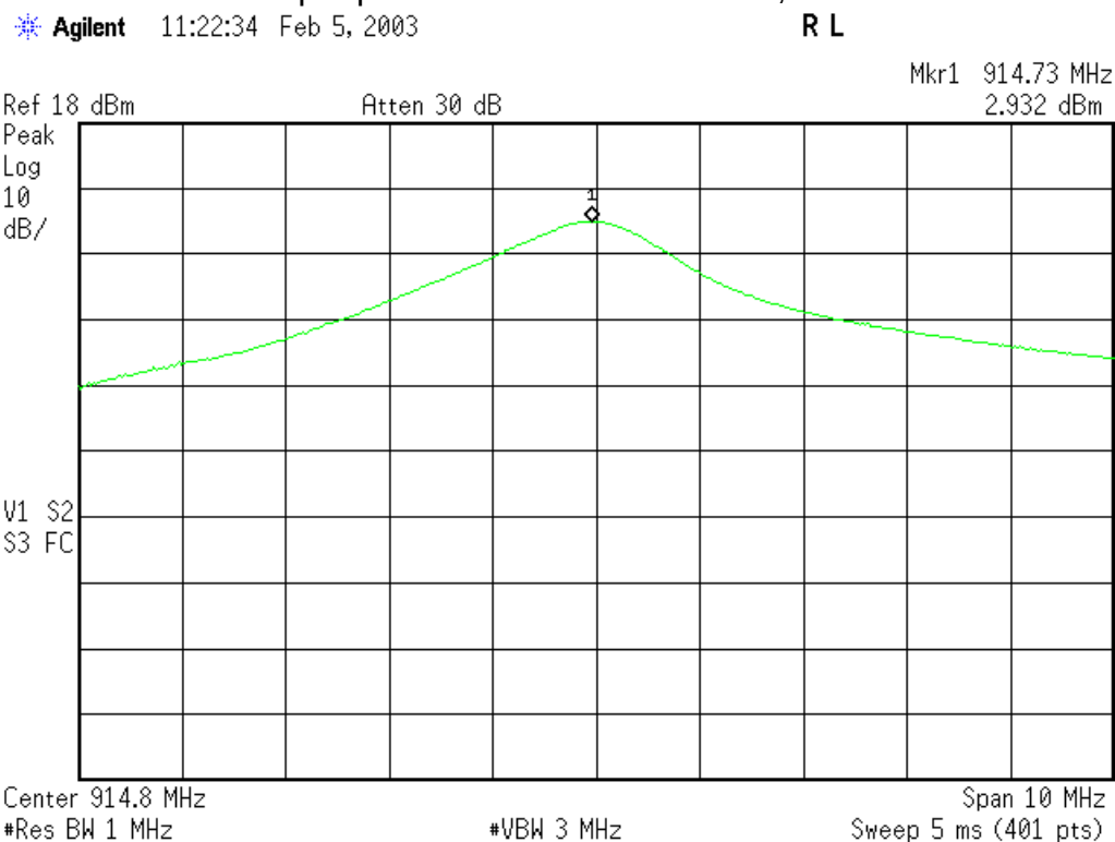
Peak output power UHF Antenna Port 1, Channel 24
