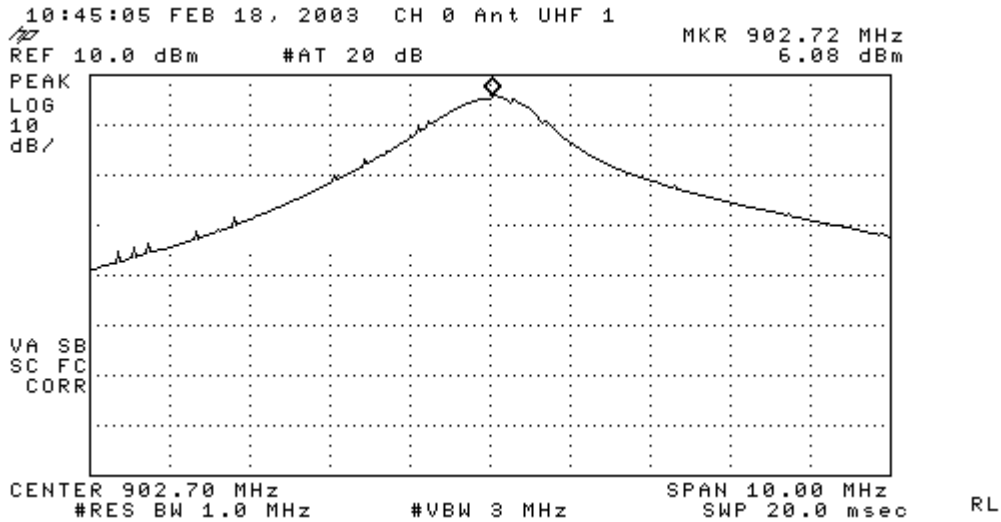
UHF Antenna Port 1, Channel 0
