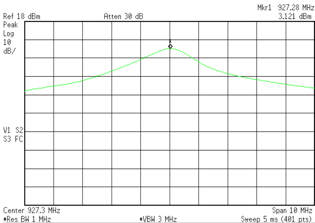
Peak output power UHF Antenna Port 1, Channel 49
