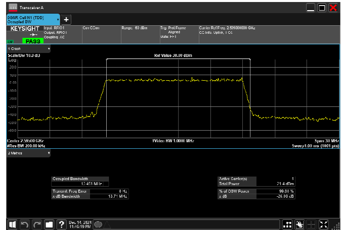
n38_15MHz_30kHz_2595MHz_CP-OFDM 16 QAM_RB38@0
