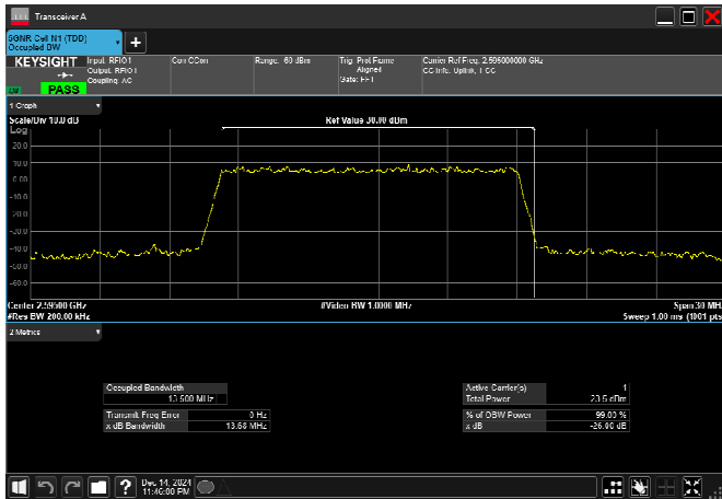
n38_15MHz_30kHz_2595MHz_CP-OFDM QPSK_RB38@0
