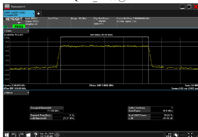
n38_25MHz_30kHz_2595MHz_CP-OFDM 256 QAM_RB65@0
