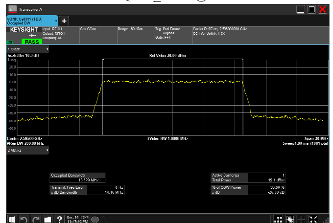
n38_15MHz_30kHz_2595MHz_CP-OFDM 256 QAM_RB38@0
