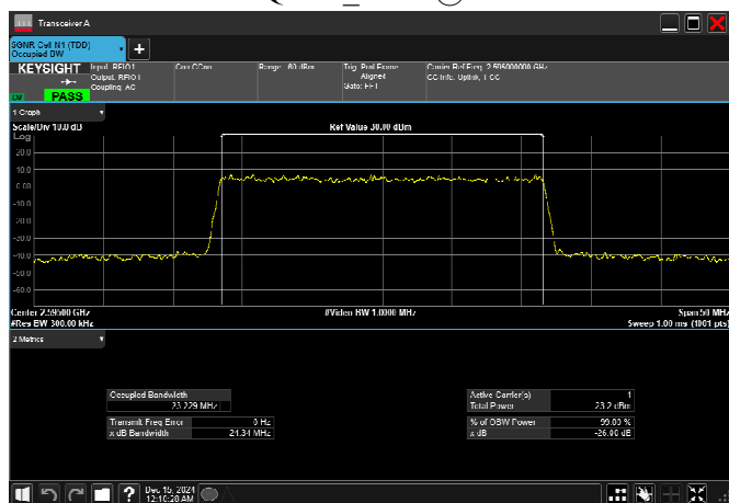
n38_25MHz_30kHz_2595MHz_CP-OFDM 64 QAM_RB65@0
