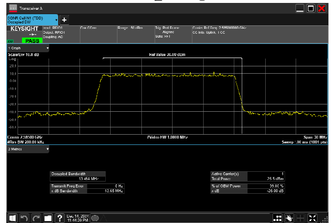
n38_15MHz_30kHz_2595MHz_DFT-s-OFDM 16 QAM_RB36@0
