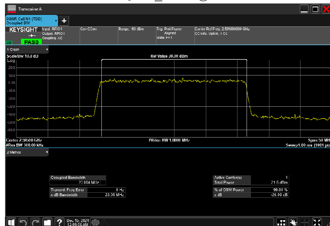
n38_25MHz_30kHz_2595MHz_CP-OFDM 16 QAM_RB65@0
