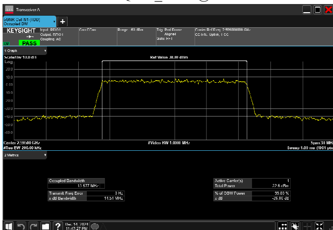
n38_15MHz_30kHz_2595MHz_CP-OFDM 64 QAM_RB38@0
