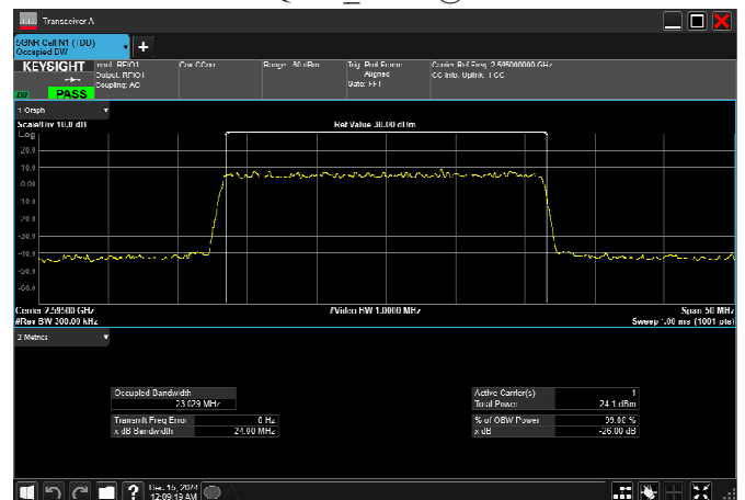
n38_25MHz_30kHz_2595MHz_DFT-s-OFDM 16 QAM_RB64@0
