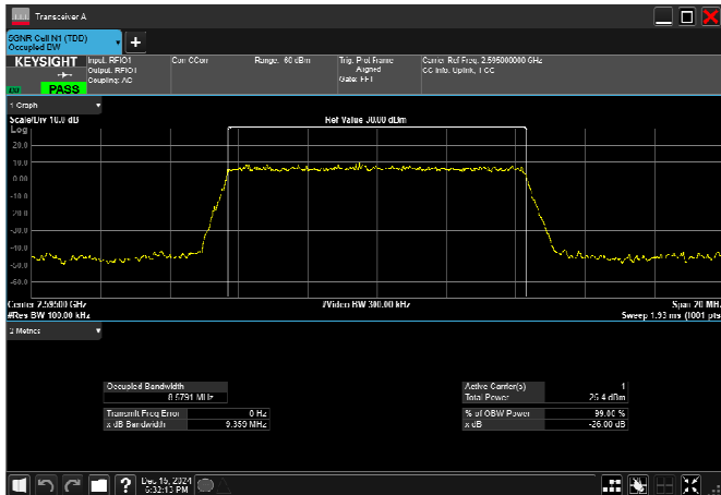
n38_10MHz_30kHz_2595MHz_DFT-s-OFDM 16 QAM_RB24@0
