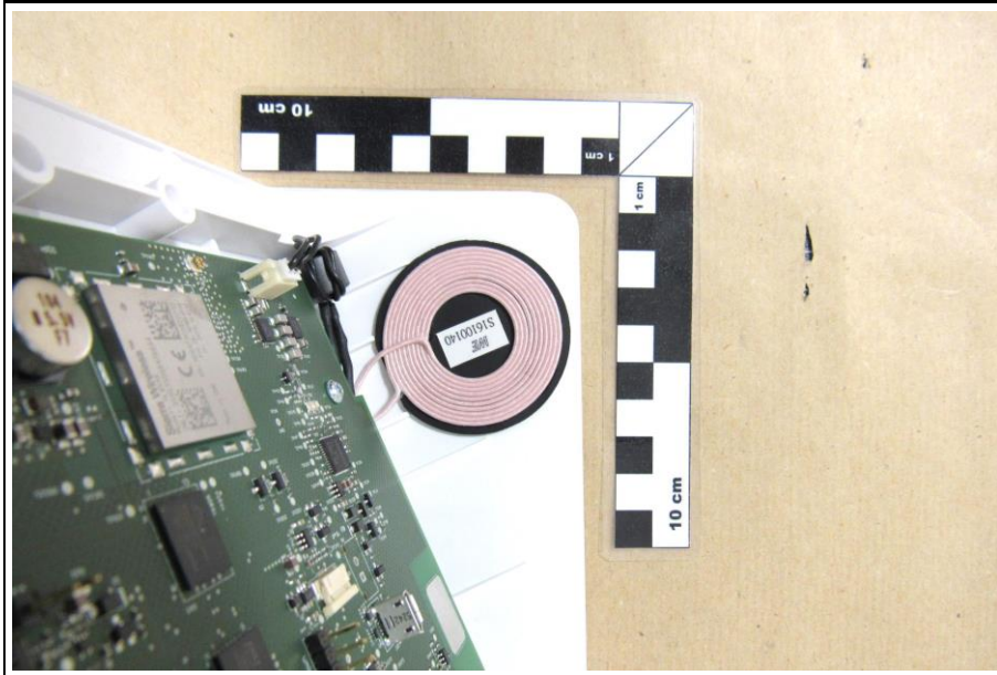
Loop antenna
