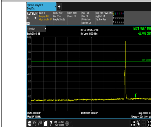
Band13_10MHz_QPSK_23230_1RB#49_30~1000_30~1000
