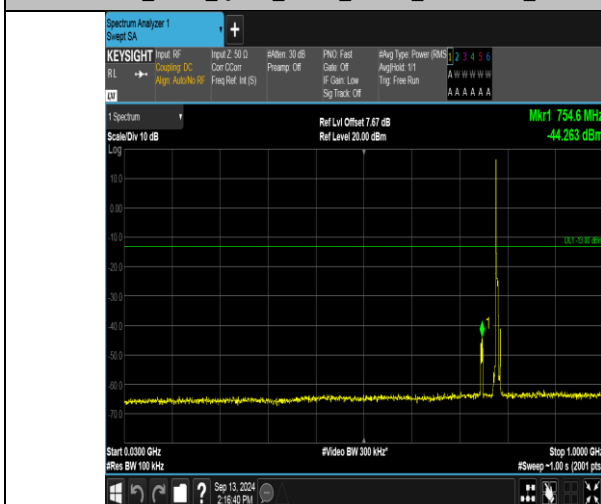
Band13_5MHz_QPSK_23255_1RB#0_30~1000_30~1000
