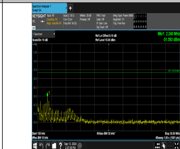
Band13_10MHz_QPSK_23230_50RB#0_0.15~30_0.15~30
