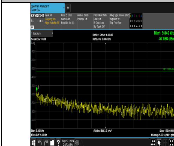
Band13_10MHz_QPSK_23230_50RB#0_0.009~0.15_0.009~0.15
