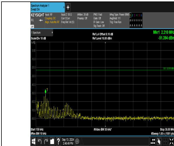
Band13_10MHz_16QAM_23230_1RB#49_0.15~30_0.15~30
