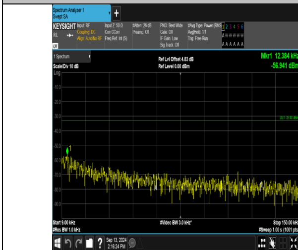
Band13_5MHz_QPSK_23255_1RB#0_0.009~0.15_0.009~0.15
