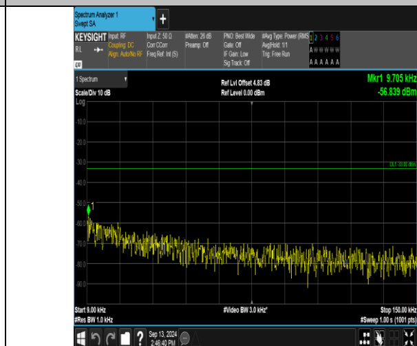
Band13_10MHz_16QAM_23230_1RB#49_0.009~0.15_0.009~0.15
