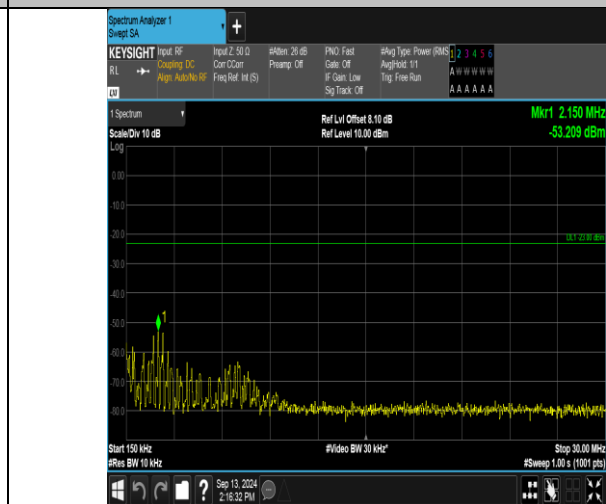
Band13_5MHz_QPSK_23255_1RB#0_0.15~30_0.15~30
