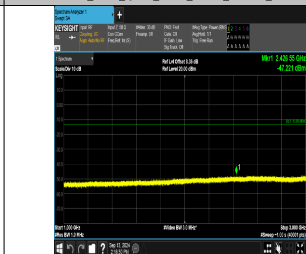
Band13_5MHz_QPSK_23255_1RB#0_1000~3000_1000~3000
