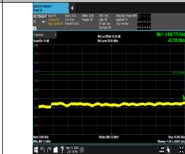
Band13_10MHz_16QAM_23230_1RB#49_3000~10000_3000~10000
