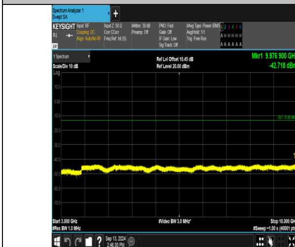
Band13_10MHz_QPSK_23230_1RB#49_3000~10000_3000~10000
