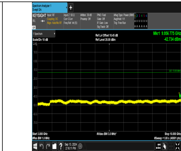
Band13_5MHz_16QAM_23230_25RB#0_3000~10000_3000~10000
