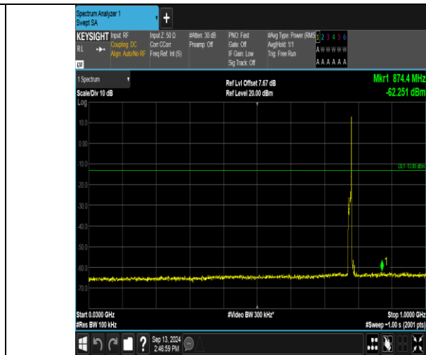
Band13_10MHz_16QAM_23230_1RB#49_30~1000_30~1000
