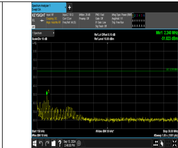
Band13_10MHz_QPSK_23230_1RB#49_0.15~30_0.15~30
