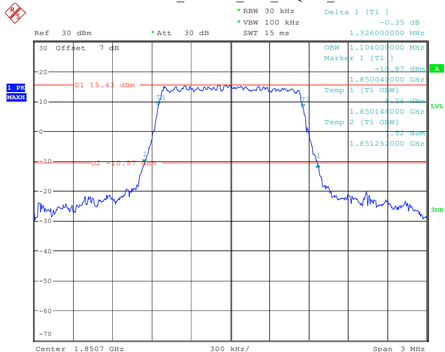
Band 2_1.4 MHz_Low_16QAM_RB6#0
