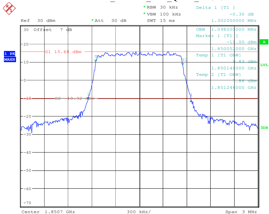
Band 2_1.4 MHz_Low_QPSK_RB6#0
