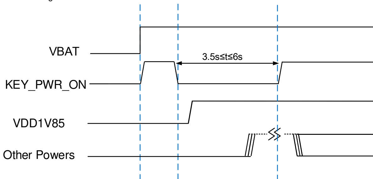
Figure 3-6 Power on timing
