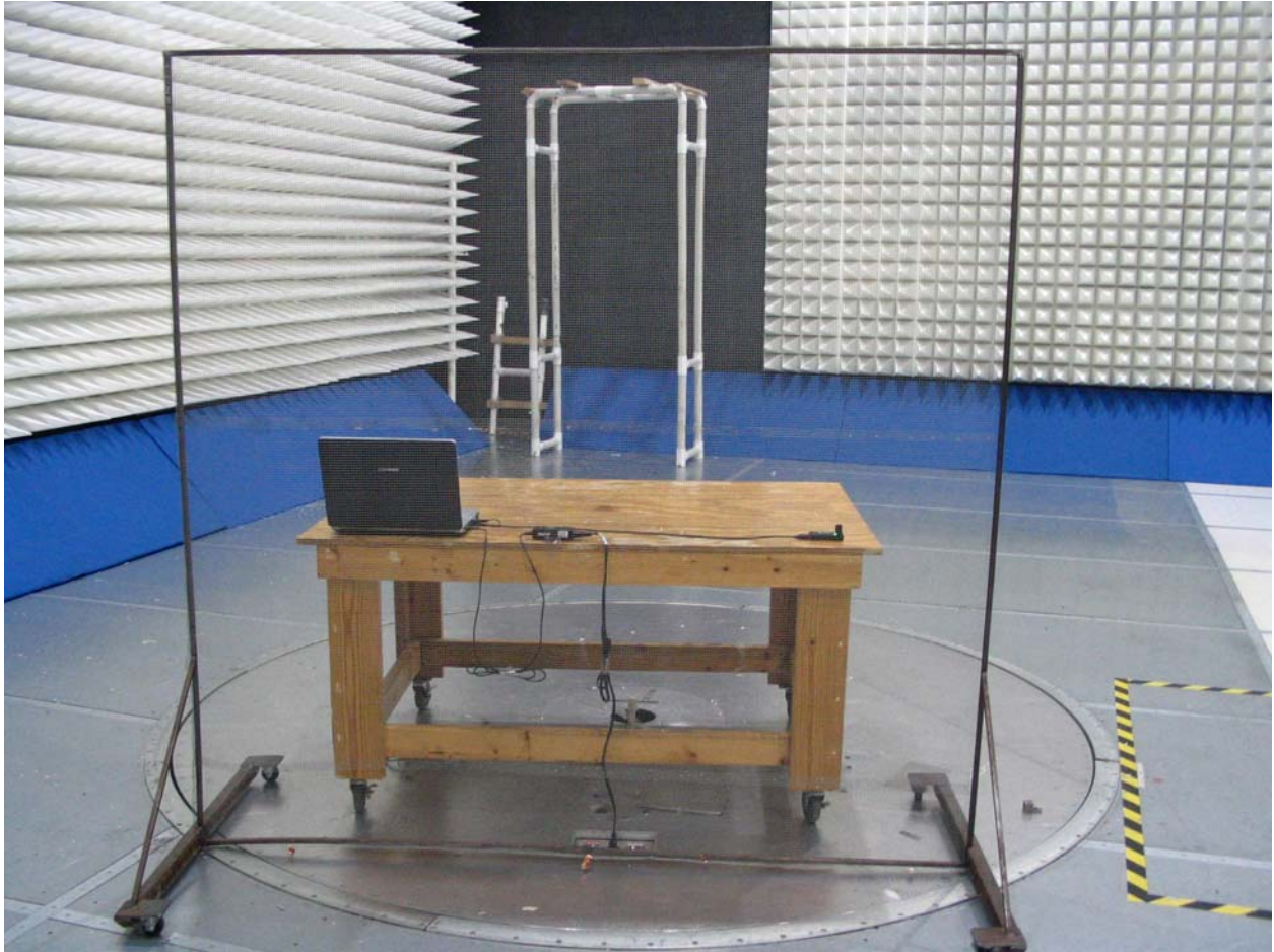
Figure 4: Conducted Voltage Emissions (Back)
