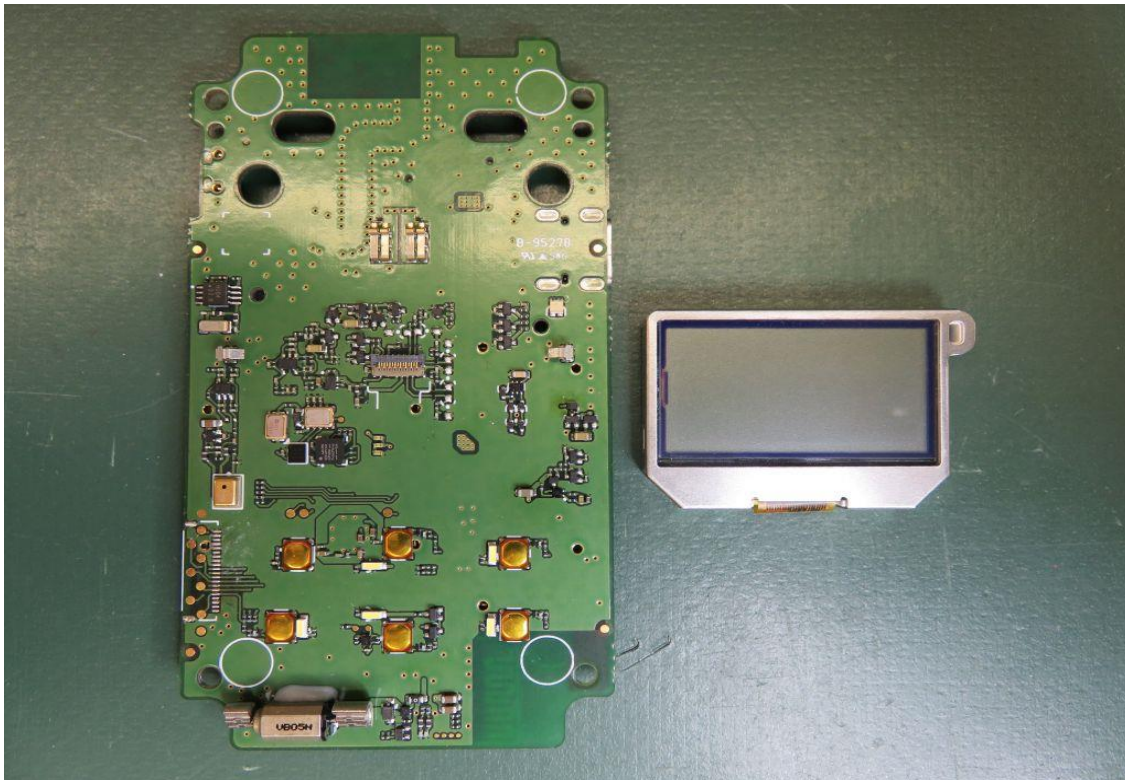
Main Board (side-A) view
