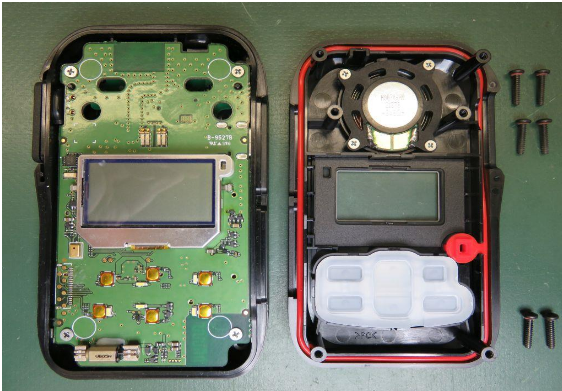
Main Board view in chassis
