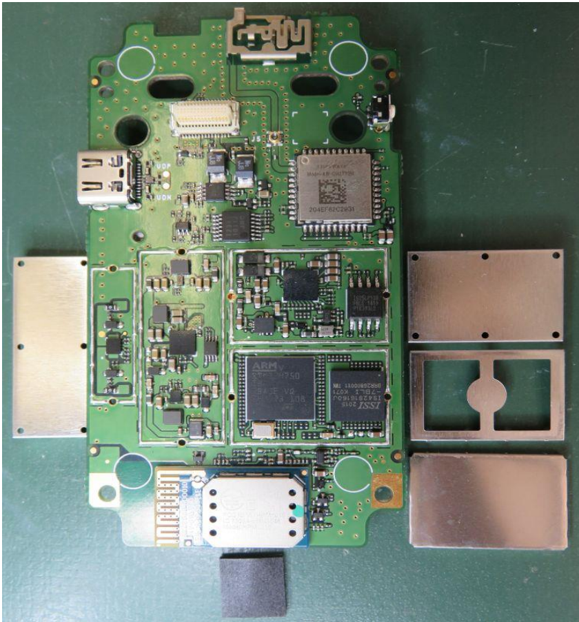
Main Board (side-B) view
