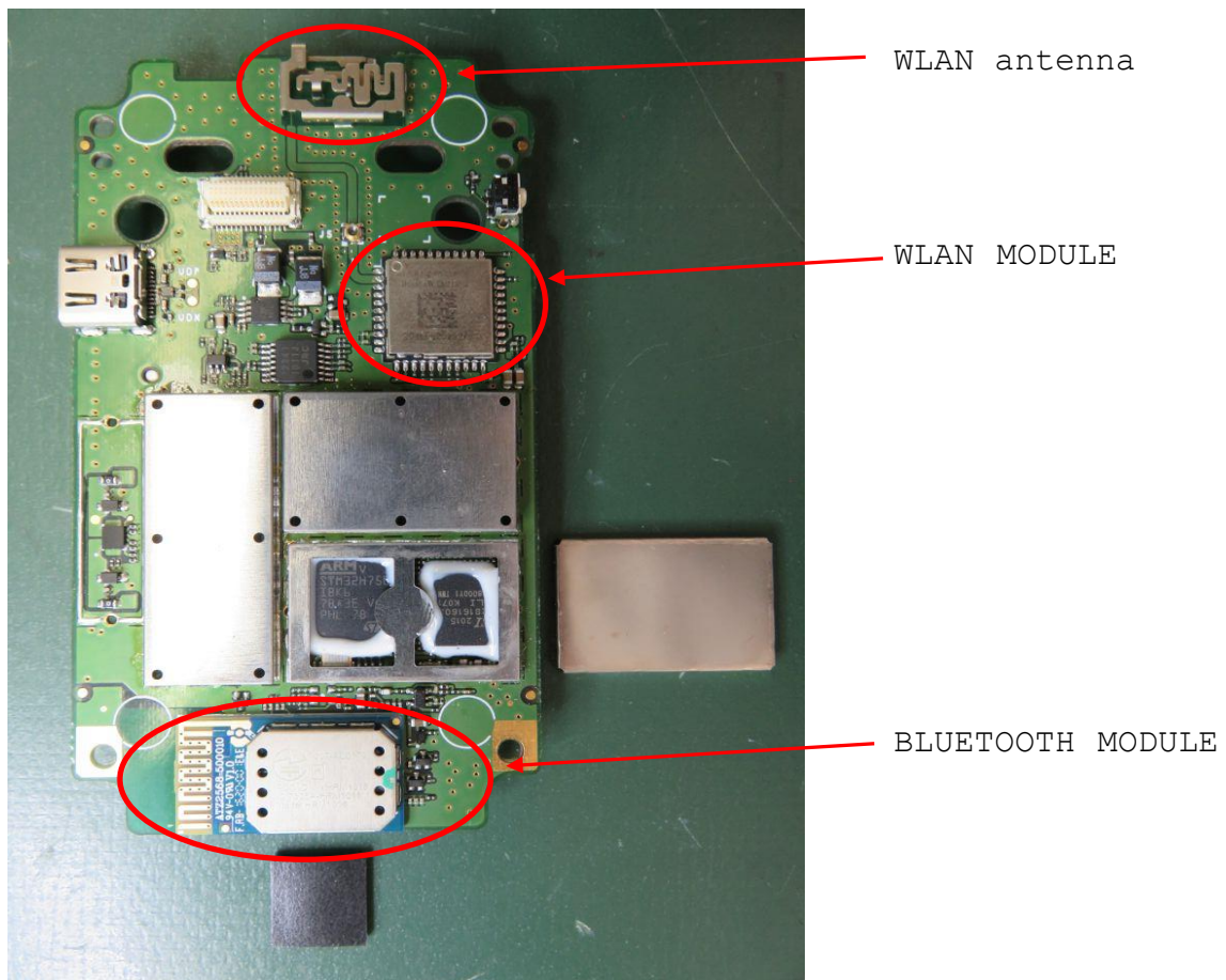
Main Board (side-B) view
