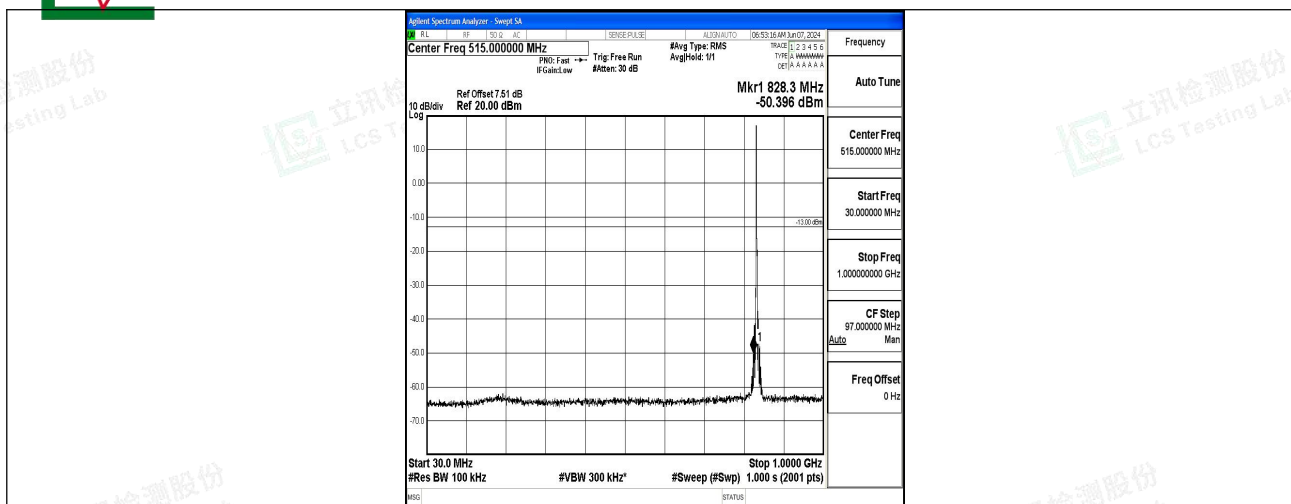
Band5_3MHz_QPSK_20525_1RB#0_30~1000_30~1000
