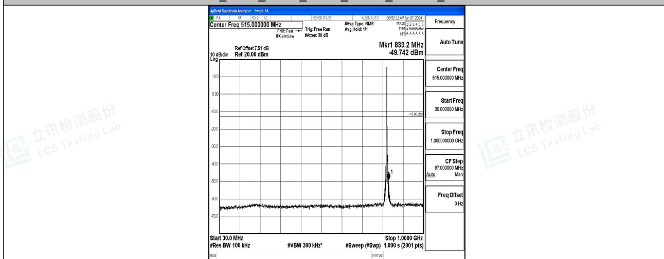
Band5_3MHz_QPSK_20415_1RB#0_30~1000_30~1000
