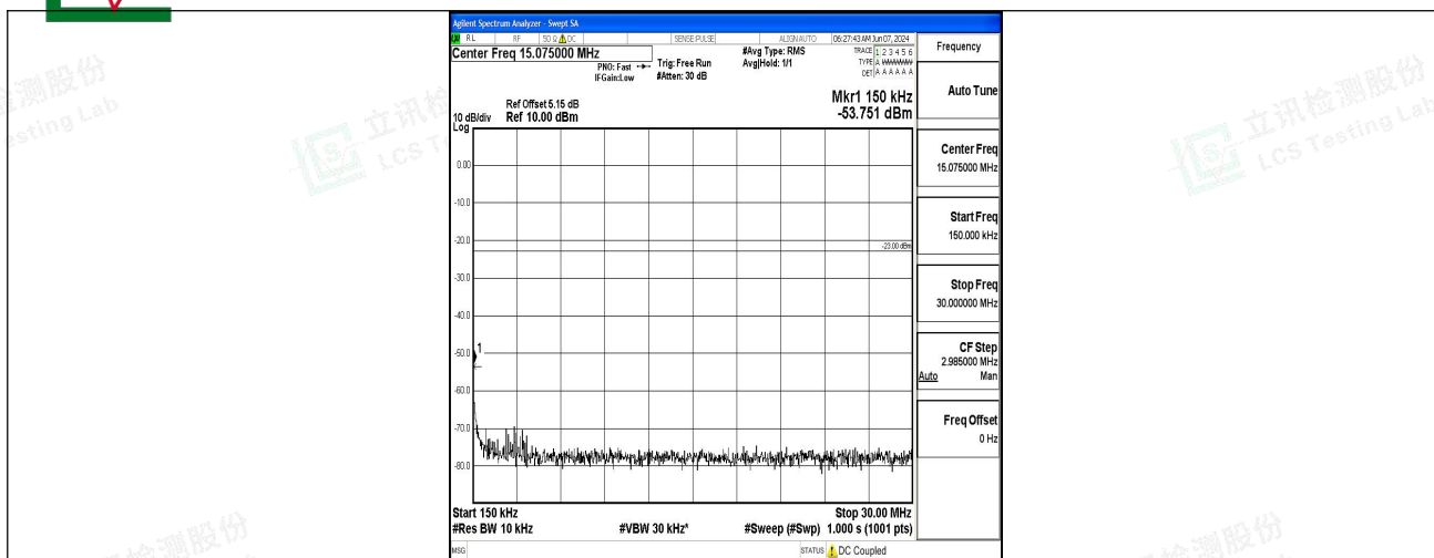
Band5_1.4MHz_16QAM_20407_1RB#0_0.15~30_0.15~30
