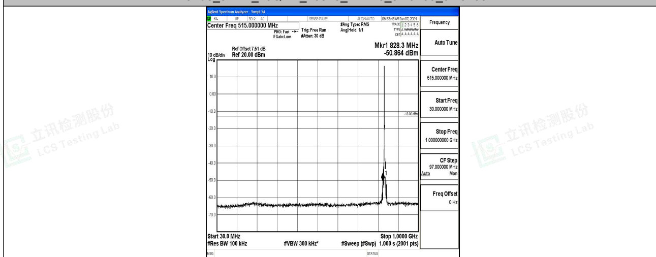
Band5_3MHz_16QAM_20525_1RB#0_30~1000_30~1000
