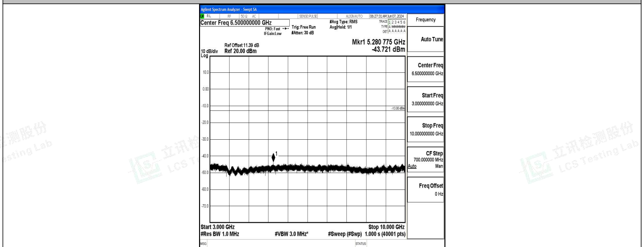
Band5_1.4MHz_QPSK_20407_1RB#0_3000~10000_3000~10000
