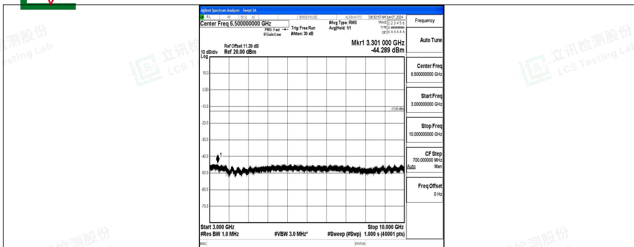
Band5_3MHz_16QAM_20415_1RB#0_3000~10000_3000~10000
