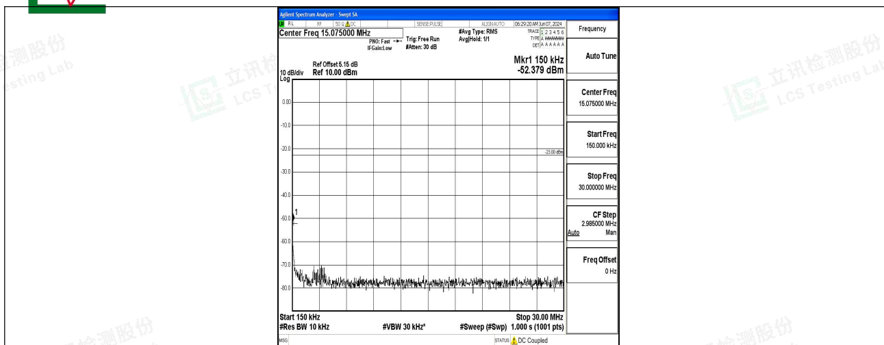
Band5_1.4MHz_QPSK_20643_1RB#0_0.15~30_0.15~30
