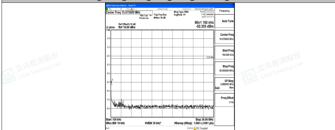
Band5_1.4MHz_16QAM_20643_1RB#0_0.15~30_0.15~30
