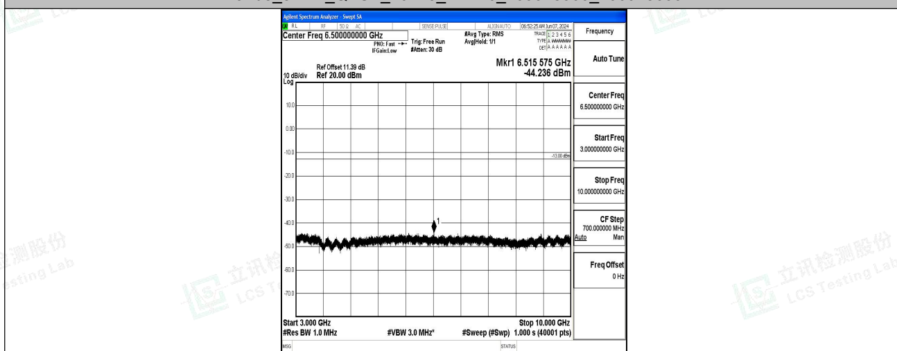
Band5_3MHz_QPSK_20415_1RB#0_3000~10000_3000~10000
