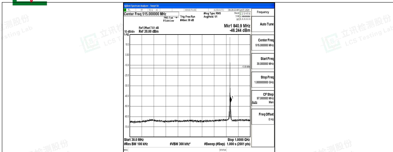
Band5_1.4MHz_QPSK_20525_1RB#0_30~1000_30~1000
