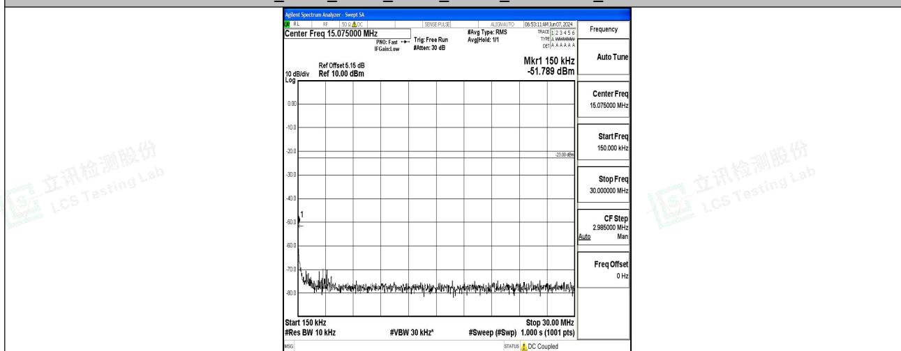
Band5_3MHz_QPSK_20525_1RB#0_0.15~30_0.15~30
