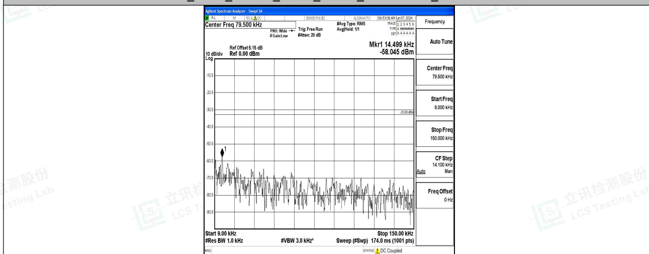
Band5_3MHz_QPSK_20525_1RB#0_0.009~0.15_0.009~0.15
