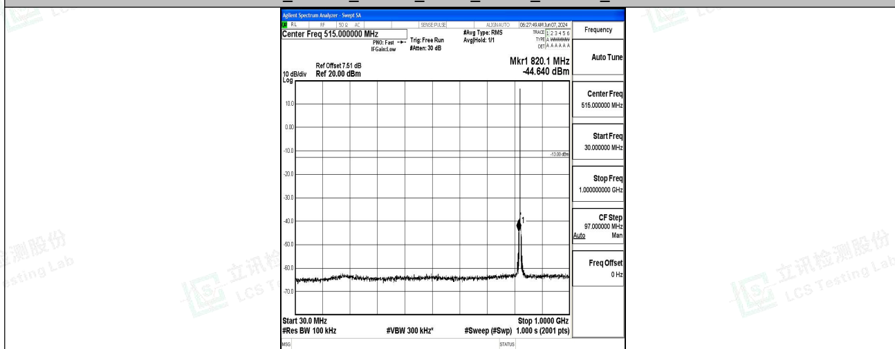
Band5_1.4MHz_16QAM_20407_1RB#0_30~1000_30~1000
