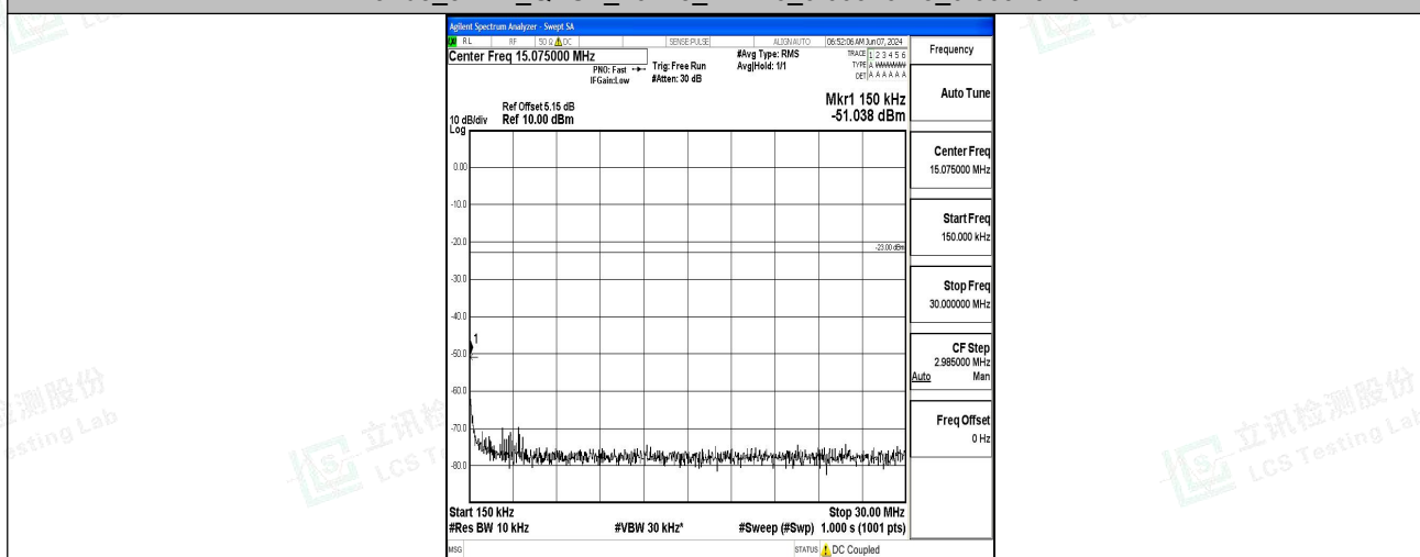
Band5_3MHz_QPSK_20415_1RB#0_0.15~30_0.15~30
