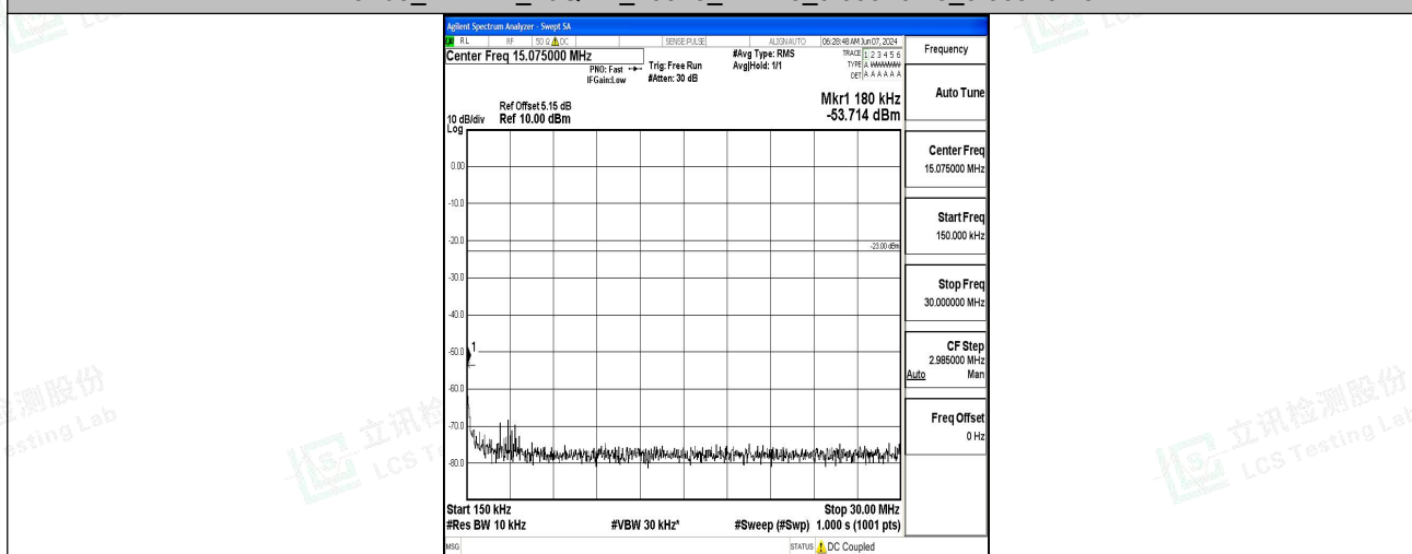
Band5_1.4MHz_16QAM_20525_1RB#0_0.15~30_0.15~30
