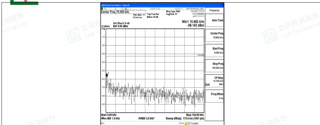
Band5_3MHz_16QAM_20525_1RB#0_0.009~0.15_0.009~0.15
