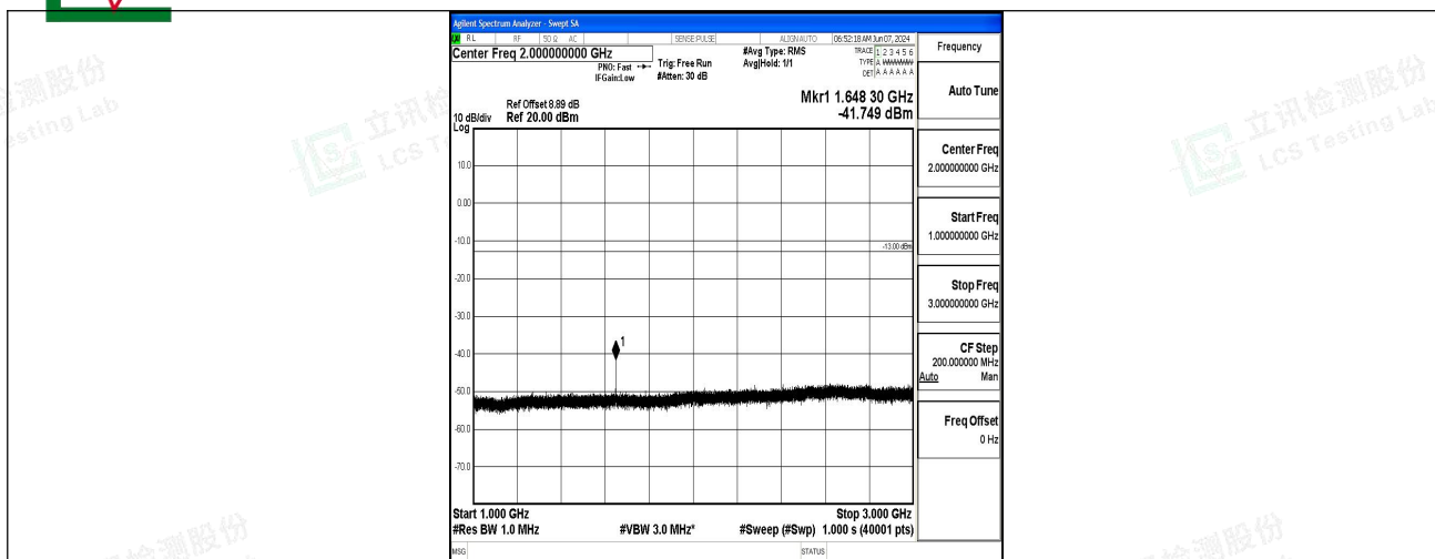
Band5_3MHz_QPSK_20415_1RB#0_1000~3000_1000~3000
