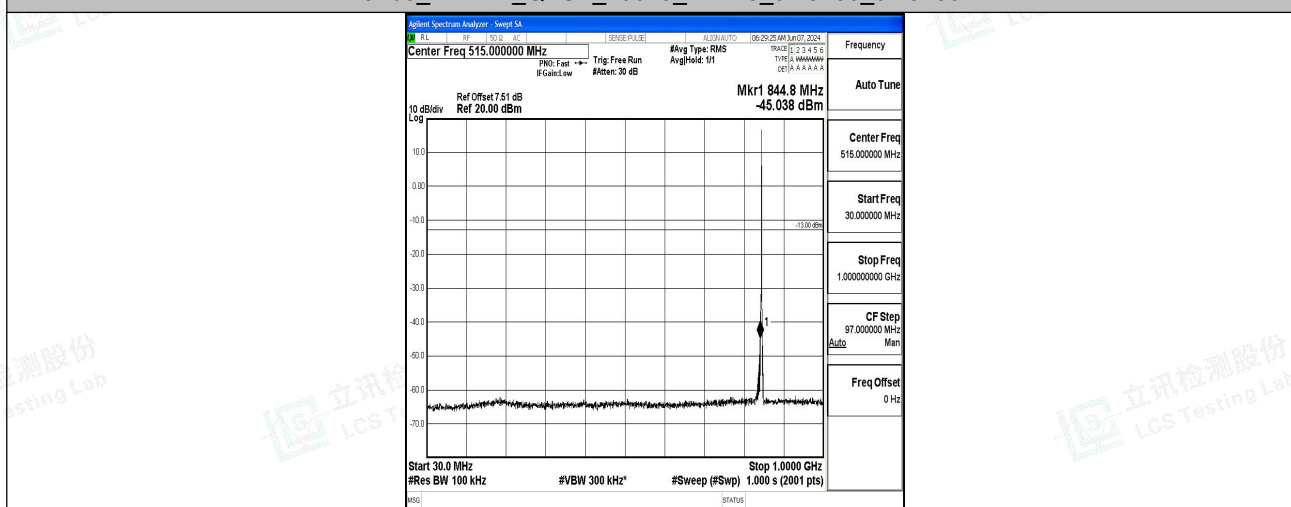
Band5_1.4MHz_QPSK_20643_1RB#0_30~1000_30~1000
