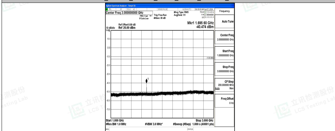
Band5_1.4MHz_16QAM_20643_1RB#0_1000~3000_1000~3000
