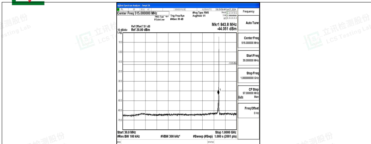
Band5_1.4MHz_16QAM_20643_1RB#0_30~1000_30~1000
