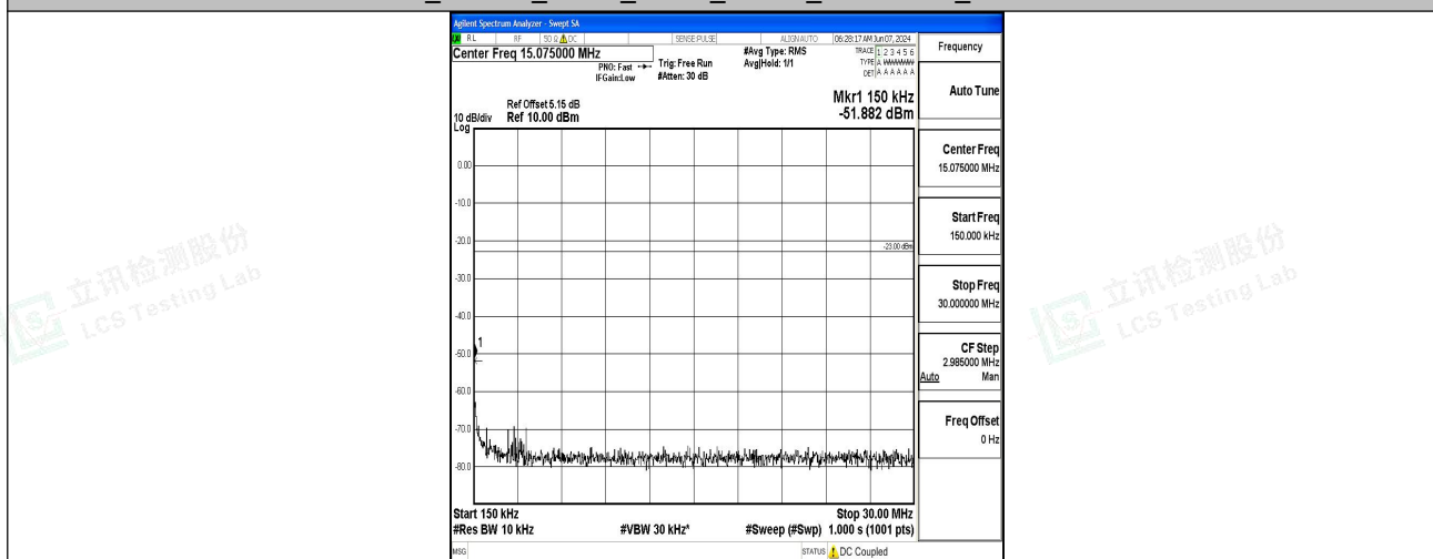
Band5_1.4MHz_QPSK_20525_1RB#0_0.15~30_0.15~30
