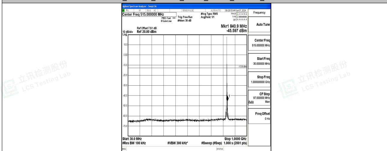
Band5_1.4MHz_16QAM_20525_1RB#0_30~1000_30~1000
