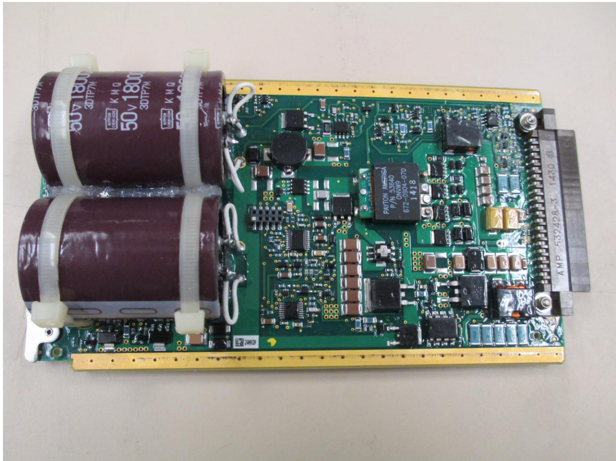
Power_supply_top
