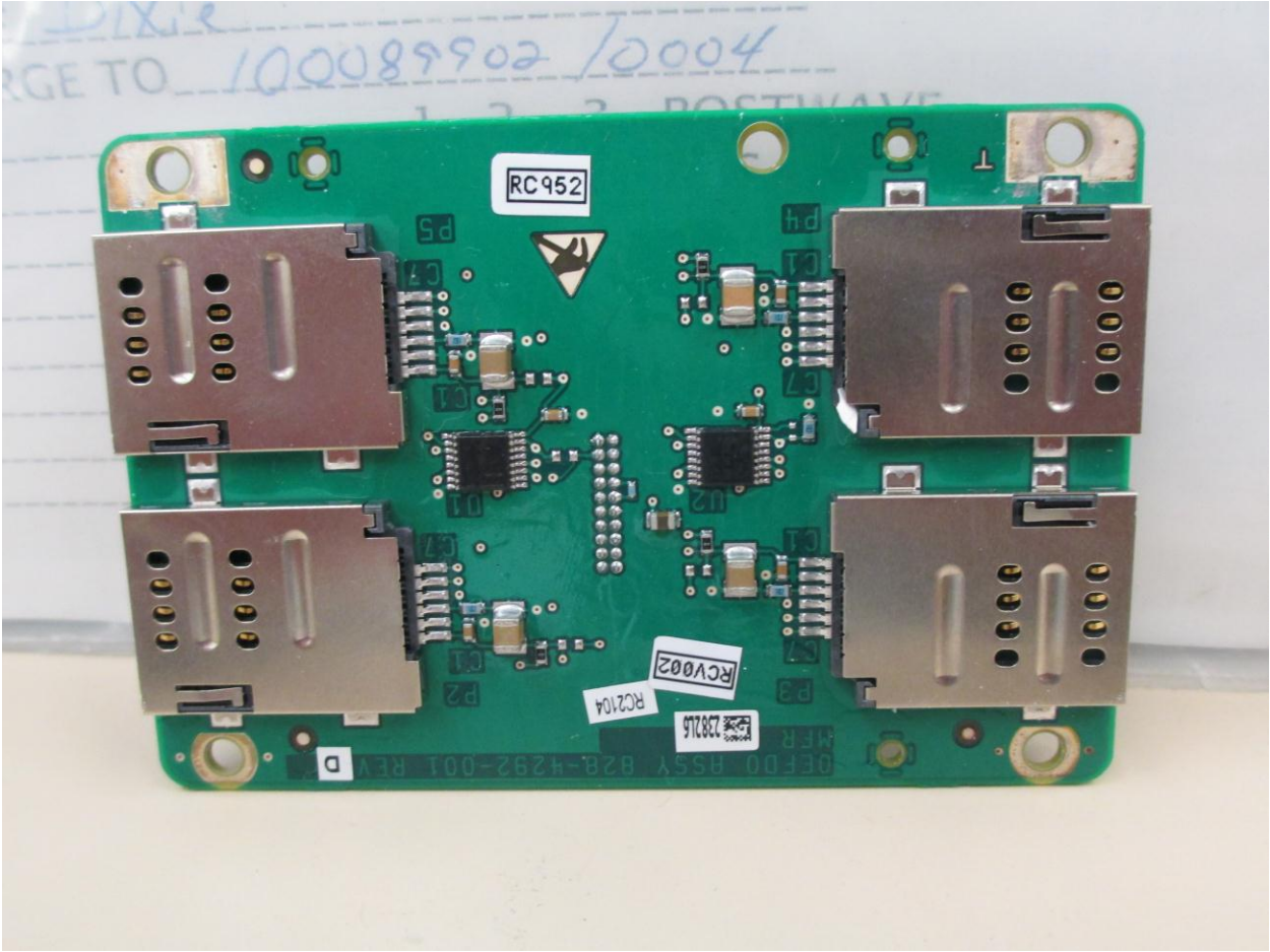
SIM_Card_top
