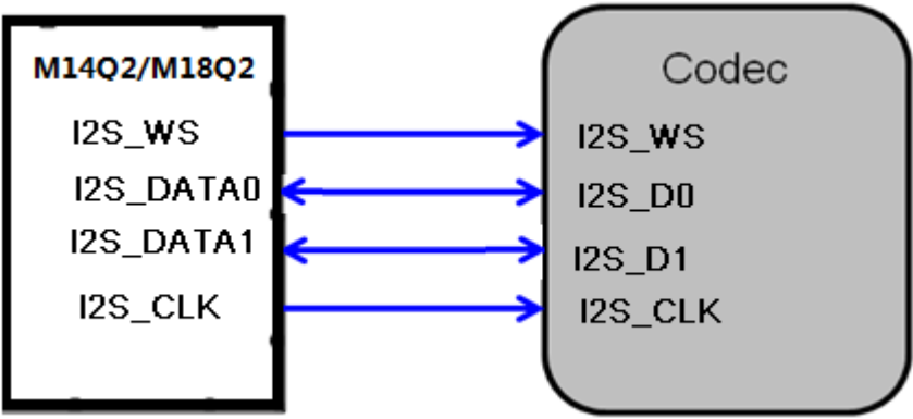
Figure 8. I2S connection (example)
