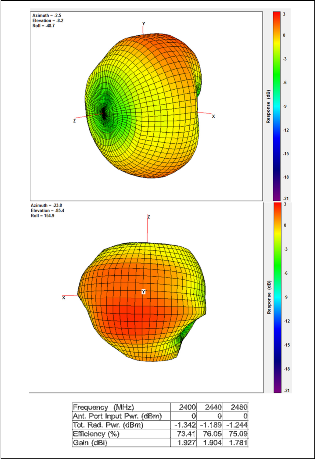
FIGURE 1-1: BM62 ANTENNA RADIATION PATTERN
