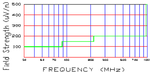
Figure B-8. Radiated limits at 3 meters.
