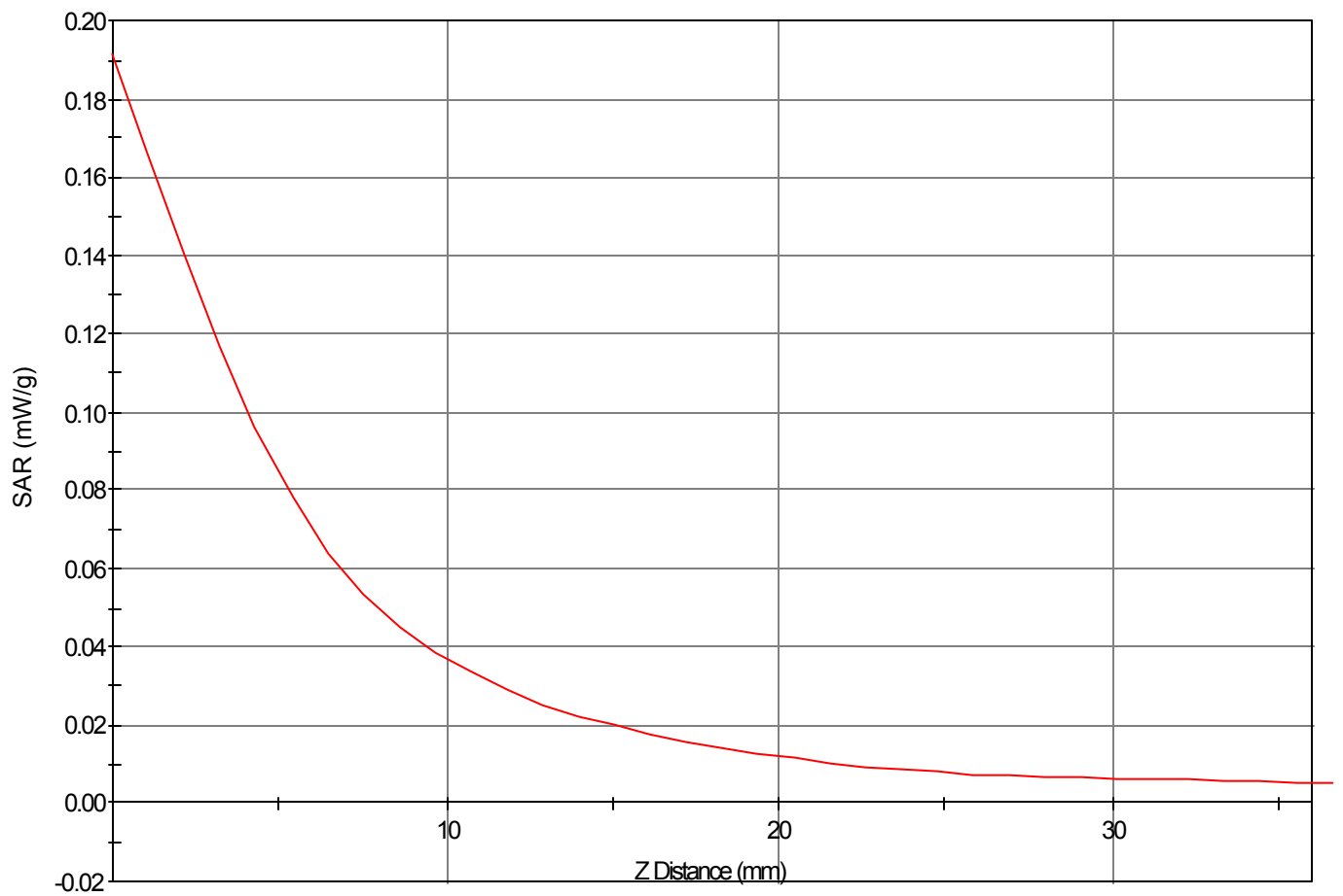
SAR - Z Axis at Hotspot x:-18.0 y:5.0
