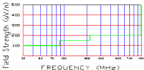
Figure B-1. Radiated limits at 3 meters.
