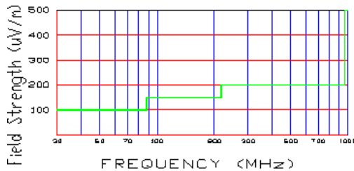
Figure B-7. Radiated limits at 3 meters.
