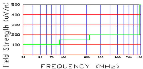
Figure B-2. Radiated limits at 3 meters.
