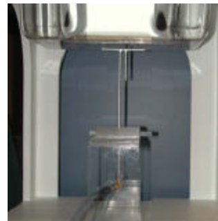
Figure A.0 Dipole Validation Test Setup
