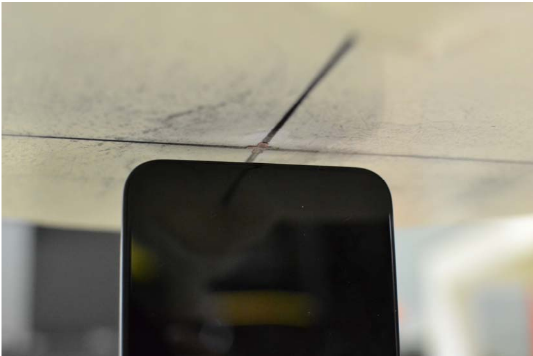
SAR Test Setup Photo 16 – Bottom Edge at 4 mm
