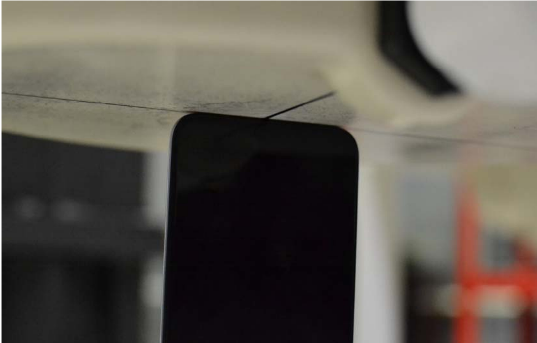
SAR Test Setup Photo 17 – Bottom Edge at 0 mm
