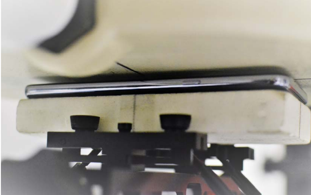
SAR Test Setup Photo 13 – Front Side at 3 mm
