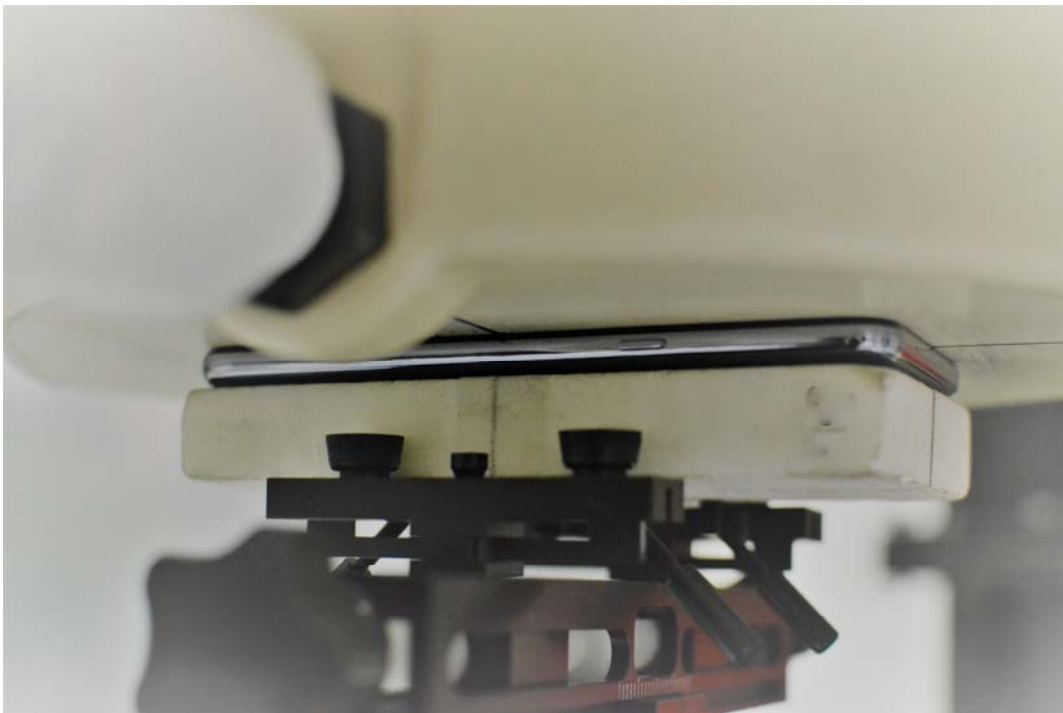
SAR Test Setup Photo 14 – Front Side at 0 mm
