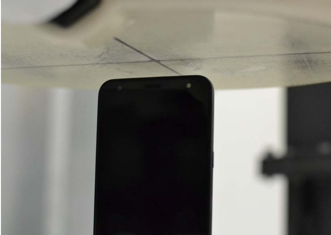
SAR Test Setup Photo 7 –Top Edge at 10 mm
