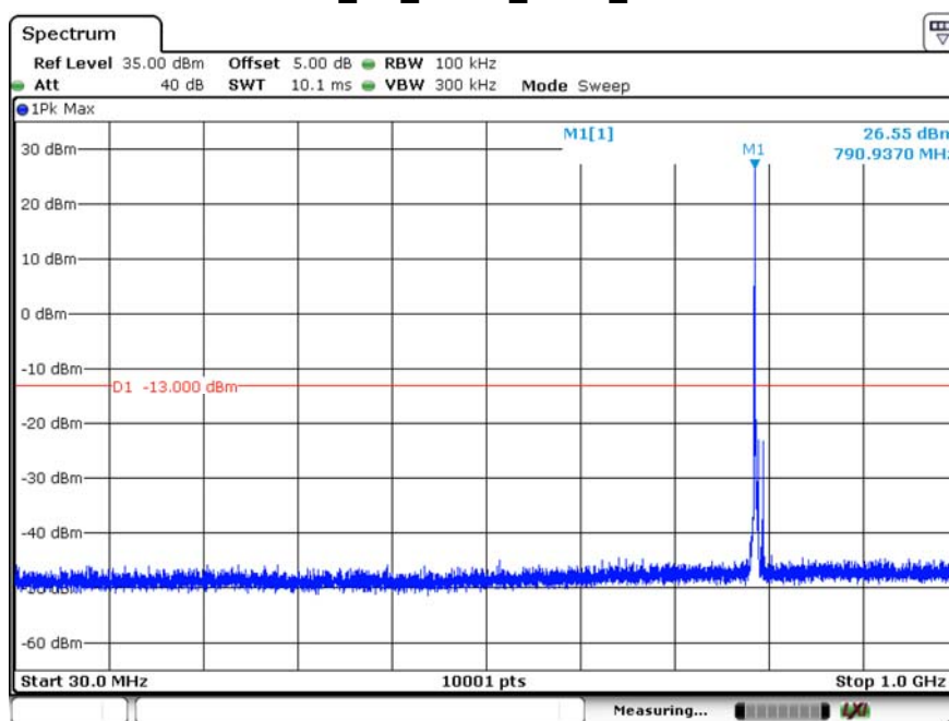
CH23330_5M_QPSK_1RB0_under 1G
