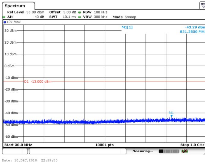
CH18900_1.4M_QPSK_1RB0_under 1G
