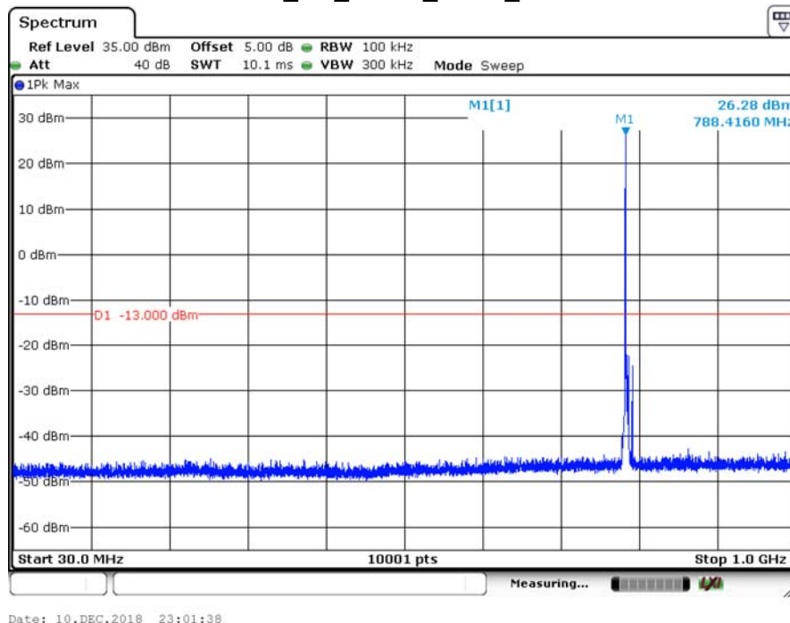
CH23305_5M_QPSK_1RB0_under 1G
