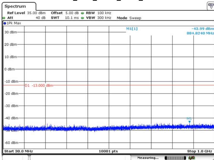
CH18900_1.4M_QPSK_1RB0_under 1G
