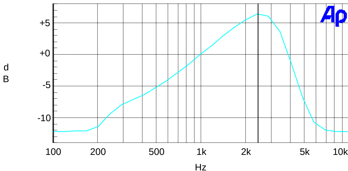
1380AUT4 Audio Frequency Response Plot
