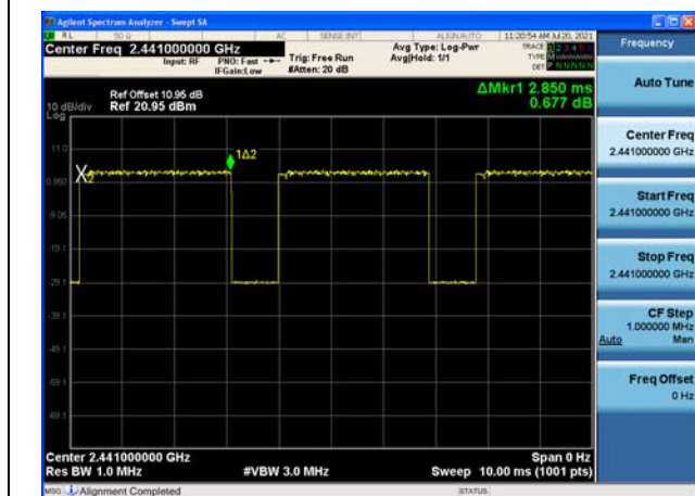
Modulation: 8DPSK 3DH5 2441
