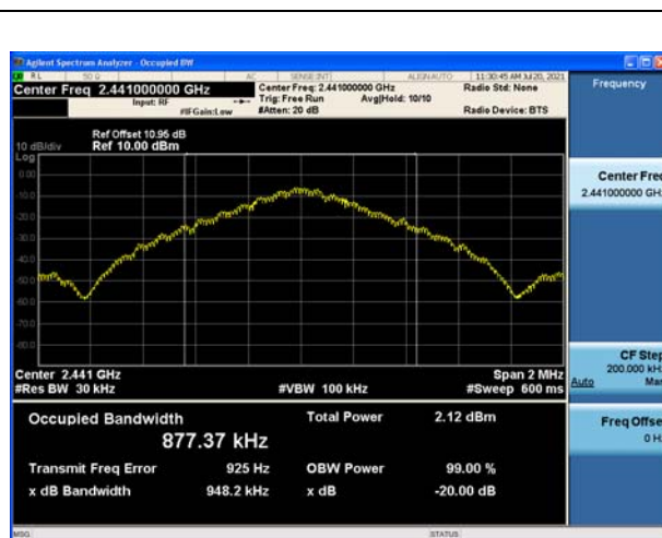
Modulation: GFSK 2441MHz
