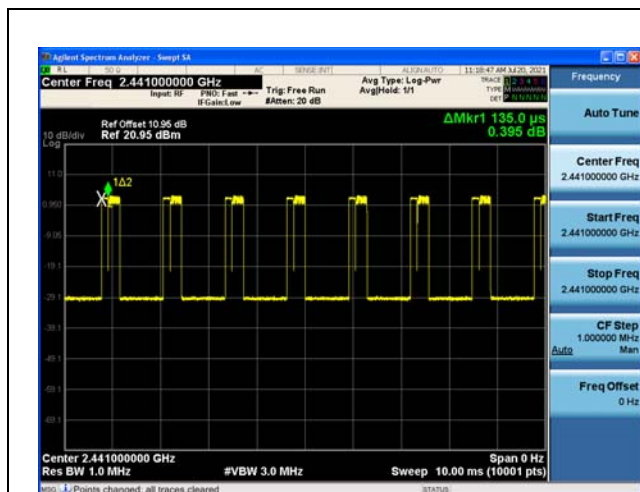
Modulation: \pi/4 DQPSK 2DH1 2441
