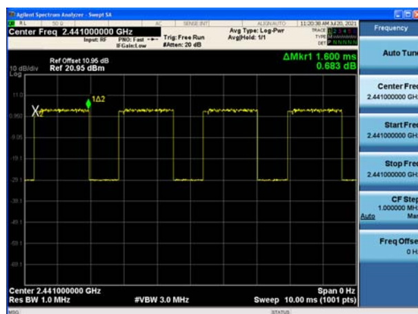
Modulation: 8DPSK 3DH3 2441
