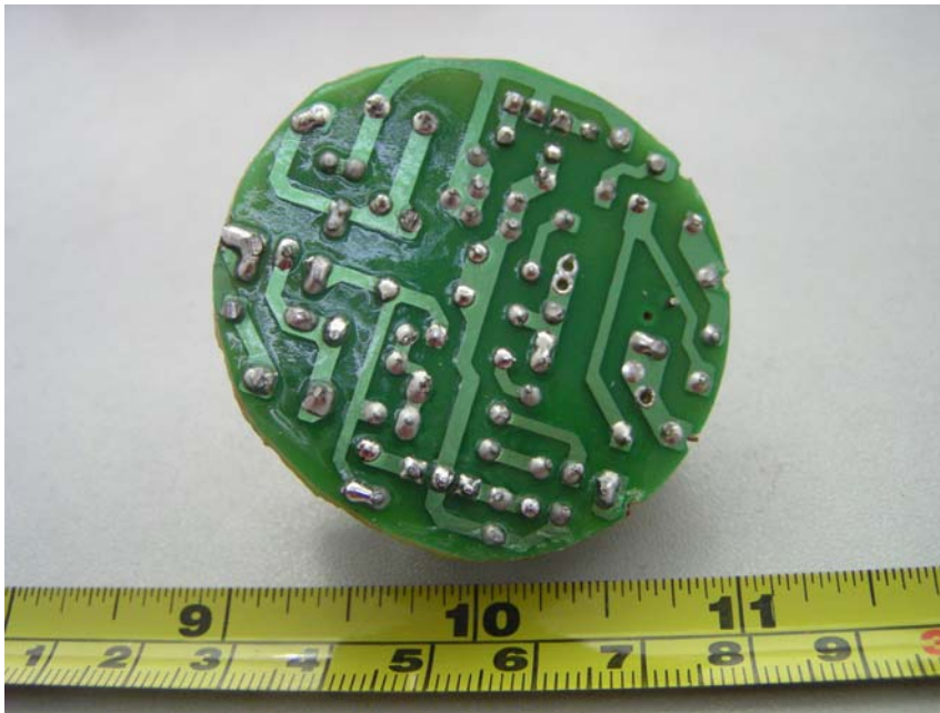
SL25B-120: EUT - Uncovered View
