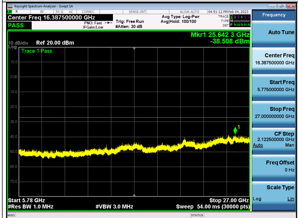
Test_Graph_802.11ax80_ANT2_5530_MCS9_Frequency Band 4
