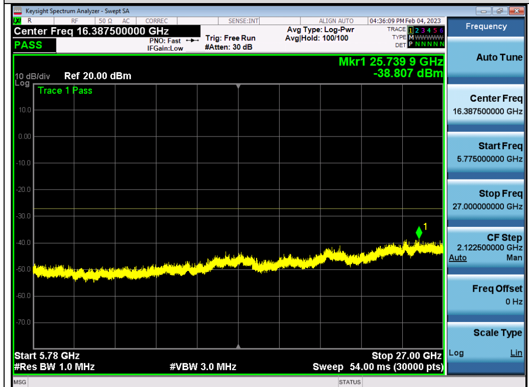
Test_Graph_802.11ac80_ANT2_5530_MCS9_Frequency Band 4
