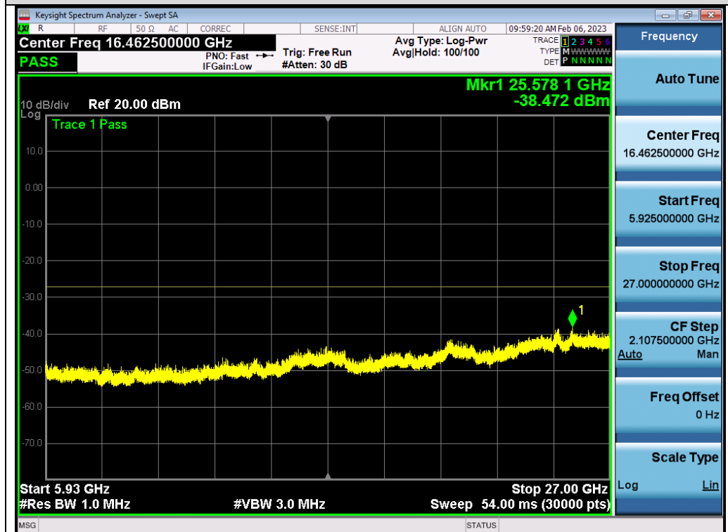
Test_Graph_802.11ax80_ANT2_5775_MCS0_Frequency Band4
