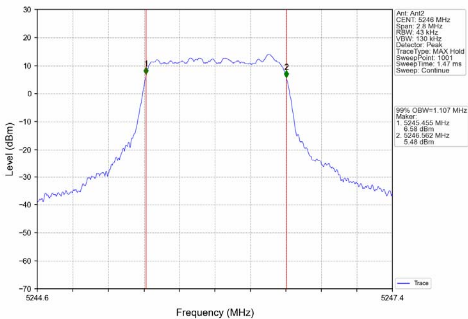
16QAM 1.4MHz_HCH_5246MHz_Ant2_NTNV
