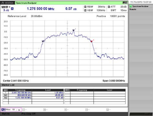
[EDR / 2441 MHz]
