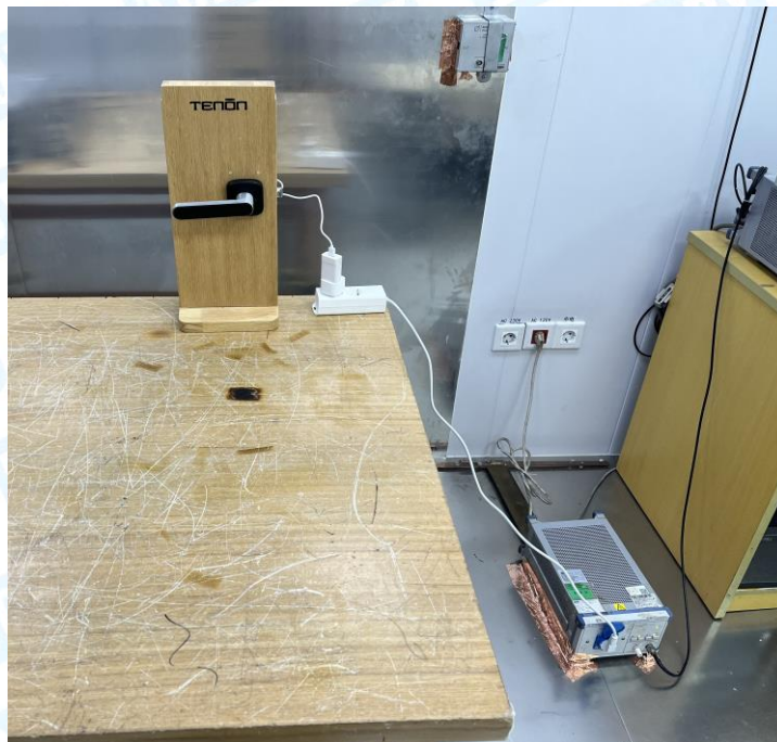
Photo of Setup for Conducted Emission
