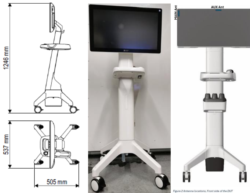
Figure 2 Antenna locations, Front side of the DUT
