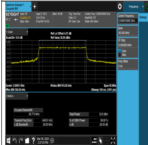
NTNV-N78-3450-3550-PC2-30-30-M-DFT-QPSK- Outer_Full-Ant7-PASS
