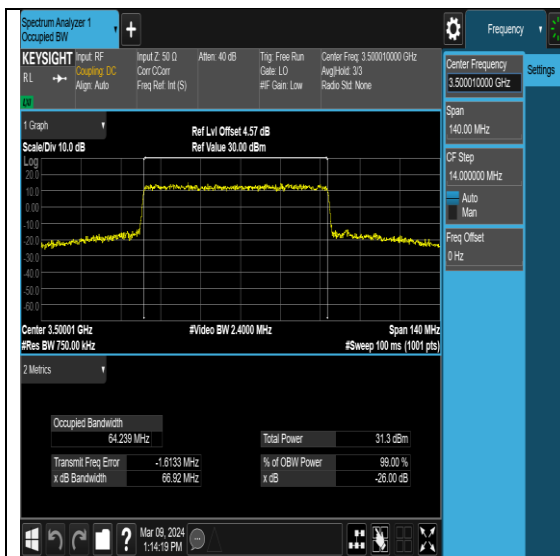
NTNV-N78-3450-3550-PC2-30-70-M-DFT- 64QAM-Outer_Full-Ant7-PASS
