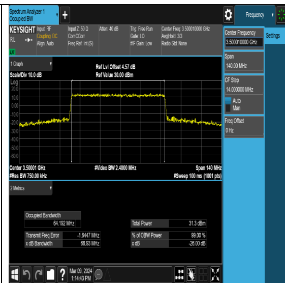
NTNV-N78-3450-3550-PC2-30-70-M-DFT- 256QAM-Outer_Full-Ant7-PASS
