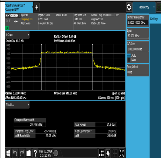
NTNV-N78-3450-3550-PC2-30-30-M-DFT- 16QAM-Outer_Full-Ant7-PASS
