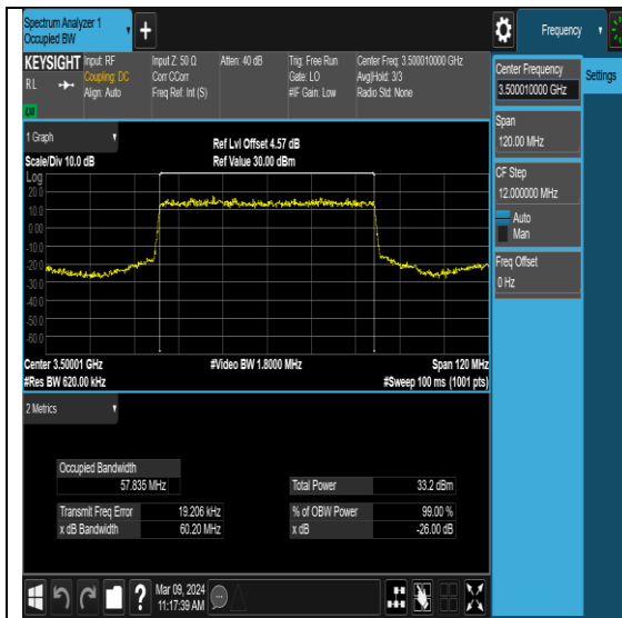
NTNV-N78-3450-3550-PC2-30-60-M-DFT- P12BPSK-Outer_Full-Ant7-PASS
