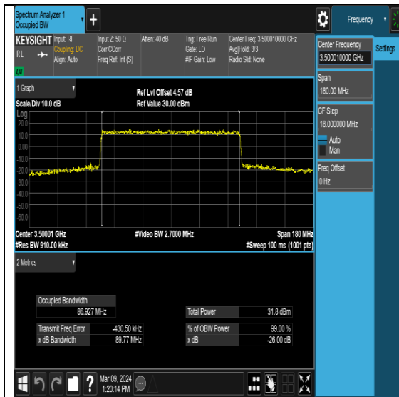
NTNV-N78-3450-3550-PC2-30-90-M-DFT- 16QAM-Outer_Full-Ant7-PASS
