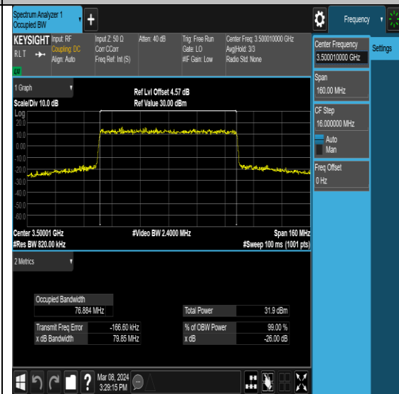
NTNV-N78-3450-3550-PC2-30-80-M-DFT- 16QAM-Outer_Full-Ant7-PASS
