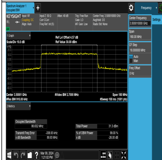
NTNV-N78-3450-3550-PC2-30-90-M-DFT- 256QAM-Outer_Full-Ant7-PASS
