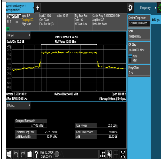
NTNV-N78-3450-3550-PC2-30-80-M-DFT-QPSK- Outer_Full-Ant7-PASS
