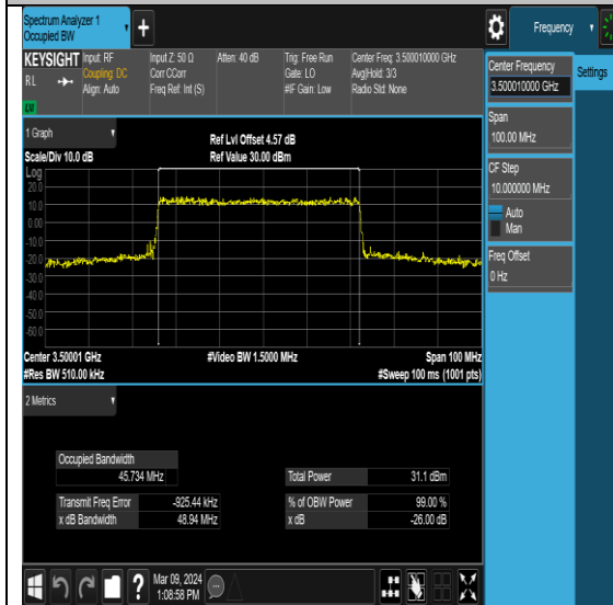
NTNV-N78-3450-3550-PC2-30-50-M-DFT- 64QAM-Outer_Full-Ant7-PASS
