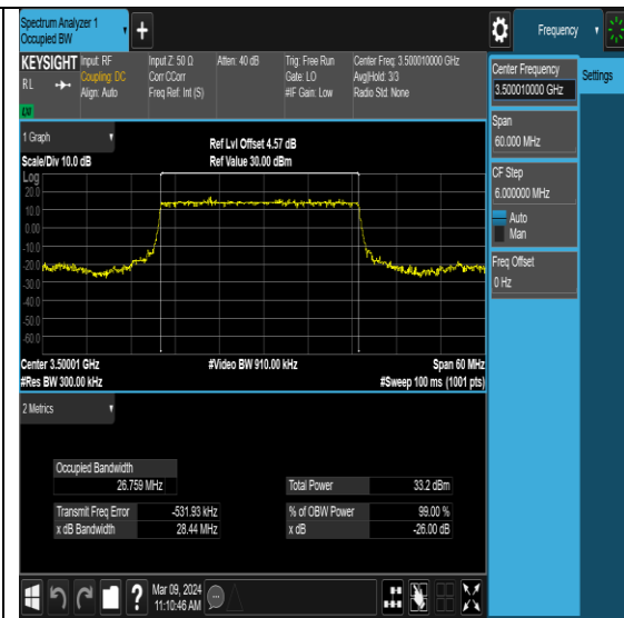
NTNV-N78-3450-3550-PC2-30-30-M-DFT- PI2BPSK-Outer_Full-Ant7-PASS
