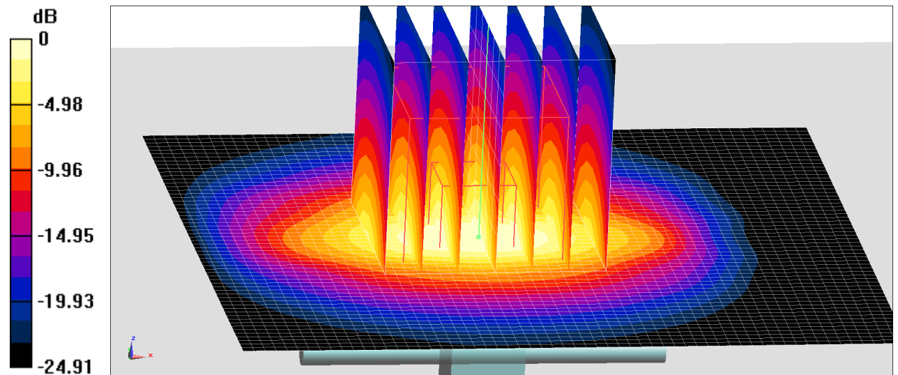
Fig.B.9 validation 2600MHz 250mW
