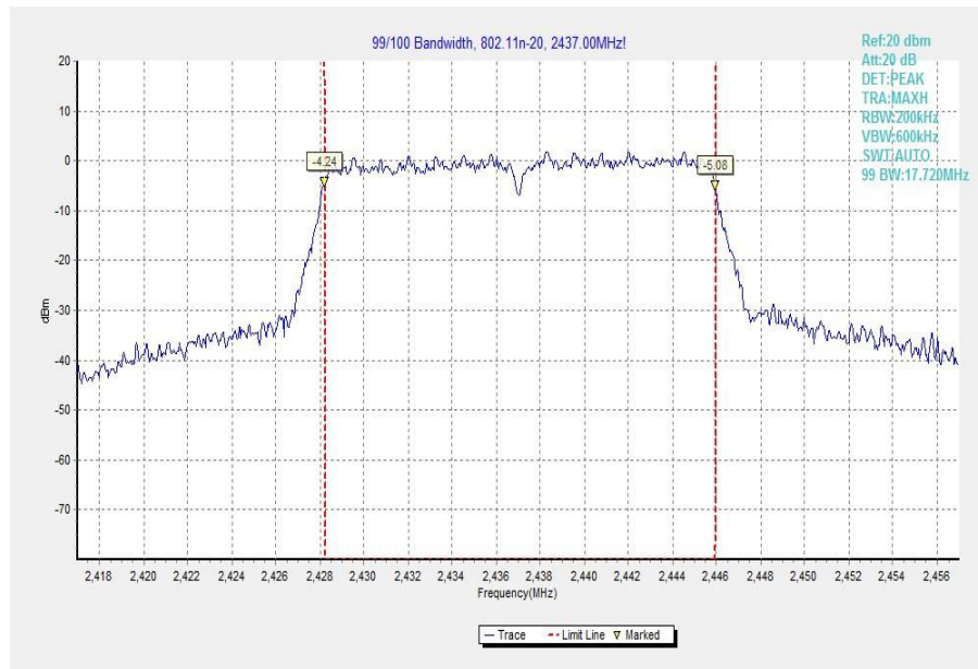
Fig.144 Occupied Bandwidth (802.11n-20MHz, Ch 6)
