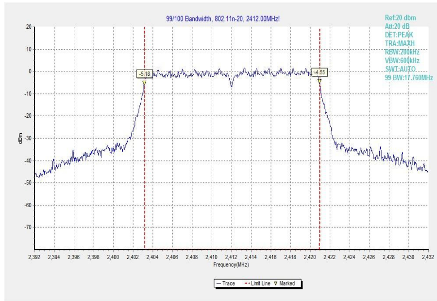
Fig.143 Occupied Bandwidth (802.11n-20MHz, Ch 1)
