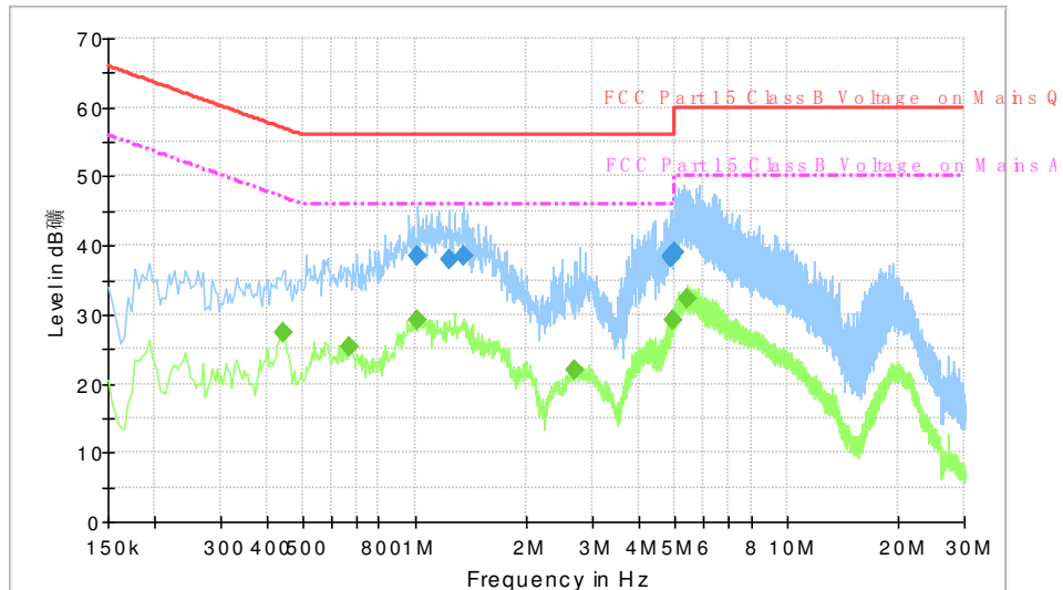
Fig.146 AC Powerline Conducted Emission (Traffic, AE1)
