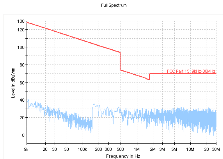
Fig.122 Radiated Spurious Emission (802.11g, Ch6, 9kHz-30MHz)
