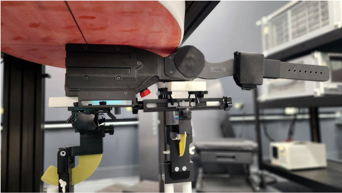
Figure E SAR Test Setup – Body – Bottom 0mm
