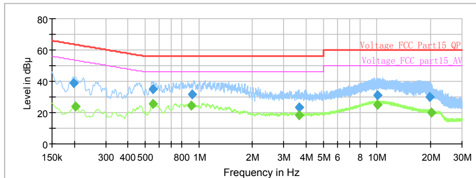
WIFI 2.4G_L_0.15-30Mhz
