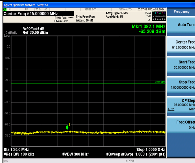
Band25_3MHz_QPSK_26365_1RB#0_30~1000_30~1000
