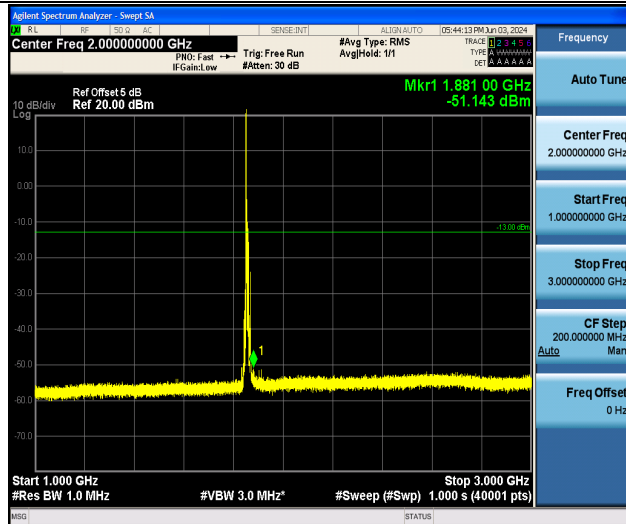
Band25_10MHz_QPSK_26090_1RB#0_1000~3000_1000~3000
