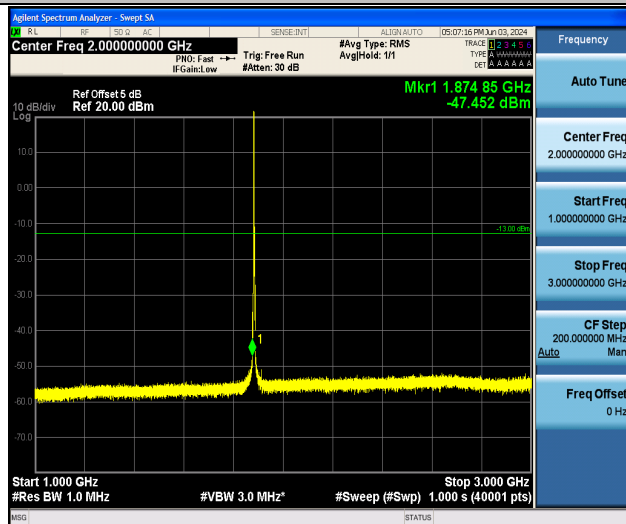
Band25_3MHz_QPSK_26365_1RB#0_1000~3000_1000~3000
