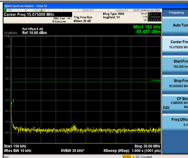
Band25_1.4MHz_16QAM_26683_1RB#0_0.15~30_0.15~30
