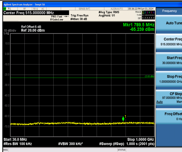
Band25_5MHz_16QAM_26665_1RB#0_30~1000_30~1000
