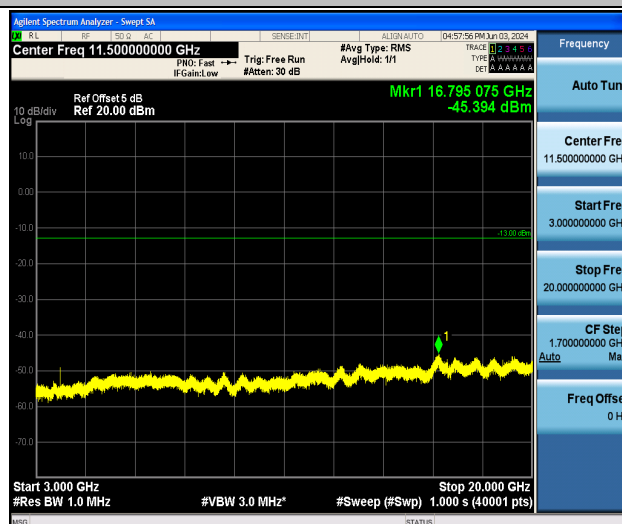
Band25_1.4MHz_16QAM_26683_1RB#0_3000~20000_3000~20000
