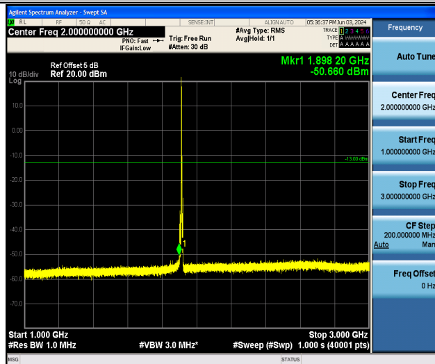
Band25_5MHz_16QAM_26665_1RB#0_1000~3000_1000~3000
