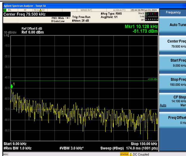
Band25_10MHz_16QAM_26090_1RB#0_0.009~0.15_0.009~0.15
