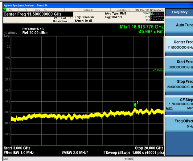
Band25_10MHz_QPSK_26090_1RB#0_3000~20000_3000~20000
