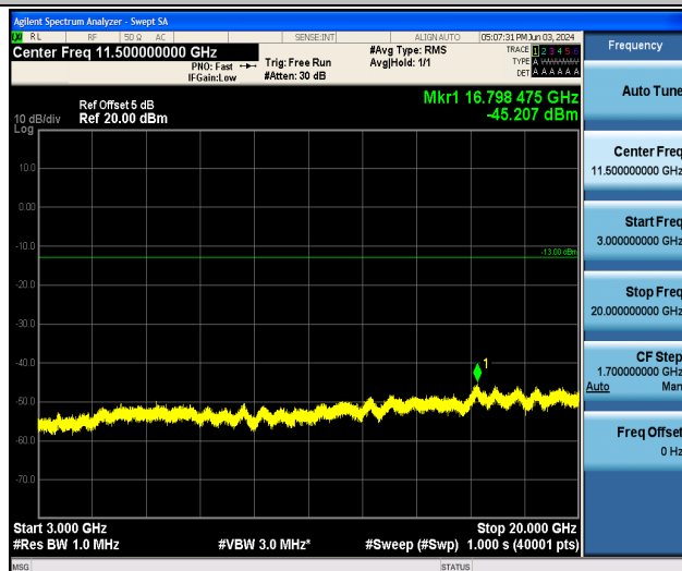
Band25_3MHz_QPSK_26365_1RB#0_3000~20000_3000~20000
