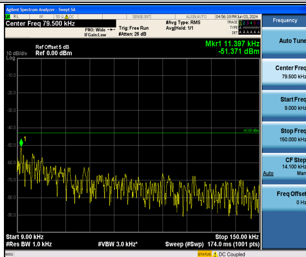
Band25_1.4MHz_QPSK_26683_1RB#0_0.009~0.15_0.009~0.15
