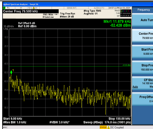
Band25_1.4MHz_16QAM_26683_1RB#0_0.009~0.15_0.009~0.15
