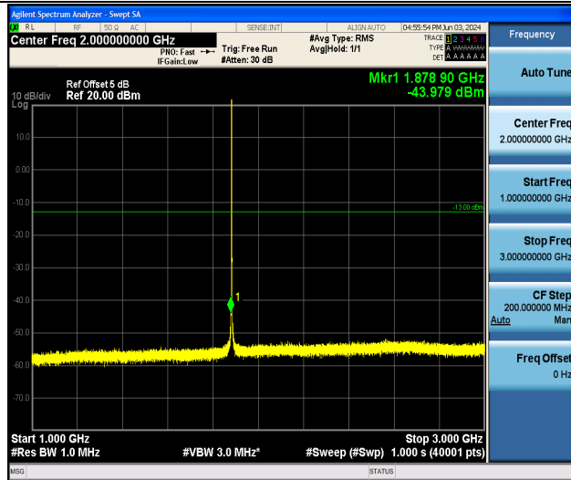
Band25_1.4MHz_16QAM_26365_1RB#0_1000~3000_1000~3000
