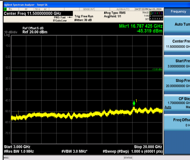
Band25_1.4MHz_QPSK_26683_1RB#0_3000~20000_3000~20000
