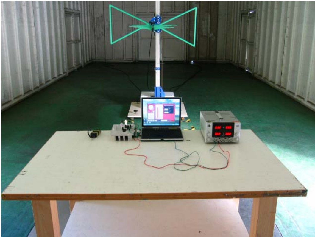
Back View of Radiated Test (Green Antenna)
