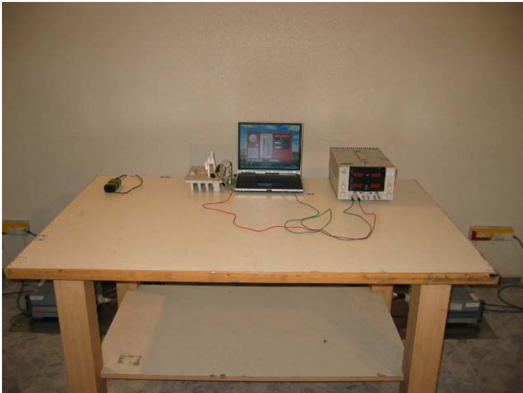
Back View of Conducted Test (White Antenna)
