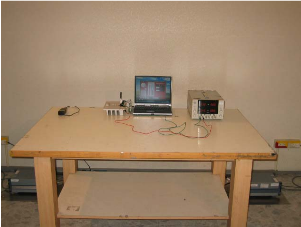
Back View of Conducted Test (Green Antenna)
