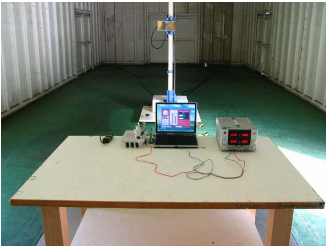
Front View of Radiated Test (White Antenna) (Horn)
