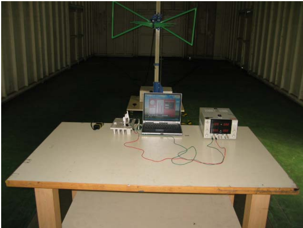
Back View of Radiated Test (White Antenna)
